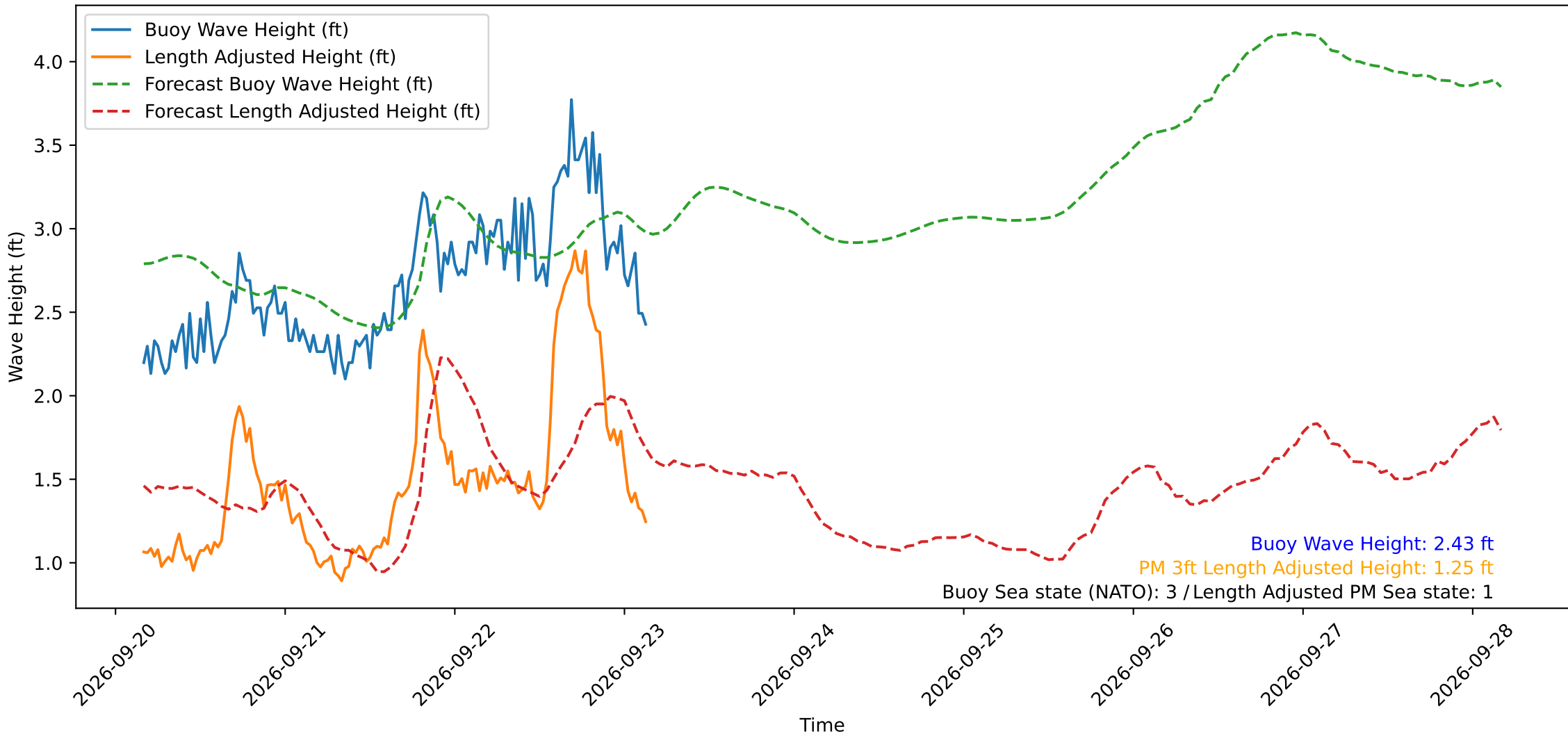
Wave Heights over Time for Oceanside Harbor at 2026-09-23 03:50:30
