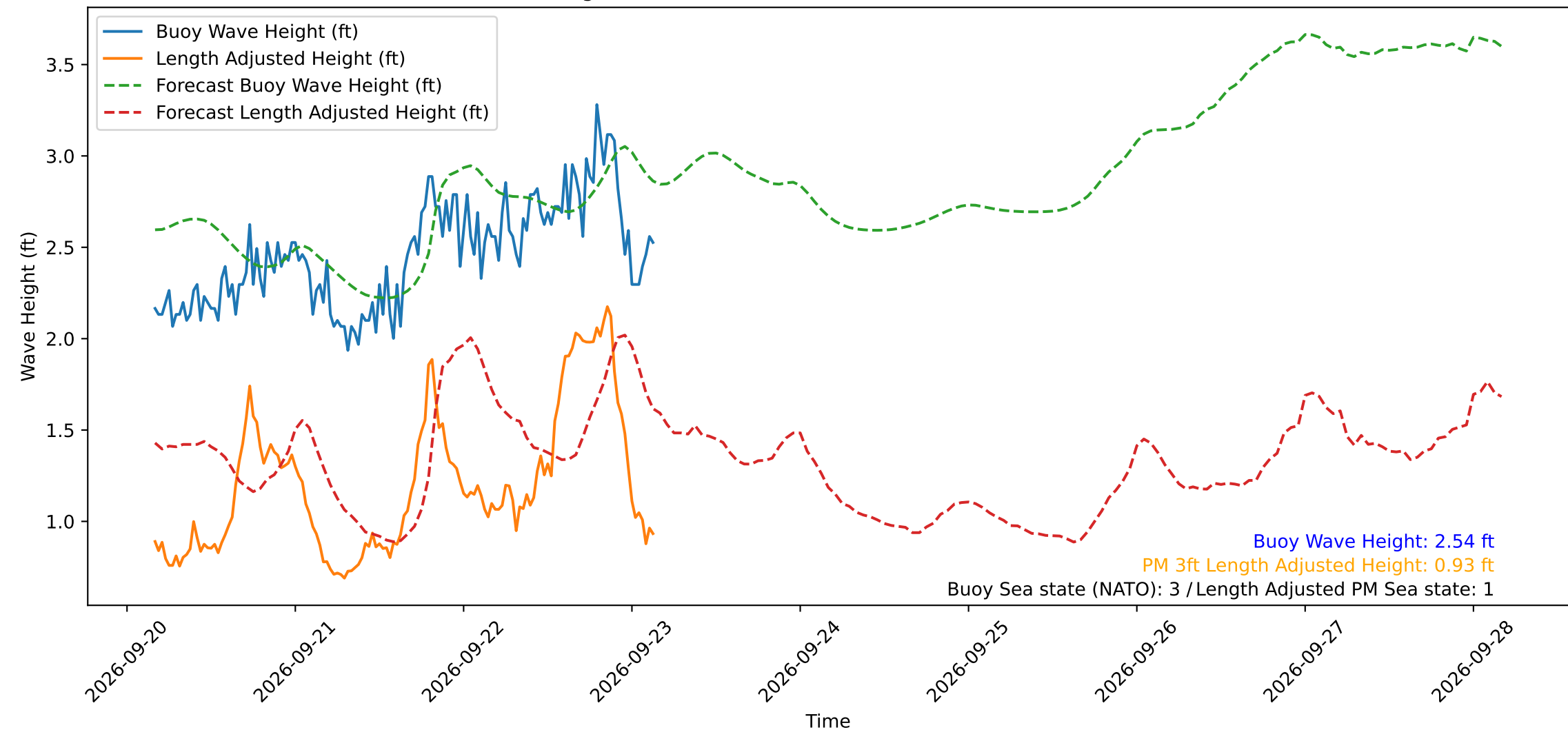
Wave Heights over Time for Red Beach at 2026-09-23 03:50:51
