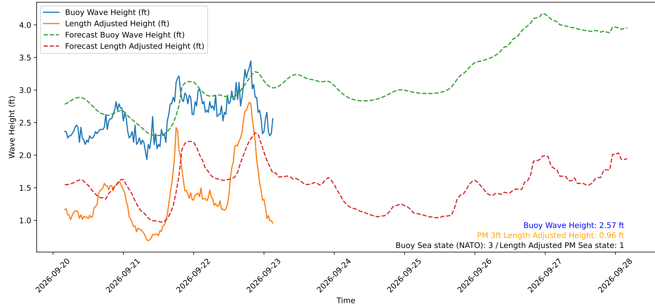
Wave Heights over Time for Green Beach at 2026-09-23 03:51:15
