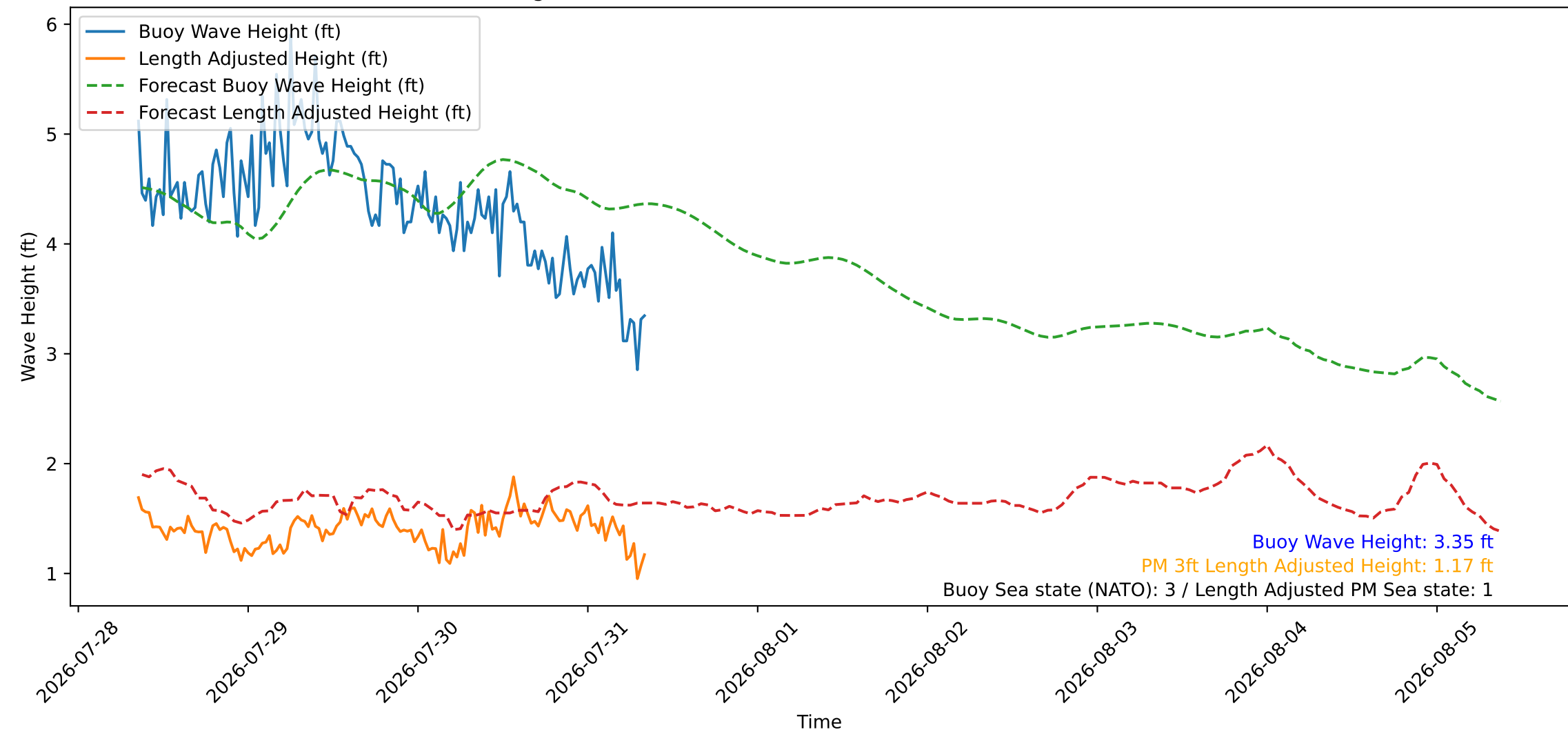
Wave Heights over Time for Oceanside Harbor at 2026-07-31 08:30:26
