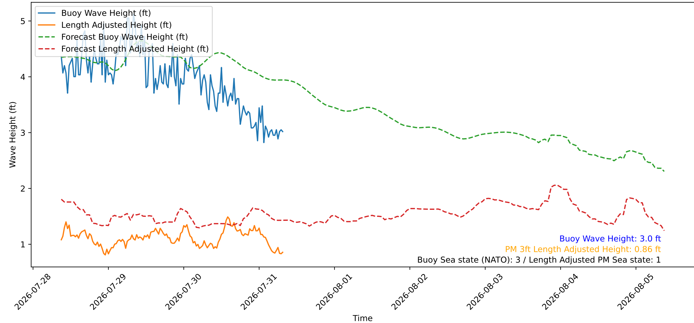
Wave Heights over Time for Red Beach at 2026-07-31 08:30:46
