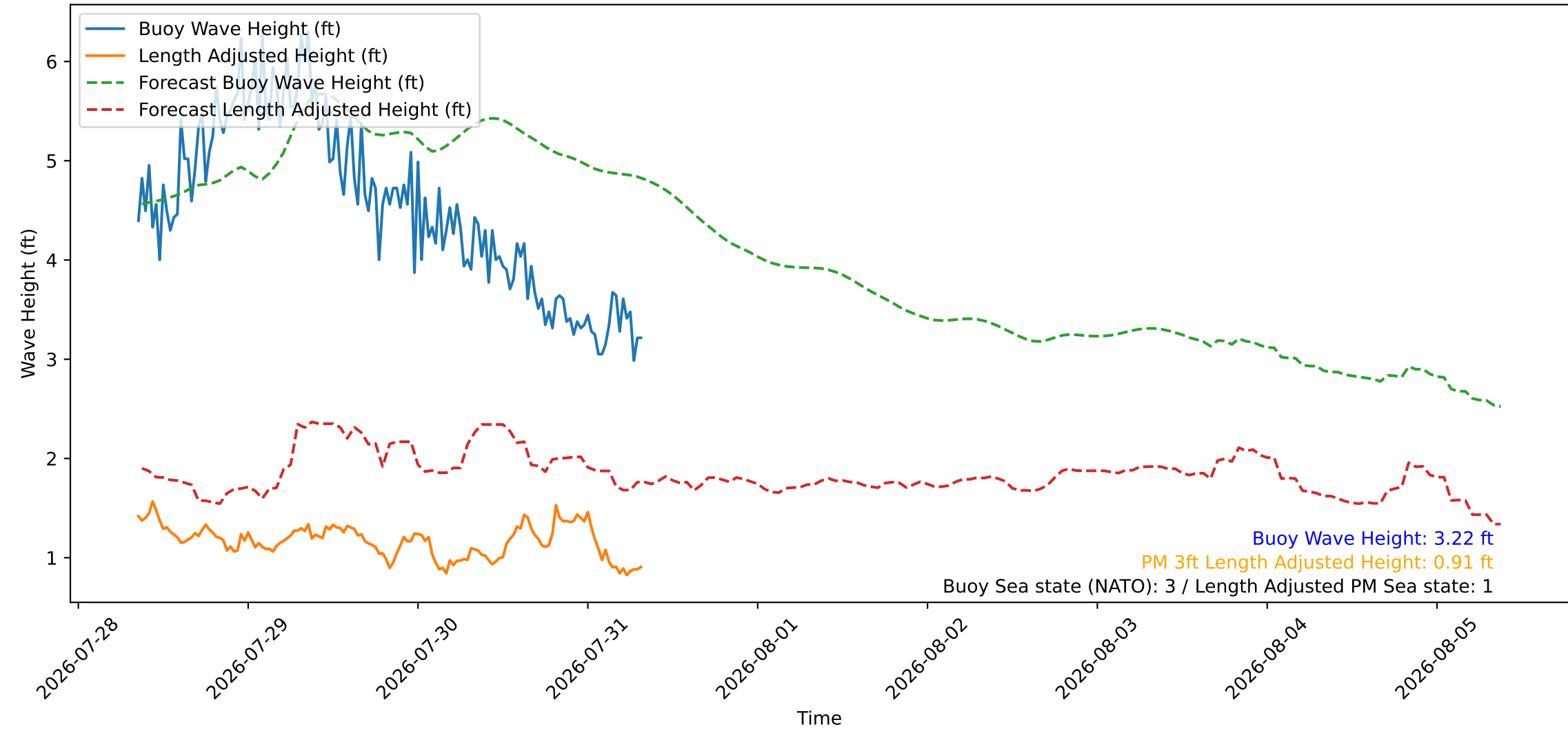
Wave Heights over Time for Green Beach at 2026-07-31 08:31:09
