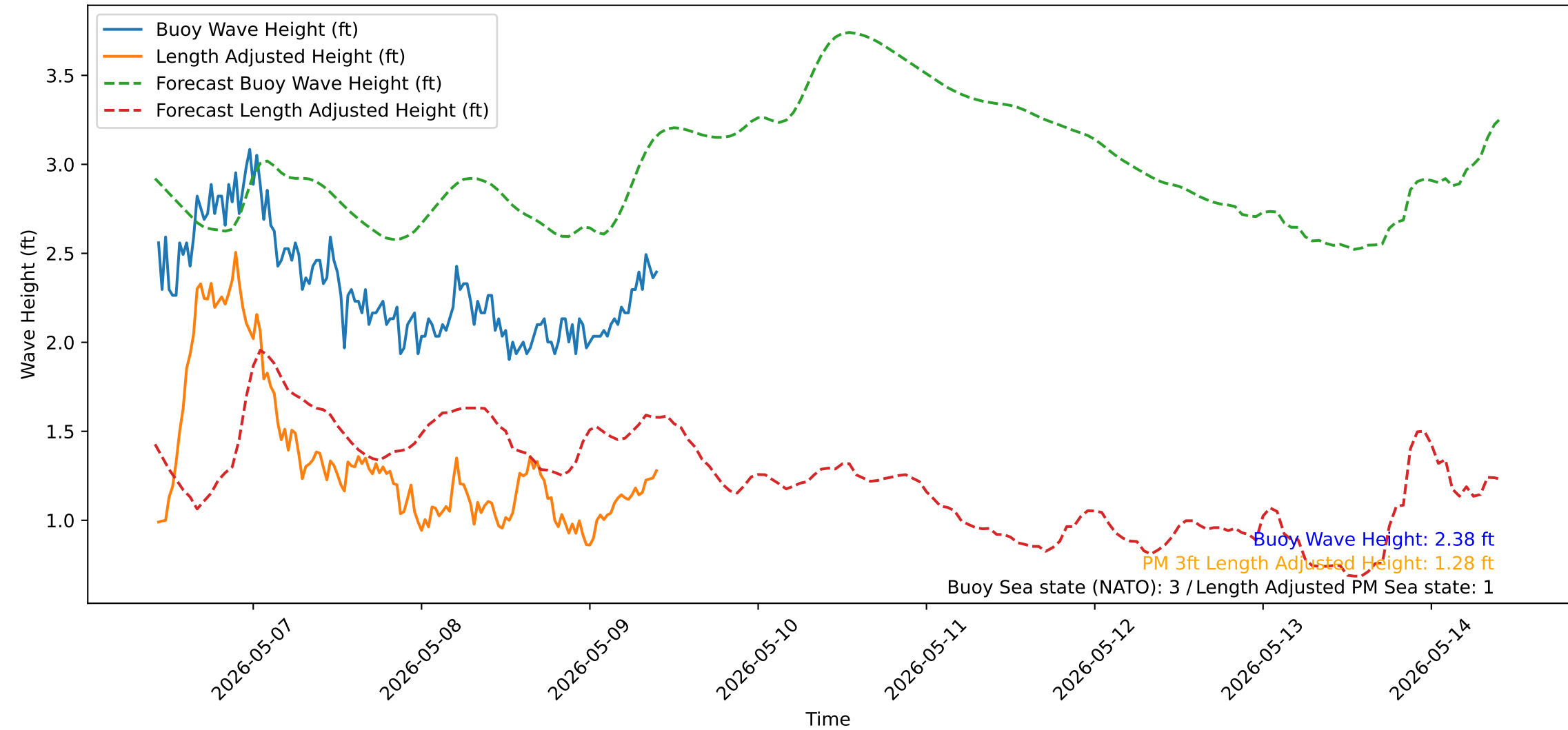
Wave Heights over Time for Red Beach at 2026-05-09 10:10:51
