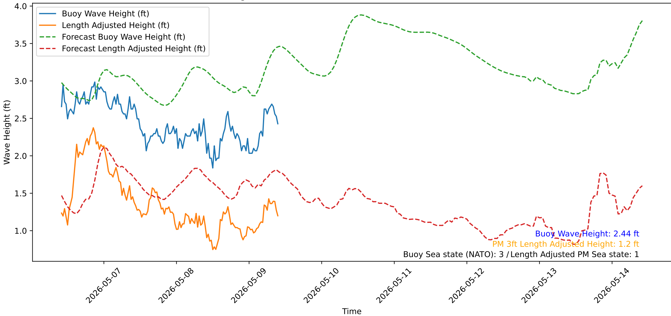
Wave Heights over Time for Green Beach at 2026-05-09 10:11:13
