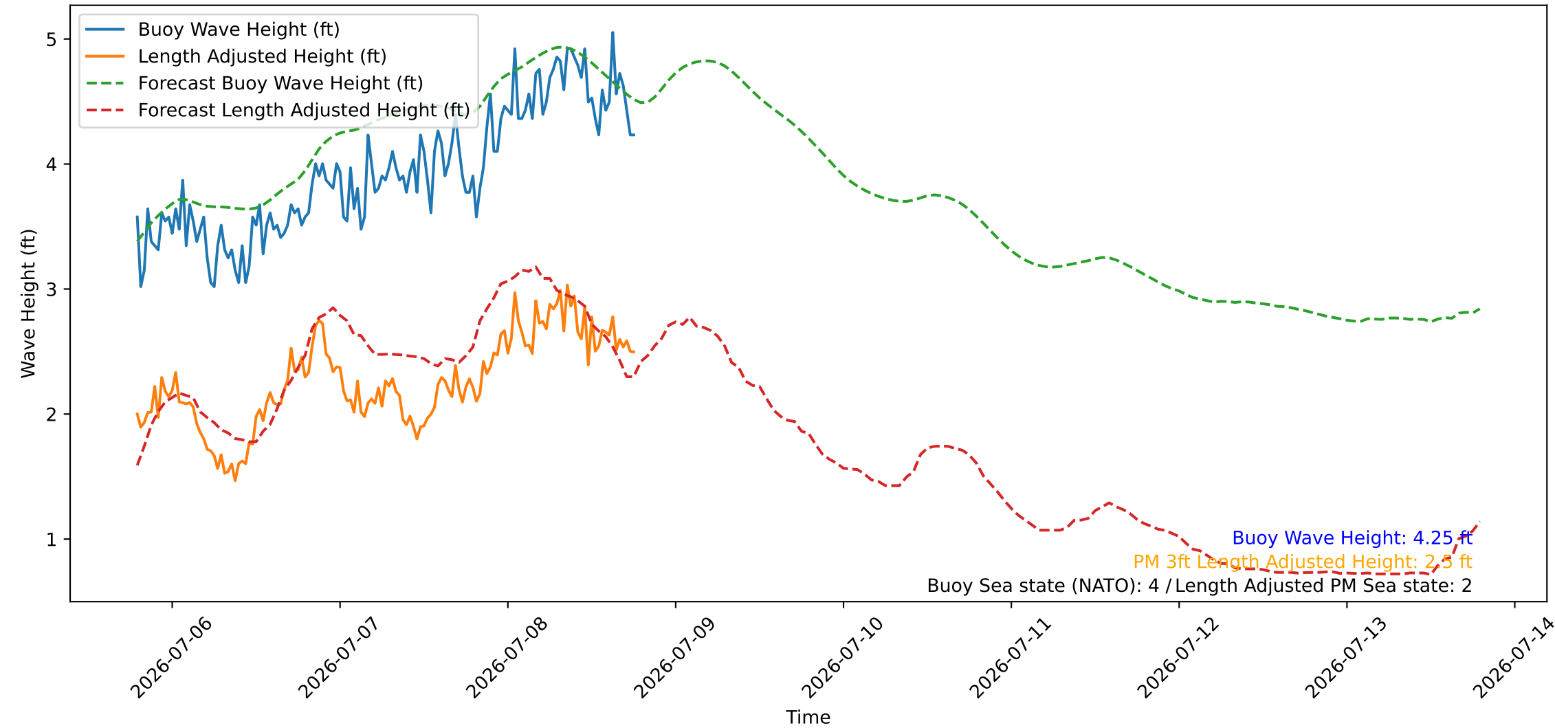
Wave Heights over Time for Oceanside Harbor at 2026-07-08 18:50:26
