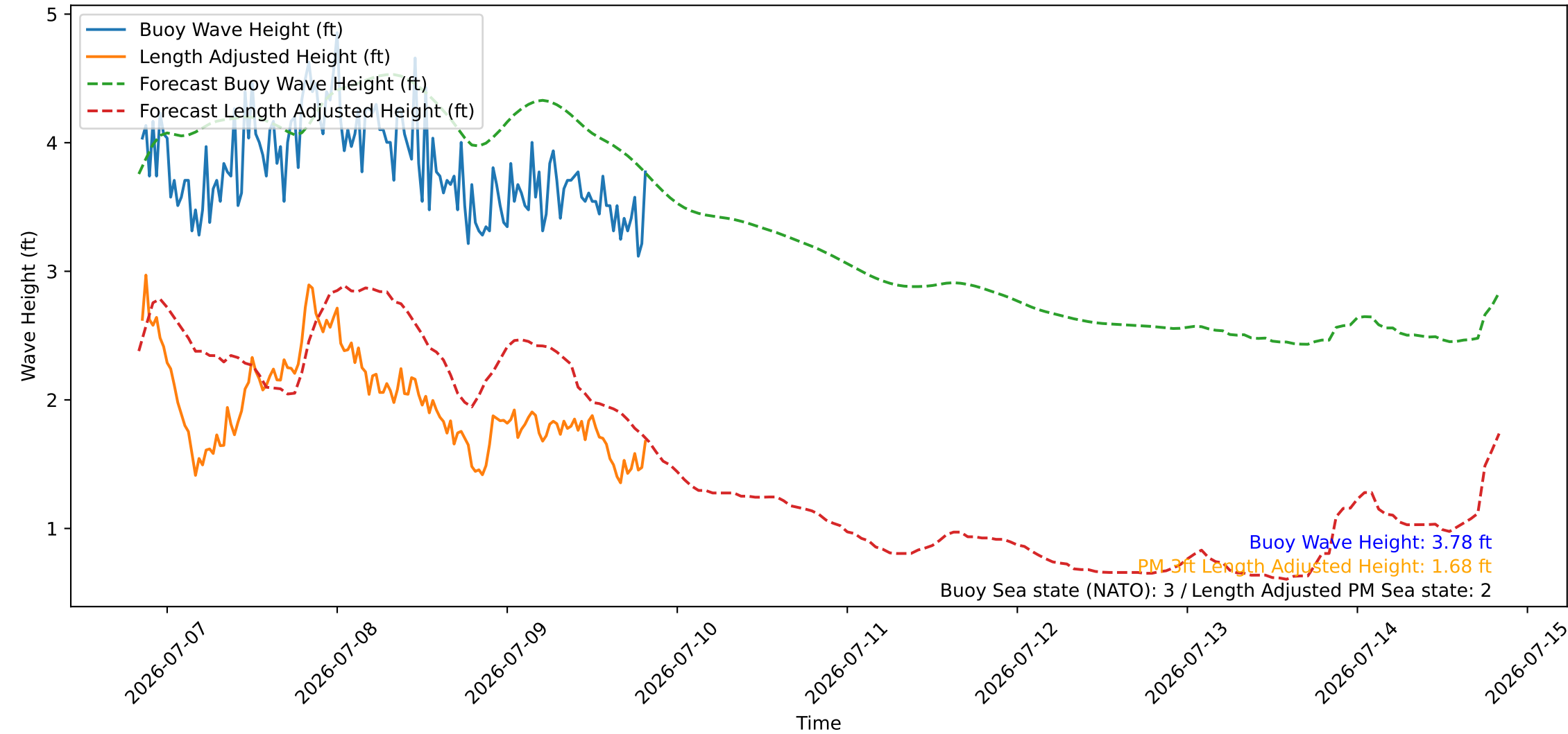
Wave Heights over Time for Red Beach at 2026-07-09 20:10:46
