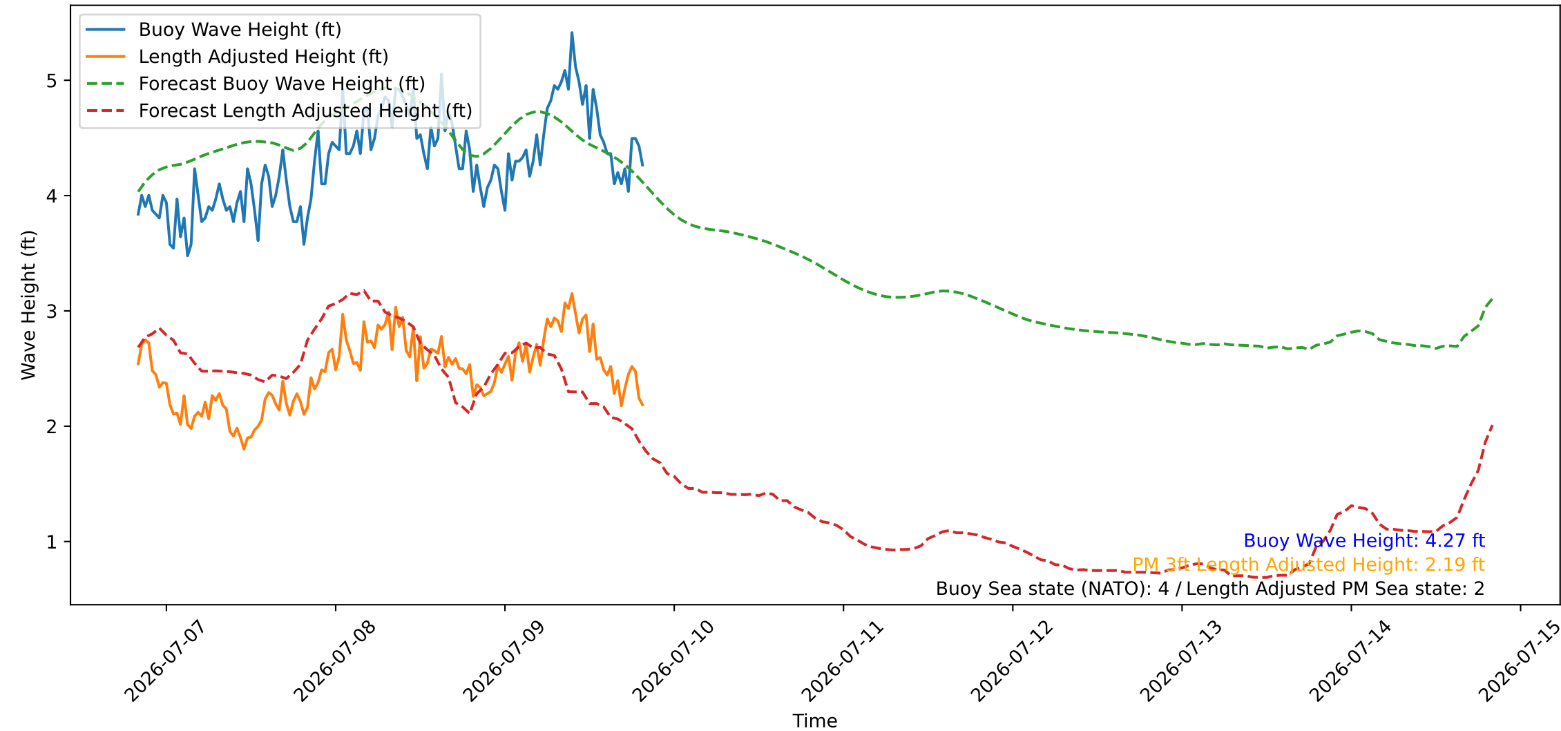
Wave Heights over Time for Oceanside Harbor at 2026-07-09 20:10:27
