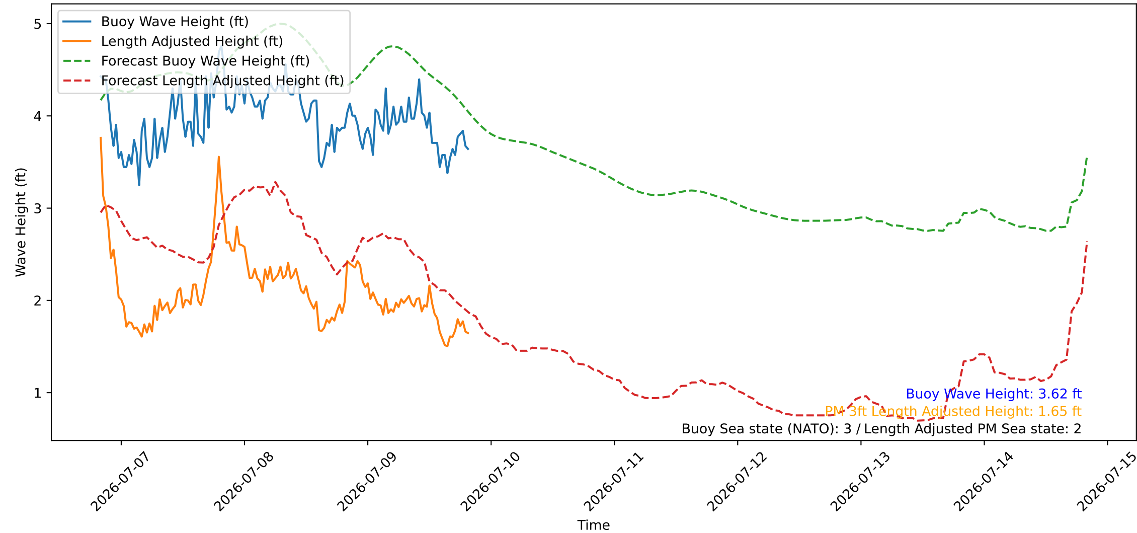
Wave Heights over Time for Green Beach at 2026-07-09 20:11:09
