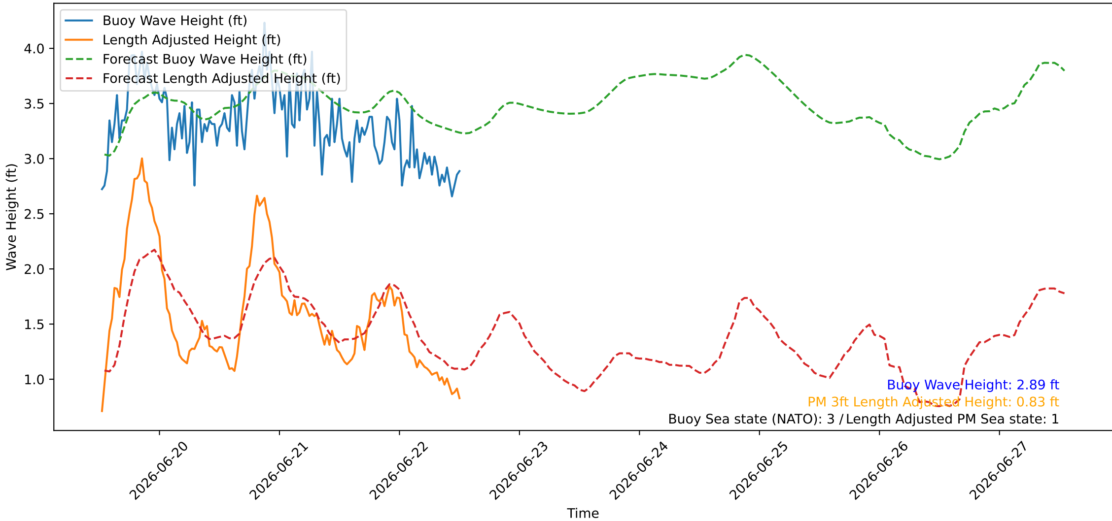
Wave Heights over Time for Green Beach at 2026-06-22 12:41:08
