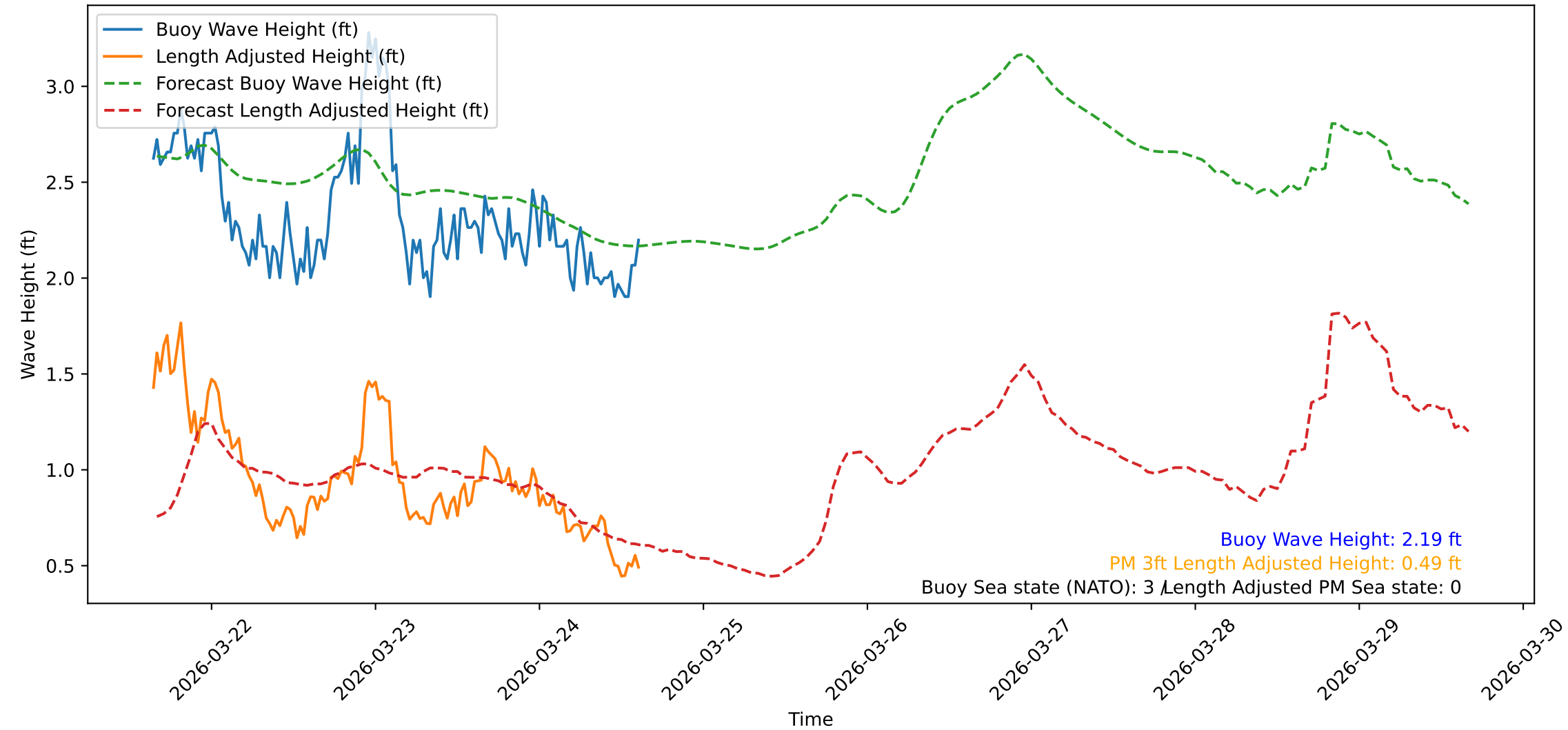
Wave Heights over Time for Green Beach at 2026-03-24 15:31:08
