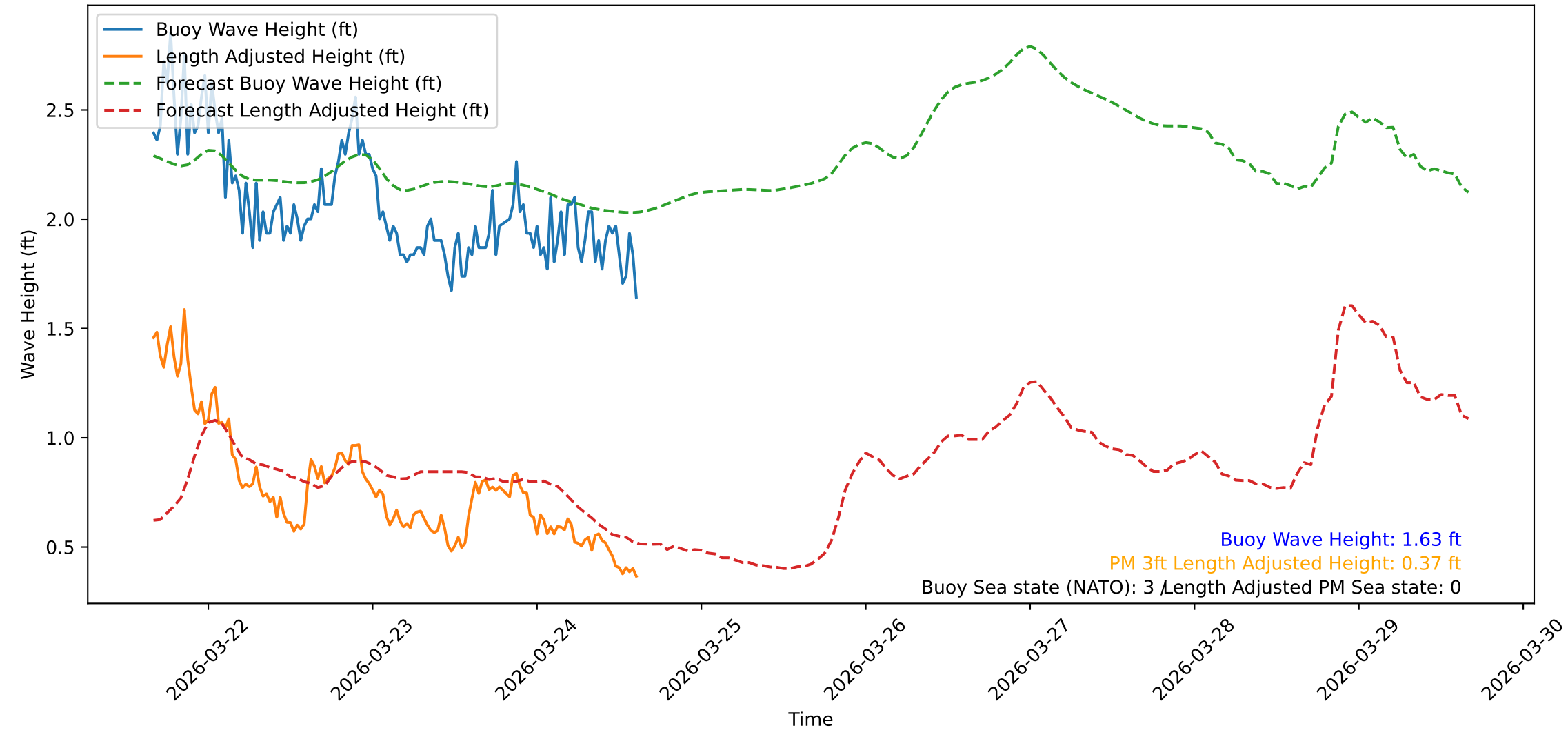
Wave Heights over Time for Red Beach at 2026-03-24 15:30:47
