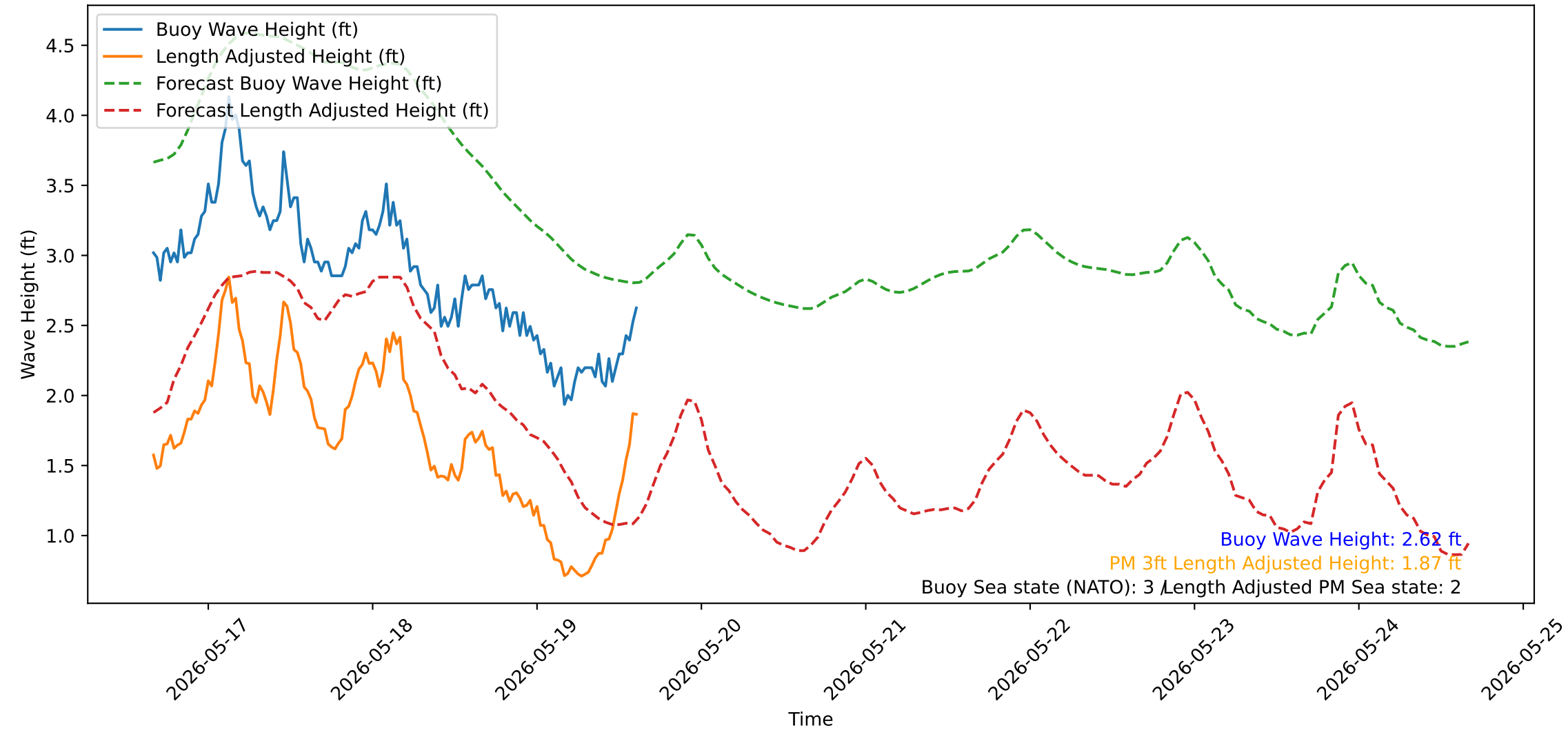
Wave Heights over Time for Red Beach at 2026-05-19 15:50:52
