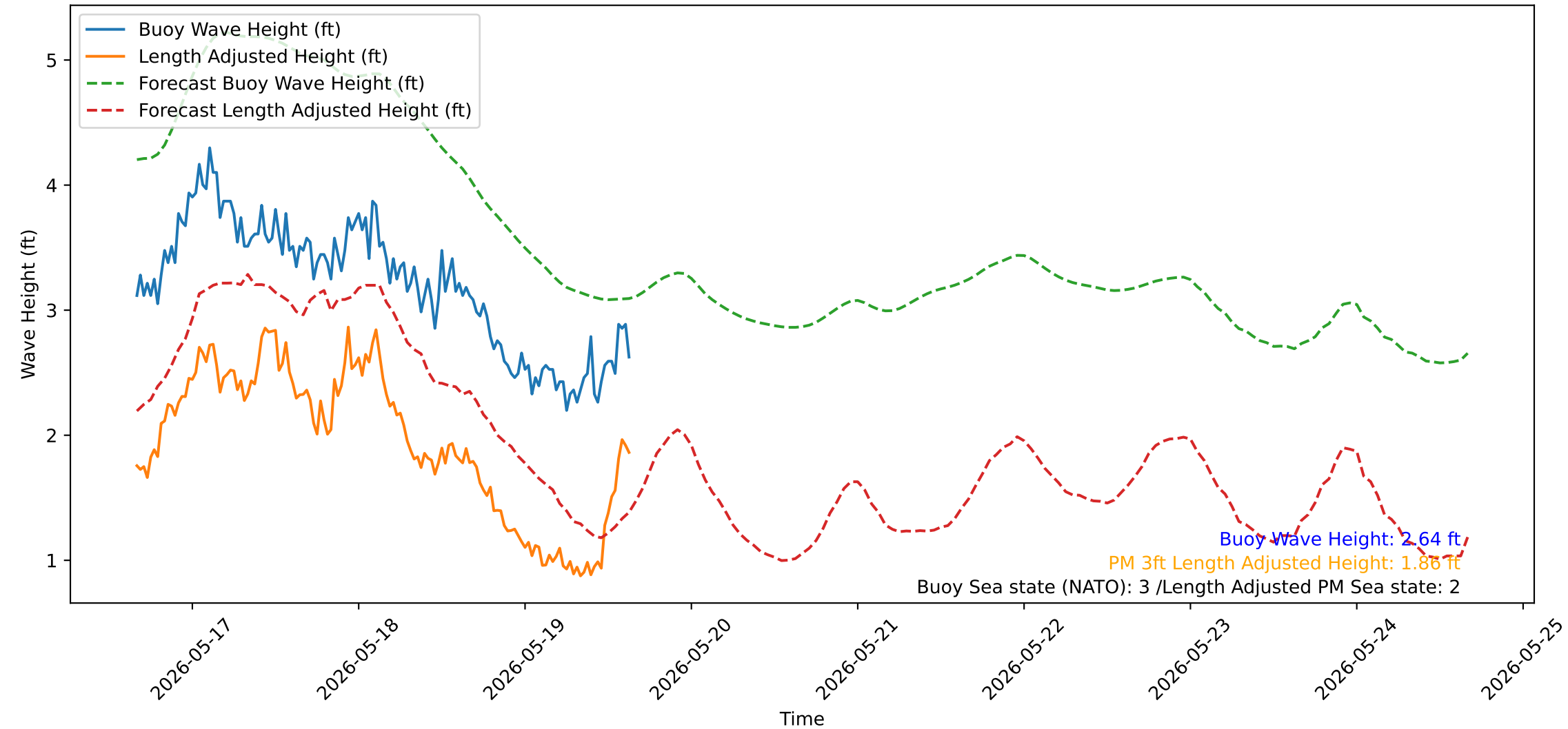
Wave Heights over Time for Oceanside Harbor at 2026-05-19 15:50:31
