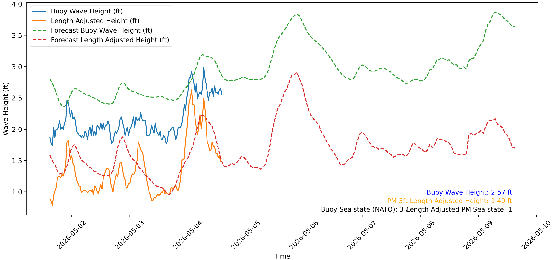
Wave Heights over Time for Green Beach at 2026-05-04 14:51:14
