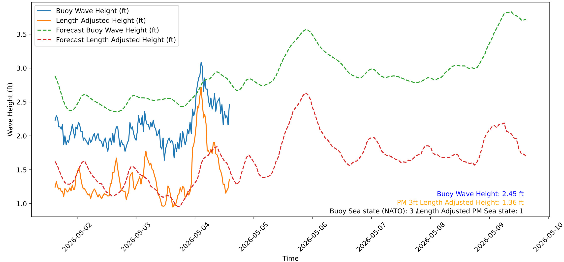
Wave Heights over Time for Oceanside Harbor at 2026-05-04 14:50:31
