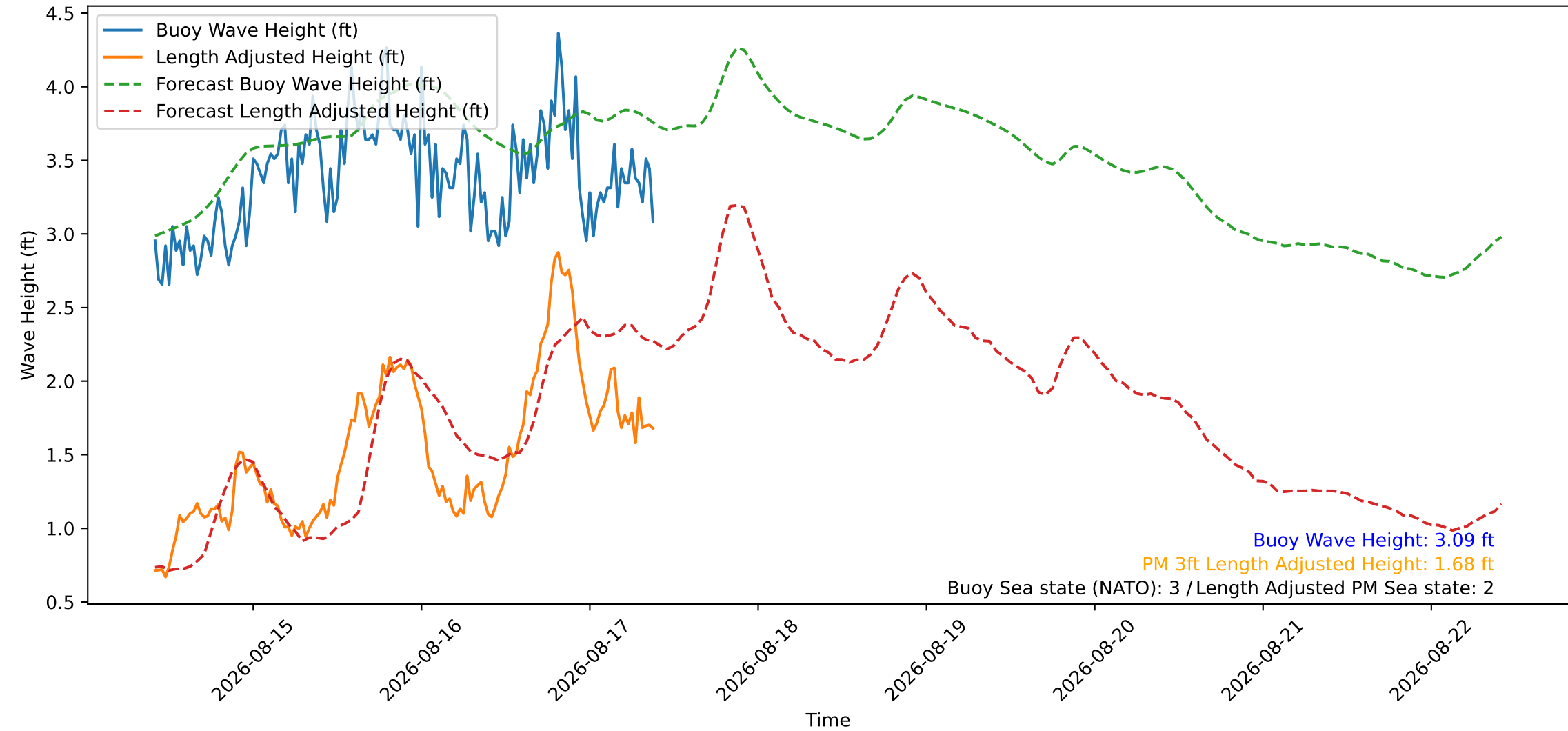
Wave Heights over Time for Green Beach at 2026-08-17 09:51:12
