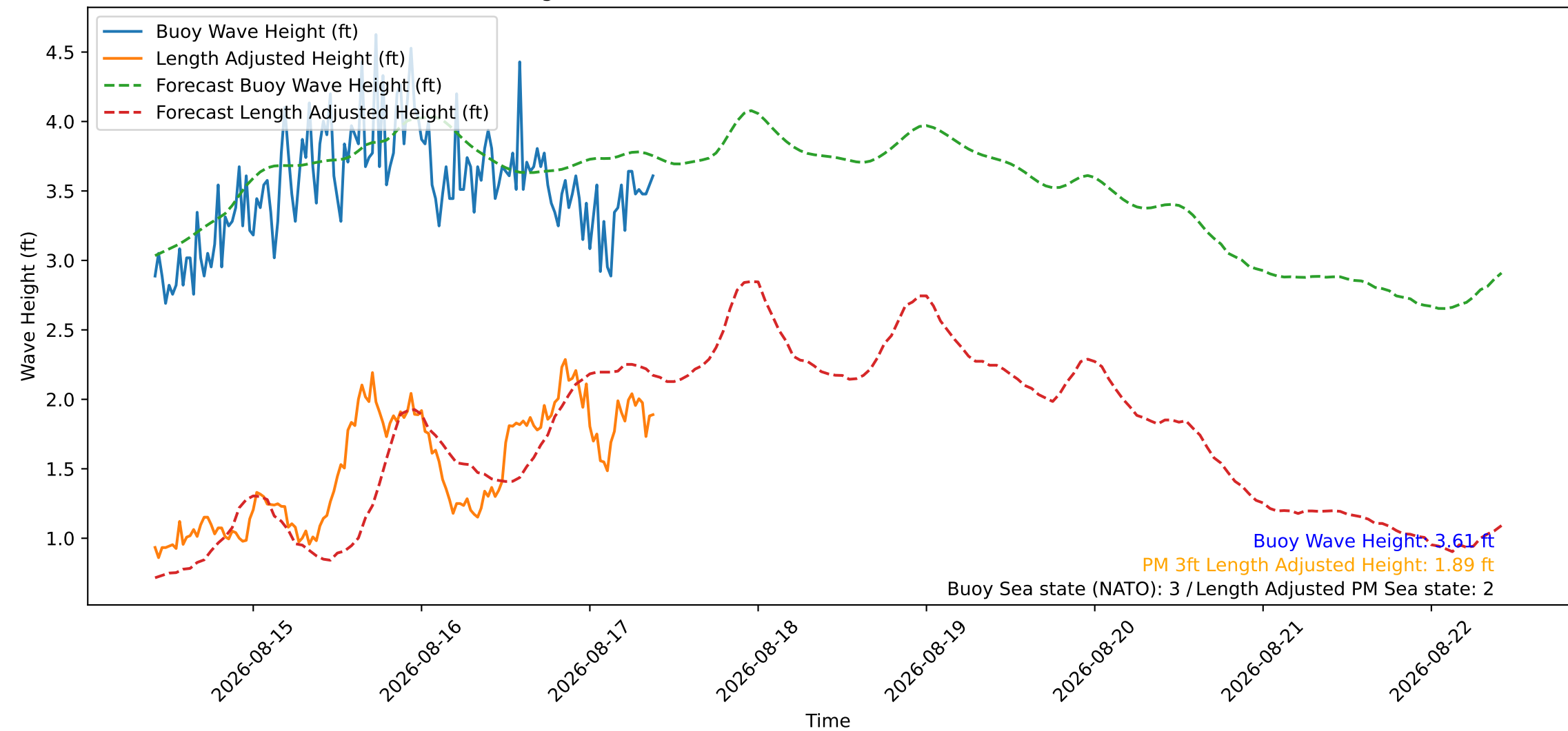
Wave Heights over Time for Oceanside Harbor at 2026-08-17 09:50:26
