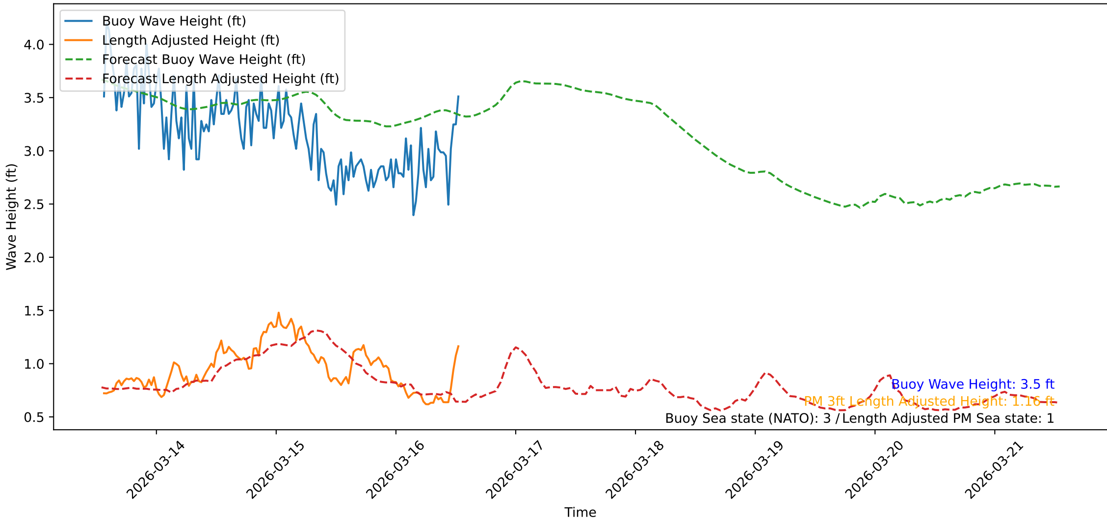
Wave Heights over Time for Oceanside Harbor at 2026-03-16 13:20:47
