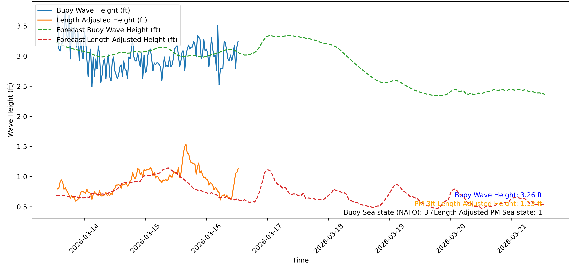
Wave Heights over Time for Red Beach at 2026-03-16 13:21:11
