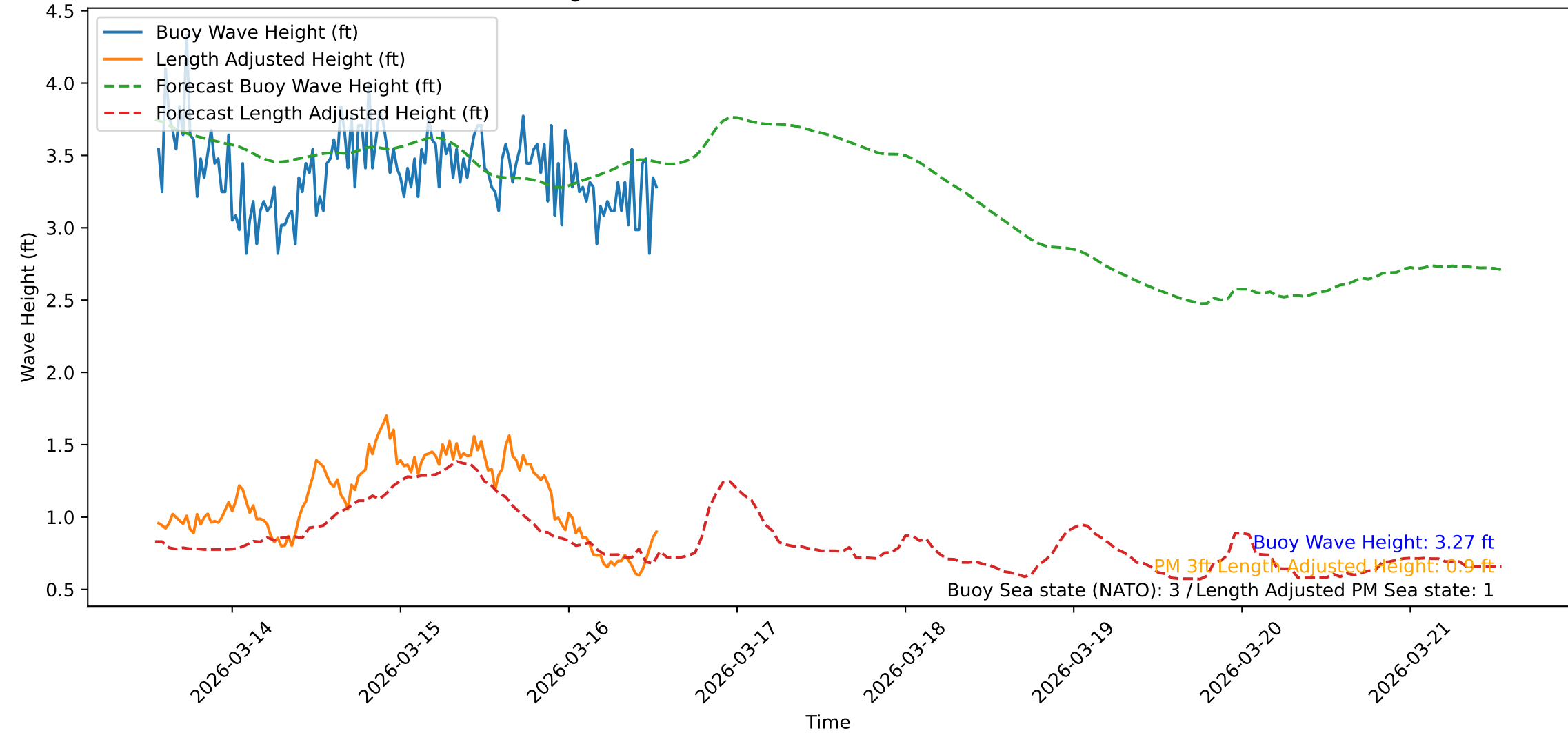
Wave Heights over Time for Green Beach at 2026-03-16 13:21:44
