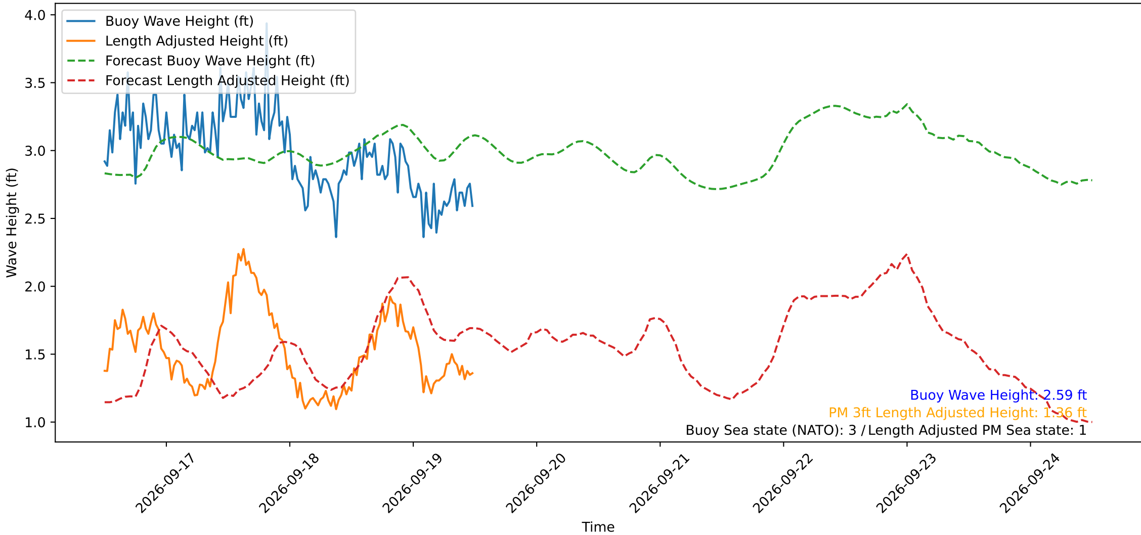
Wave Heights over Time for Oceanside Harbor at 2026-09-19 12:10:29
