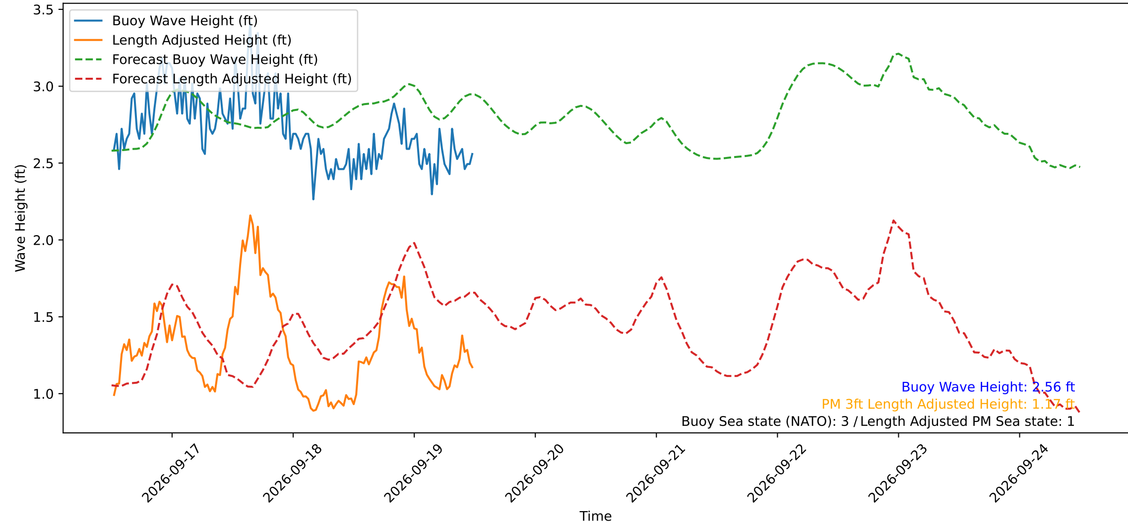
Wave Heights over Time for Red Beach at 2026-09-19 12:10:49
