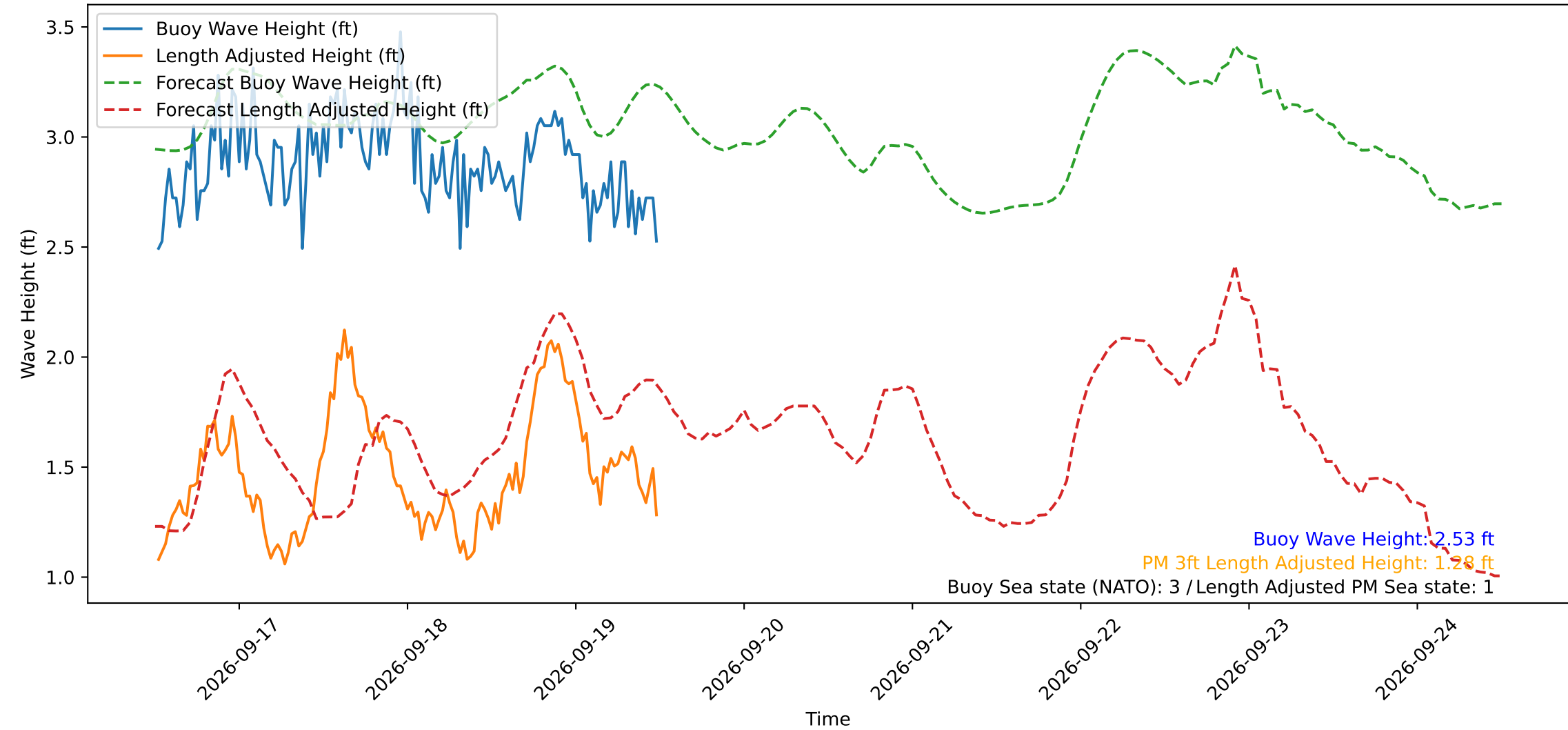
Wave Heights over Time for Green Beach at 2026-09-19 12:11:11
