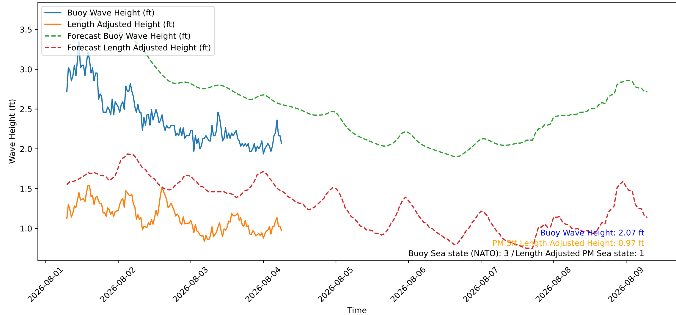
Wave Heights over Time for Red Beach at 2026-08-04 06:50:47
