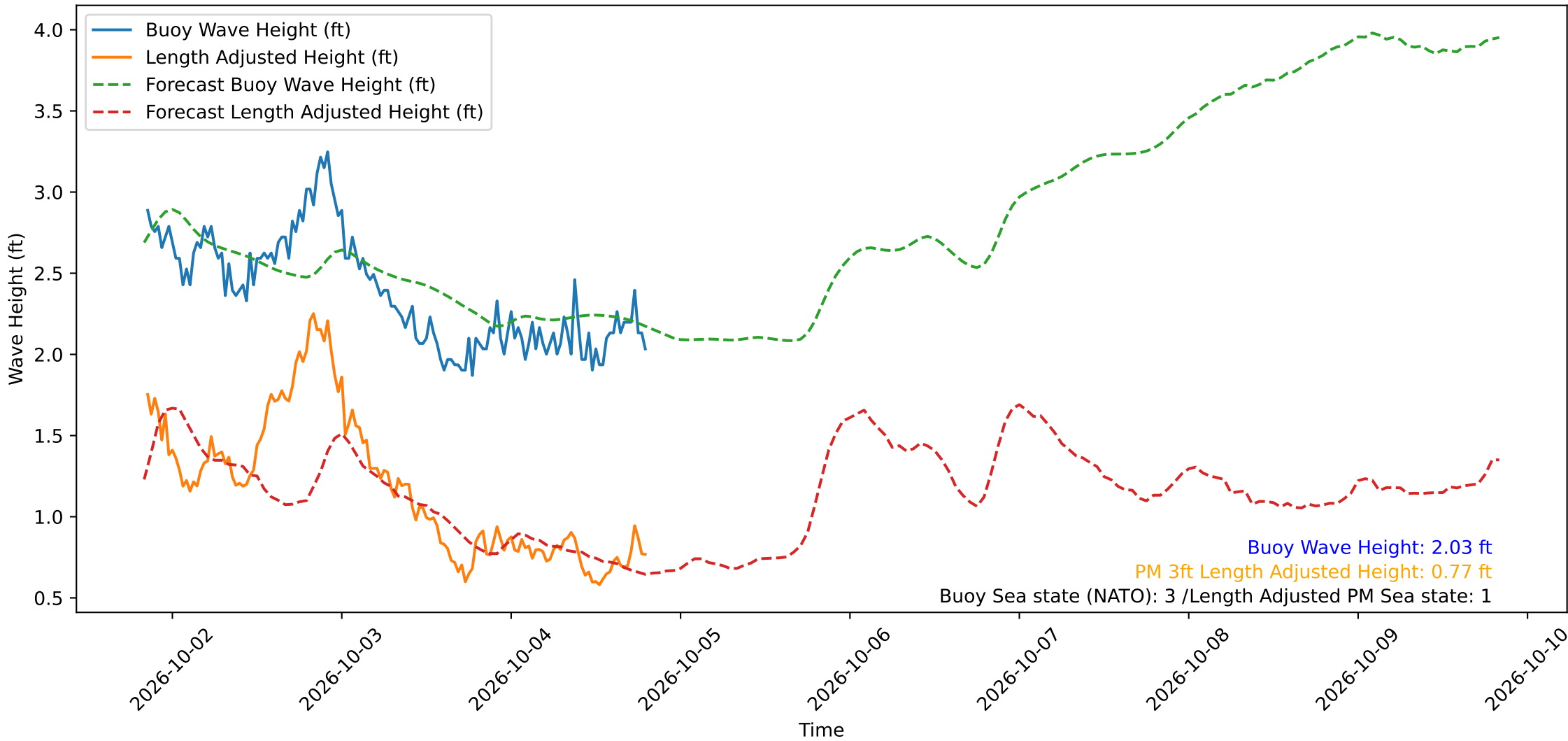
Wave Heights over Time for Red Beach at 2026-10-04 20:00:50
