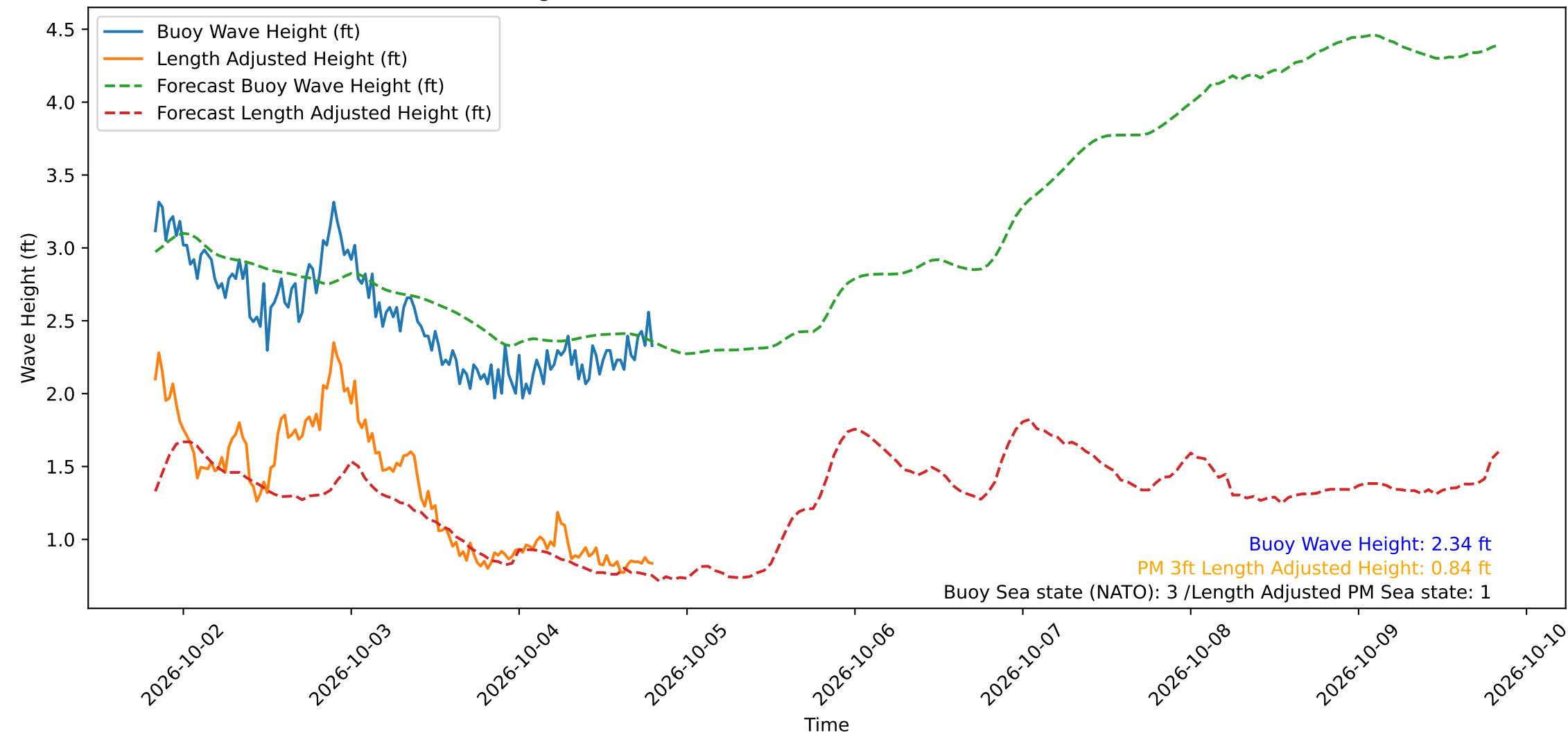
Wave Heights over Time for Oceanside Harbor at 2026-10-04 20:00:30
