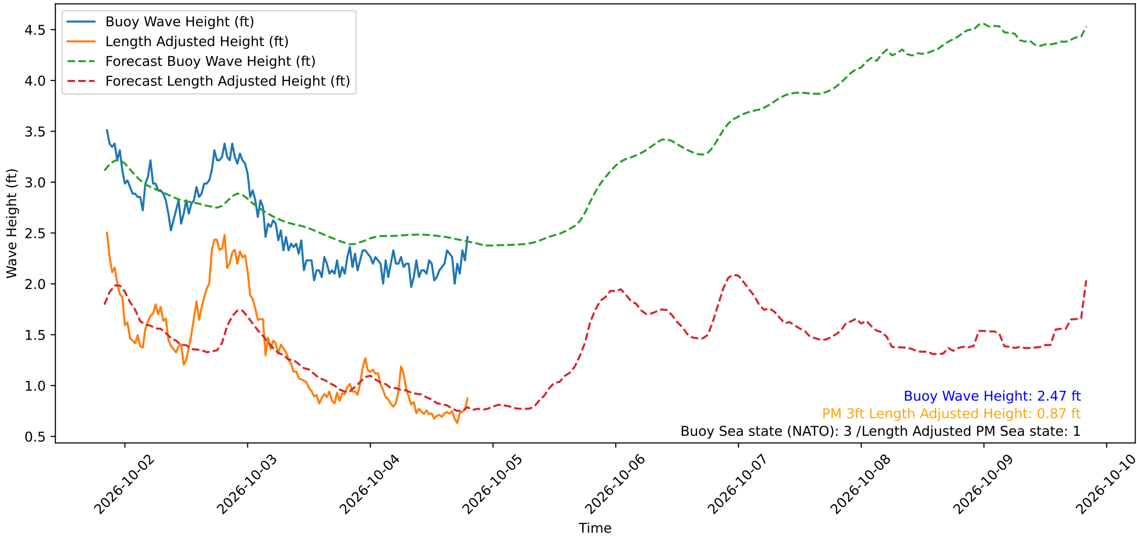
Wave Heights over Time for Green Beach at 2026-10-04 20:01:12
