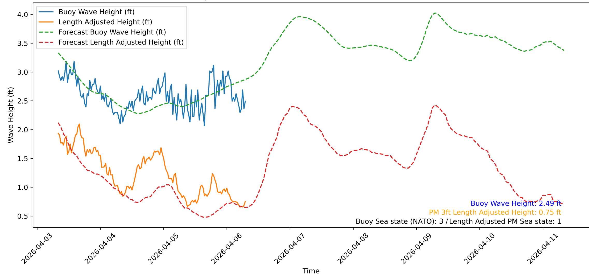
Wave Heights over Time for Oceanside Harbor at 2026-04-06 07:50:31
