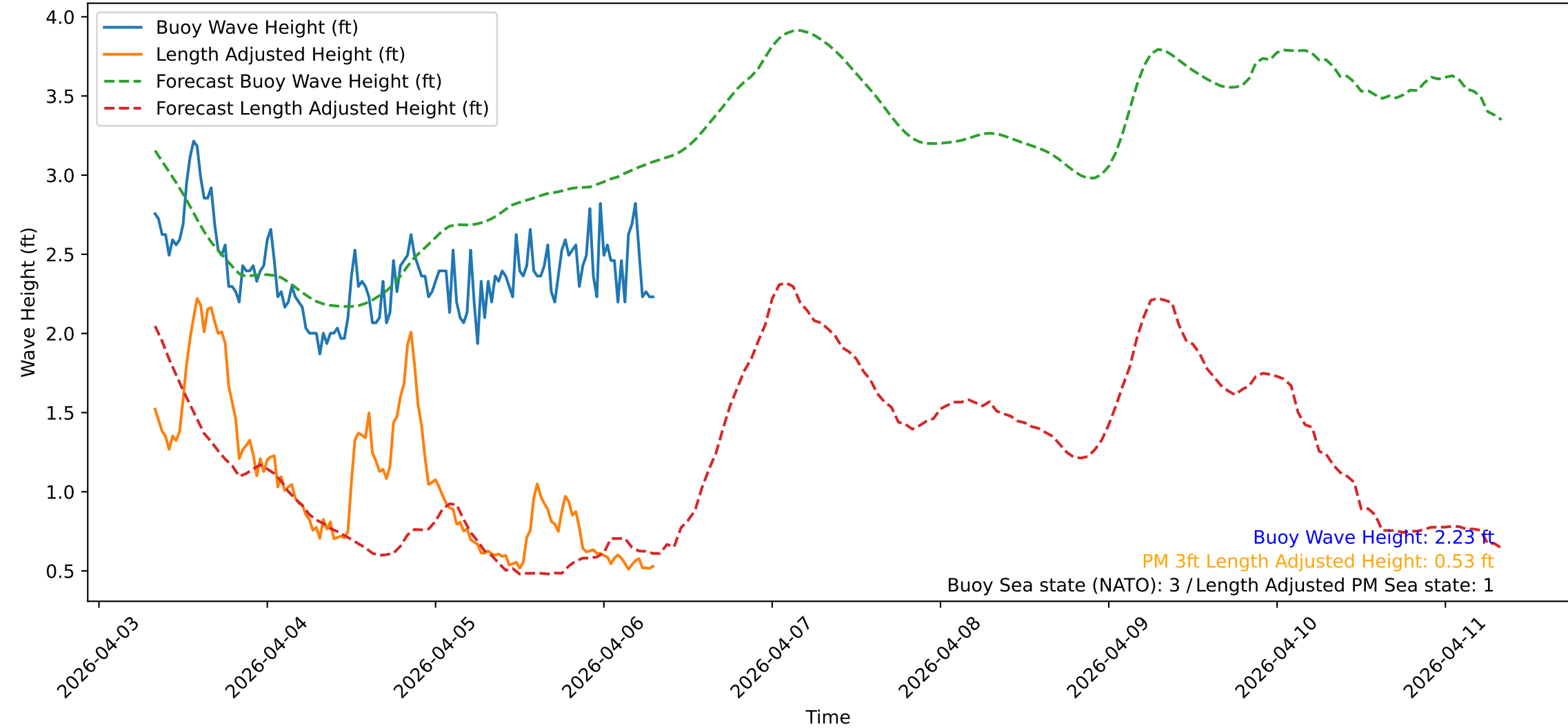
Wave Heights over Time for Red Beach at 2026-04-06 07:50:47
