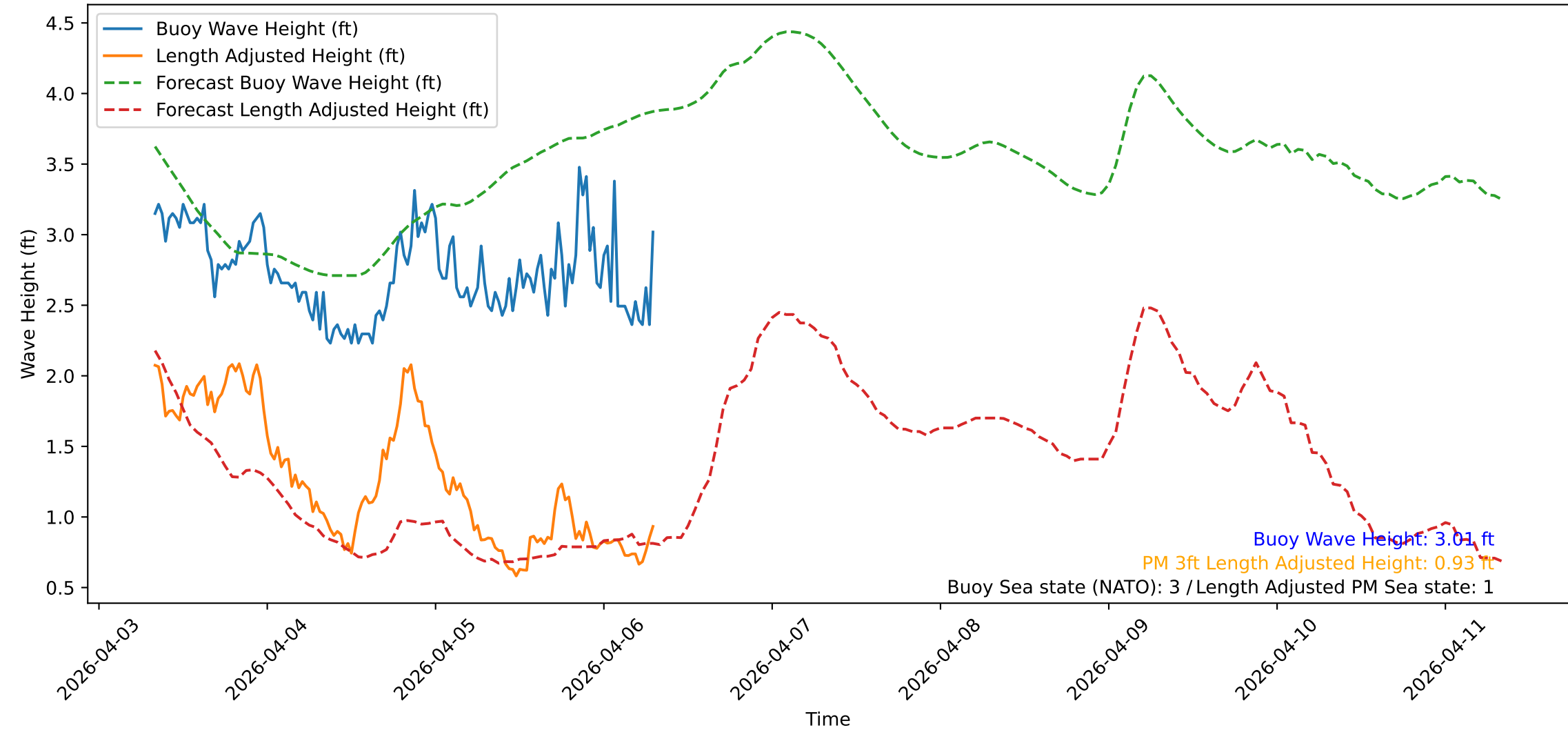
Wave Heights over Time for Green Beach at 2026-04-06 07:51:10
