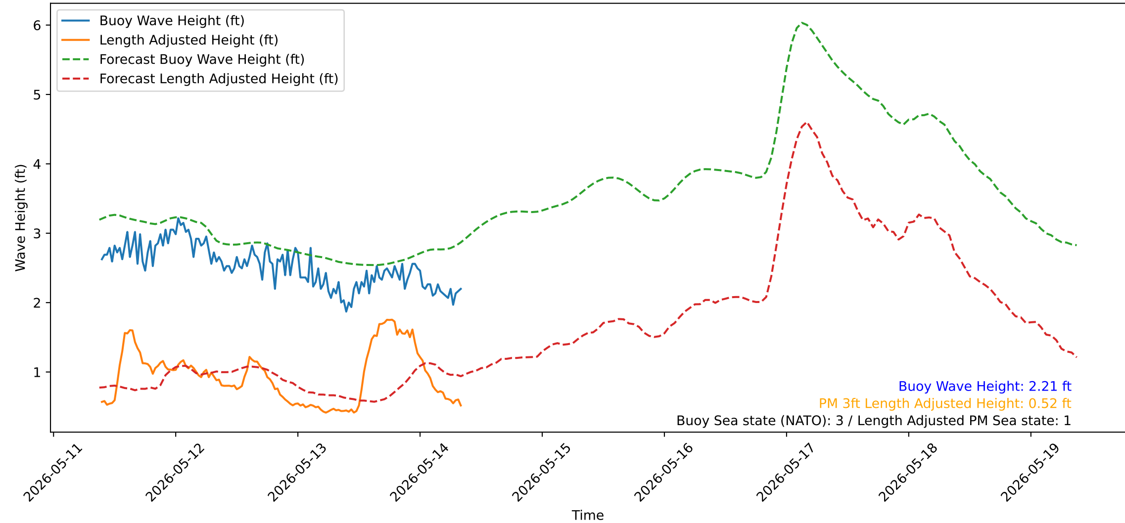
Wave Heights over Time for Red Beach at 2026-05-14 09:00:50
