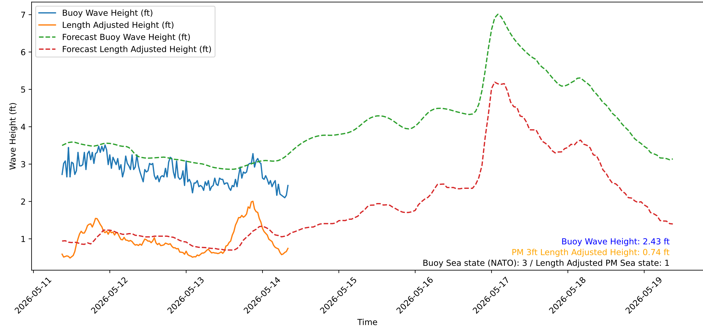
Wave Heights over Time for Green Beach at 2026-05-14 09:01:13
