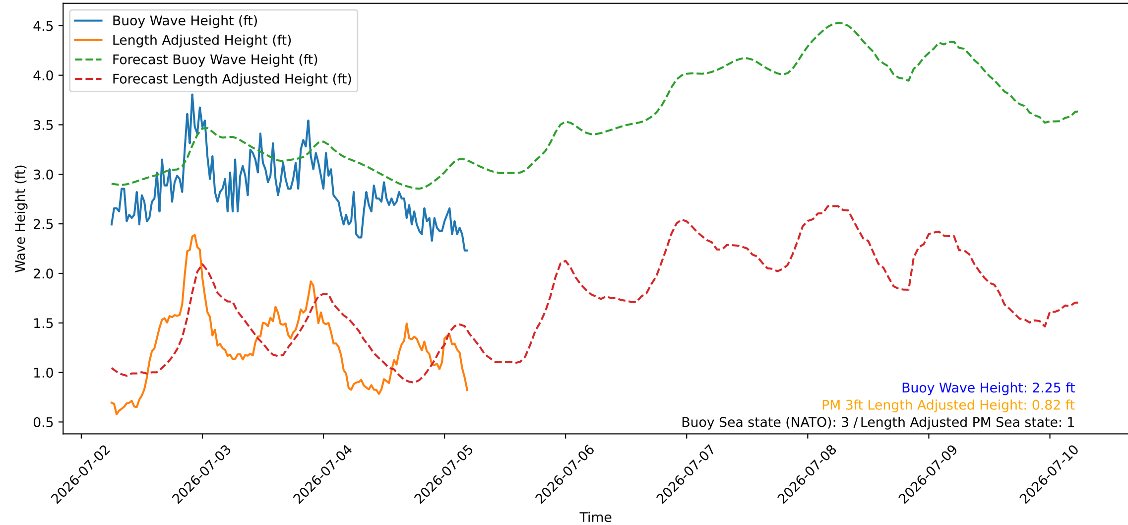
Wave Heights over Time for Red Beach at 2026-07-05 05:30:46
