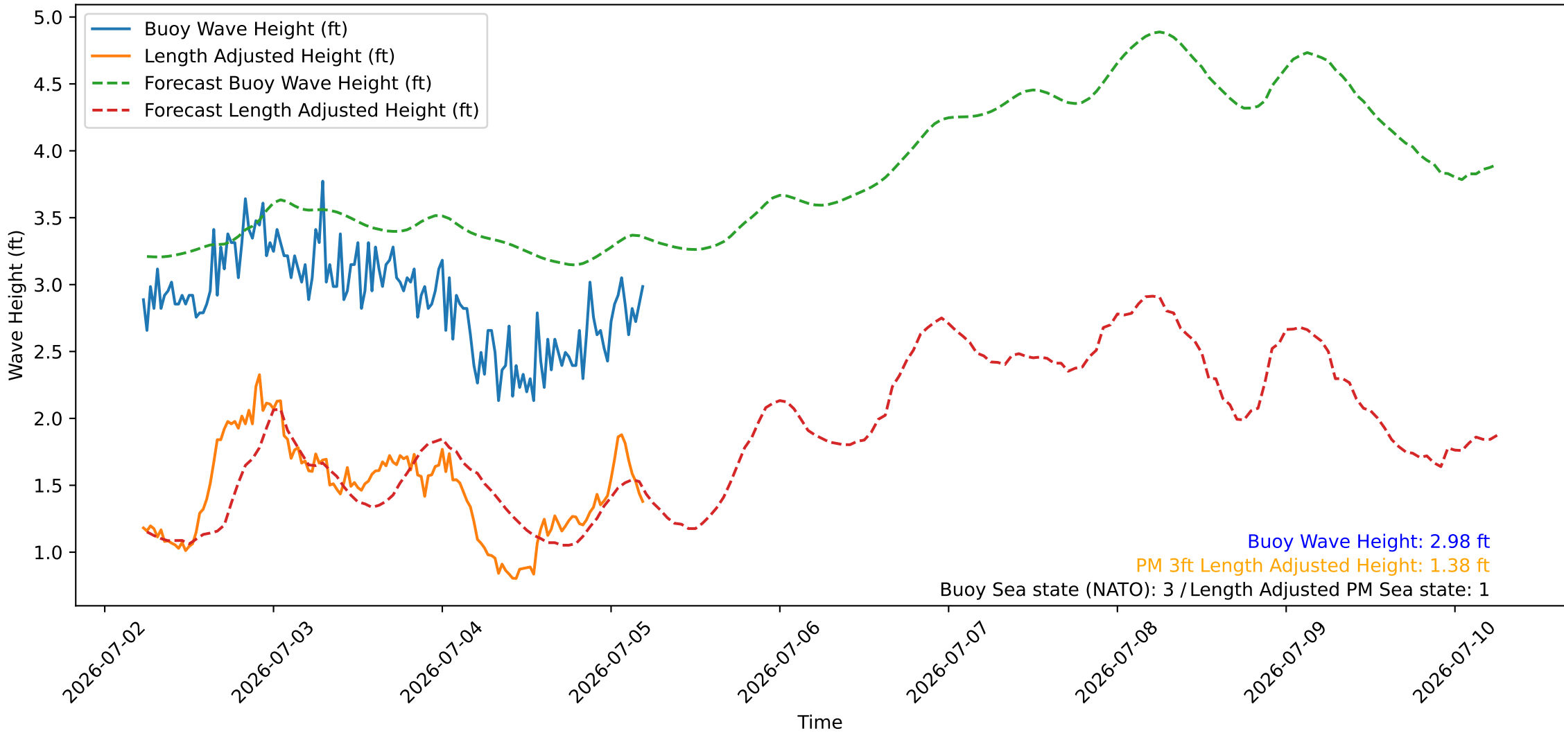
Wave Heights over Time for Oceanside Harbor at 2026-07-05 05:30:26
