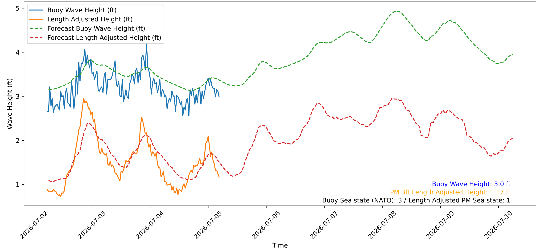
Wave Heights over Time for Green Beach at 2026-07-05 05:31:08
