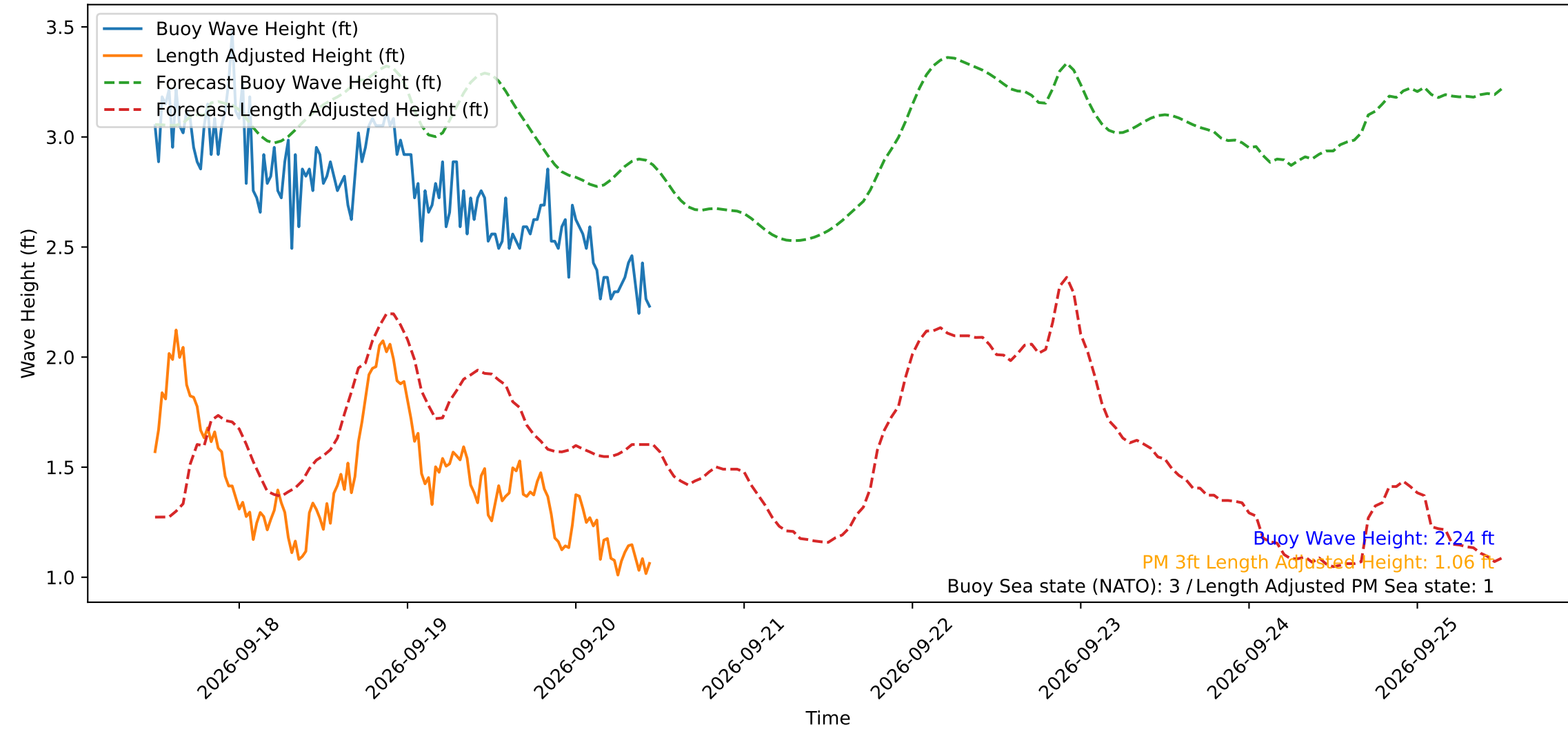
Wave Heights over Time for Green Beach at 2026-09-20 11:31:11
