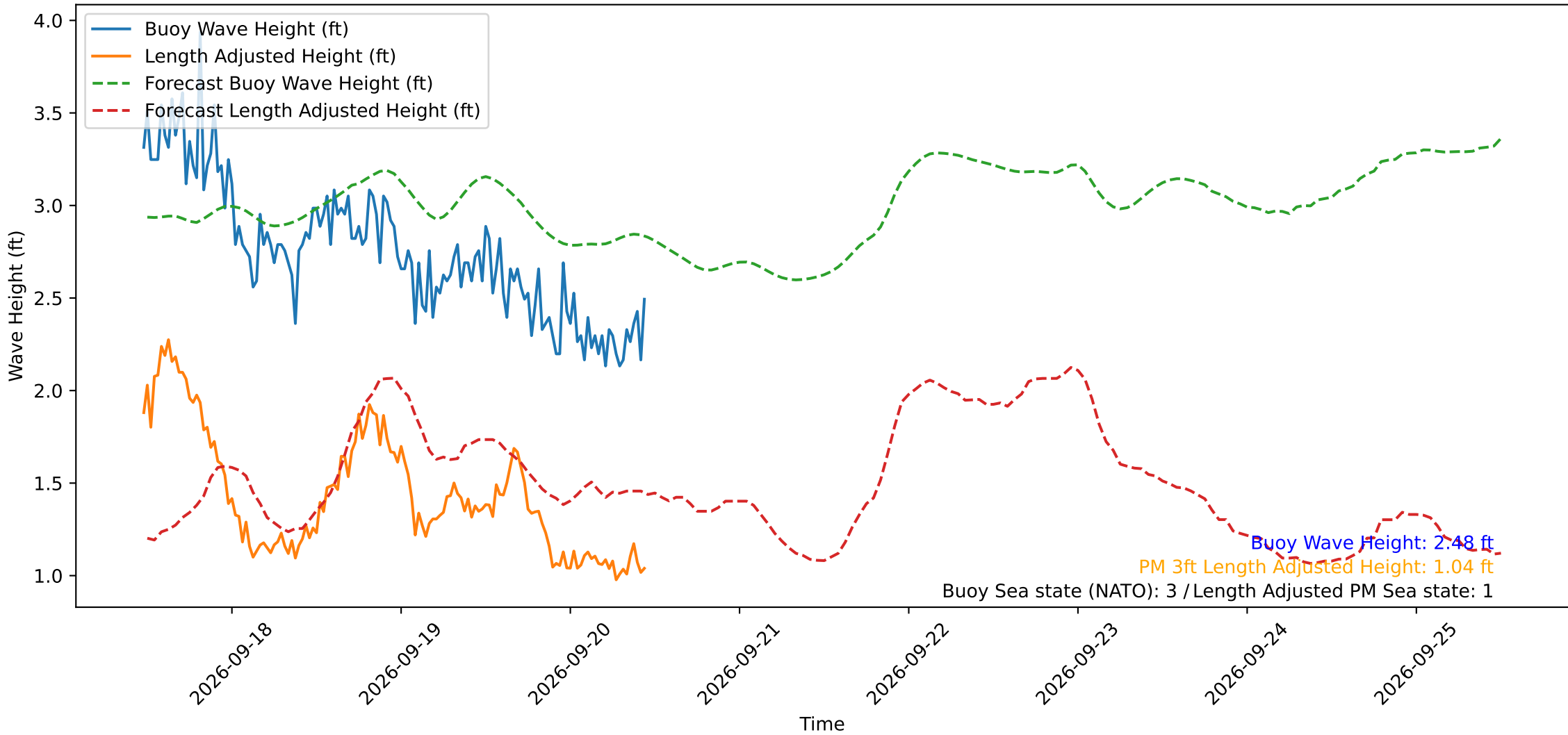
Wave Heights over Time for Oceanside Harbor at 2026-09-20 11:30:29
