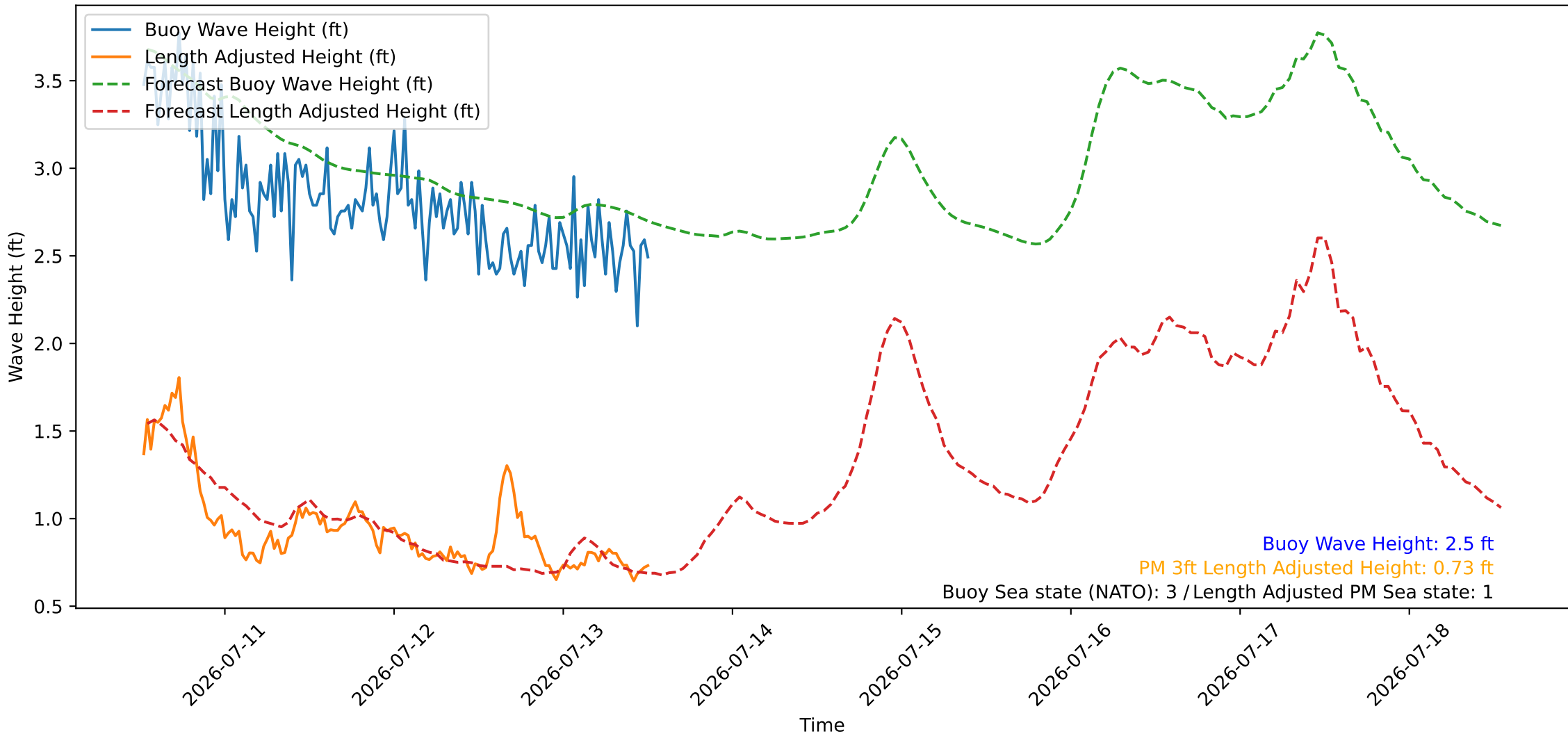
Wave Heights over Time for Oceanside Harbor at 2026-07-13 12:40:26
