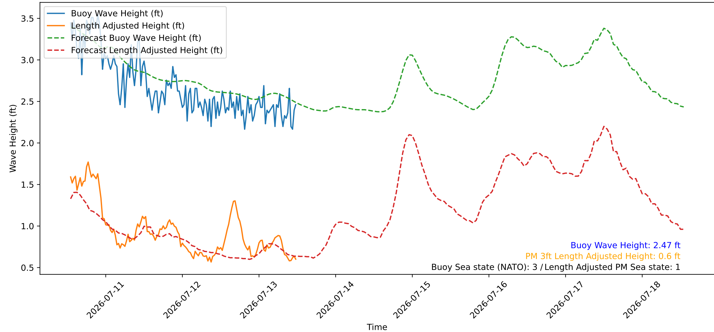
Wave Heights over Time for Red Beach at 2026-07-13 12:40:46
