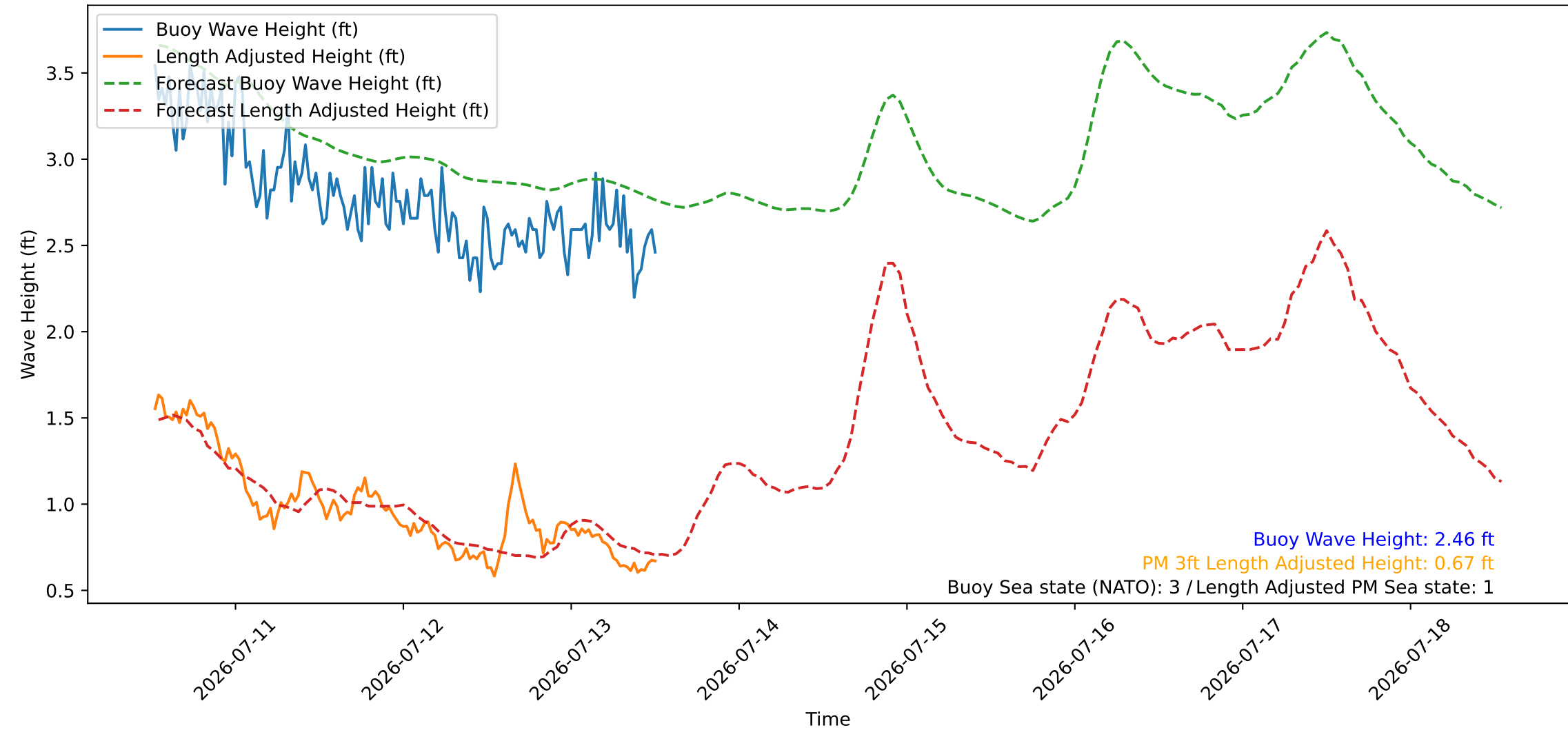
Wave Heights over Time for Green Beach at 2026-07-13 12:41:08
