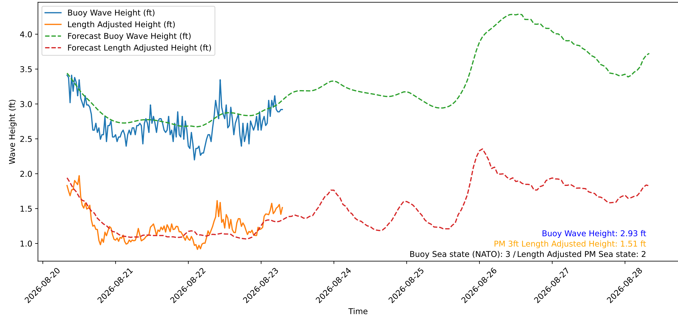
Wave Heights over Time for Oceanside Harbor at 2026-08-23 08:00:30
