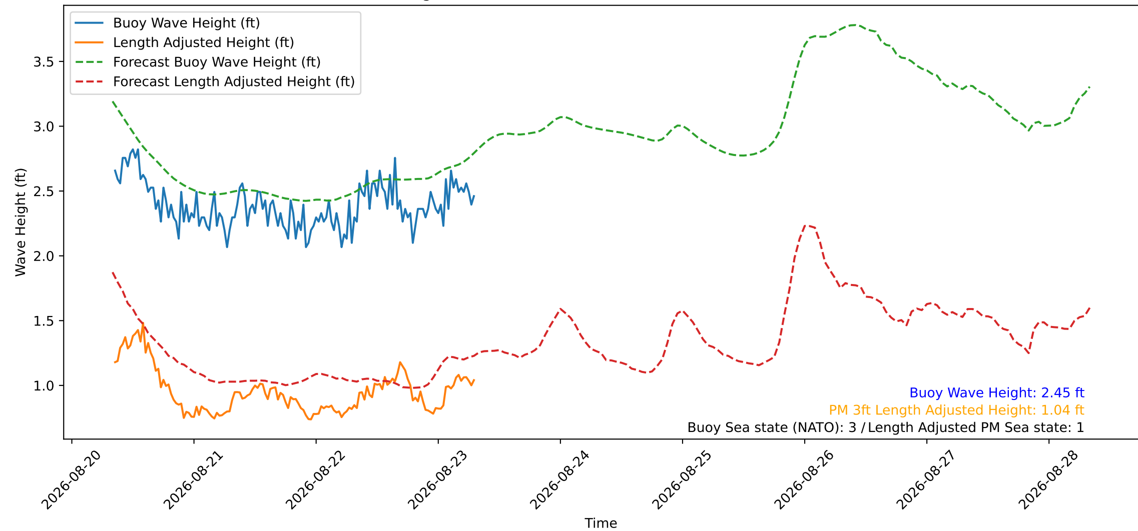
Wave Heights over Time for Red Beach at 2026-08-23 08:00:50
