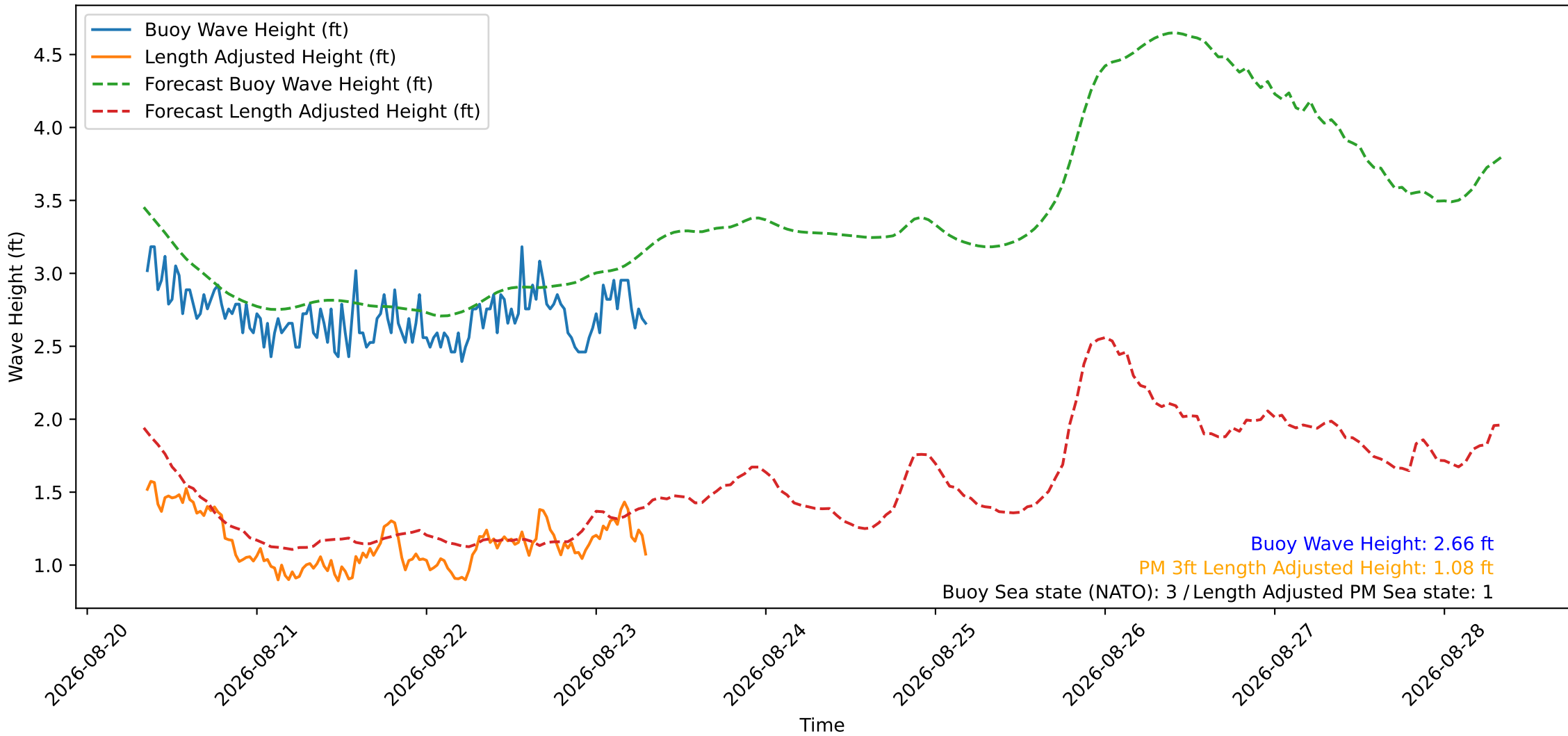
Wave Heights over Time for Green Beach at 2026-08-23 08:01:13
