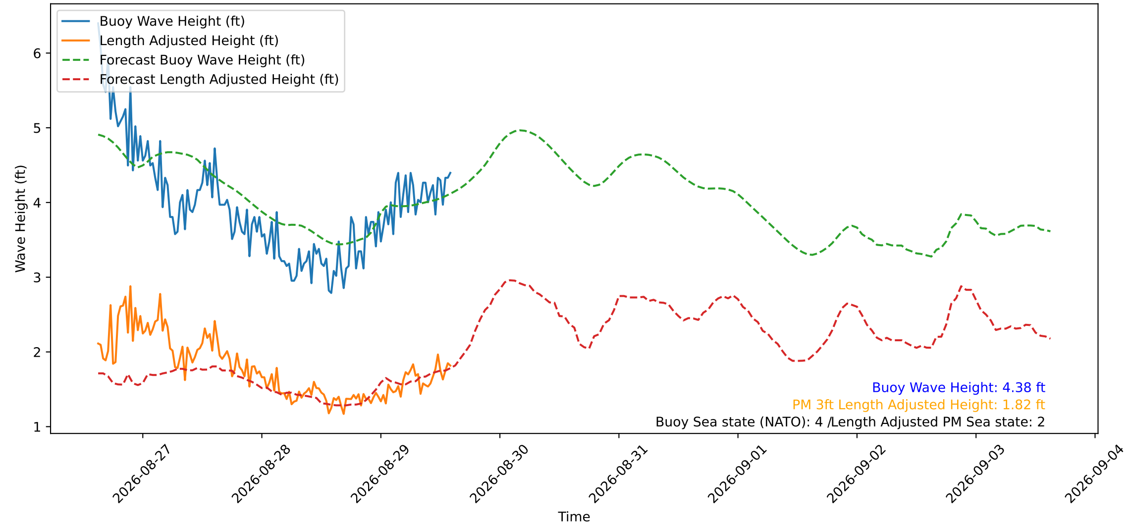
Wave Heights over Time for Oceanside Harbor at 2026-08-29 15:00:29
