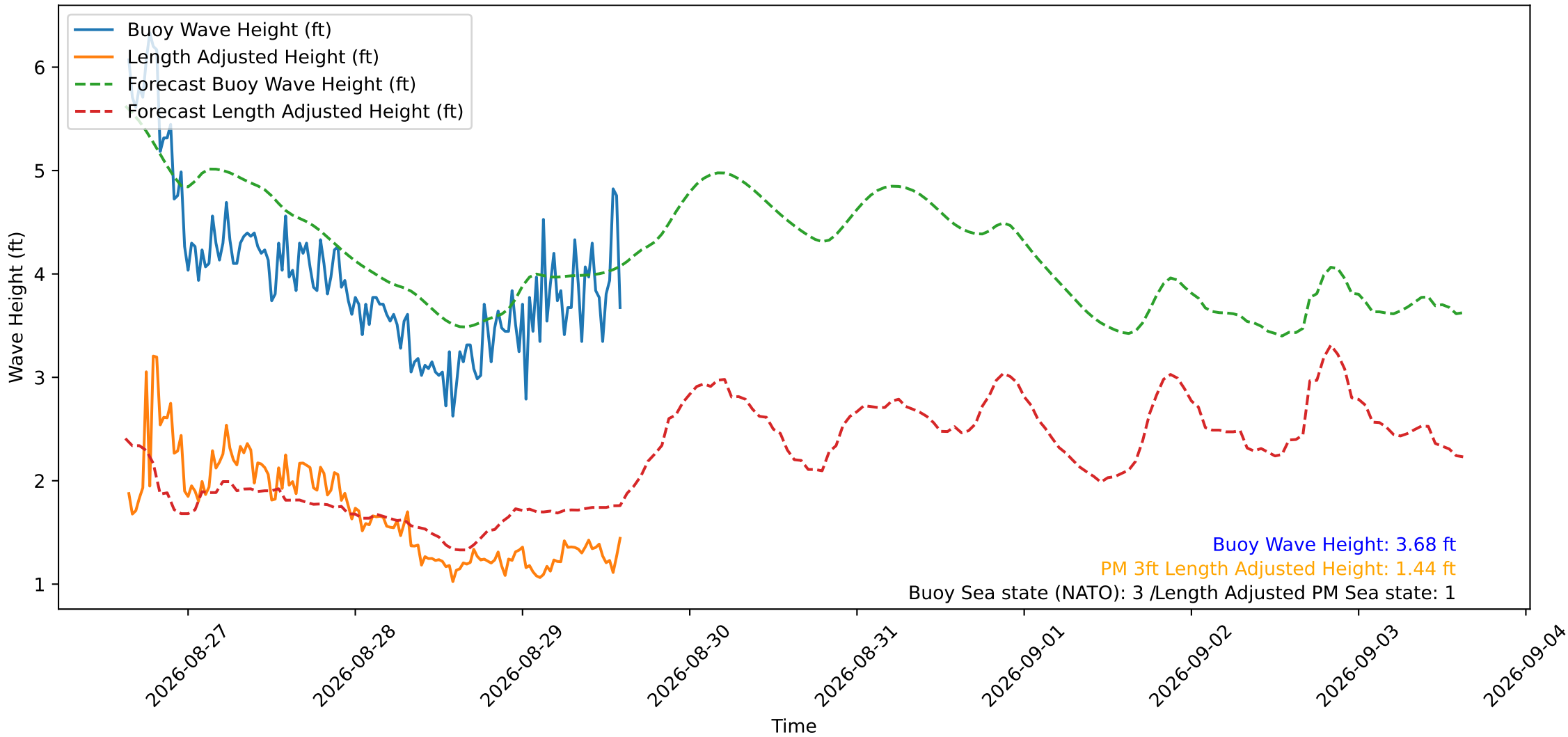
Wave Heights over Time for Green Beach at 2026-08-29 15:01:11
