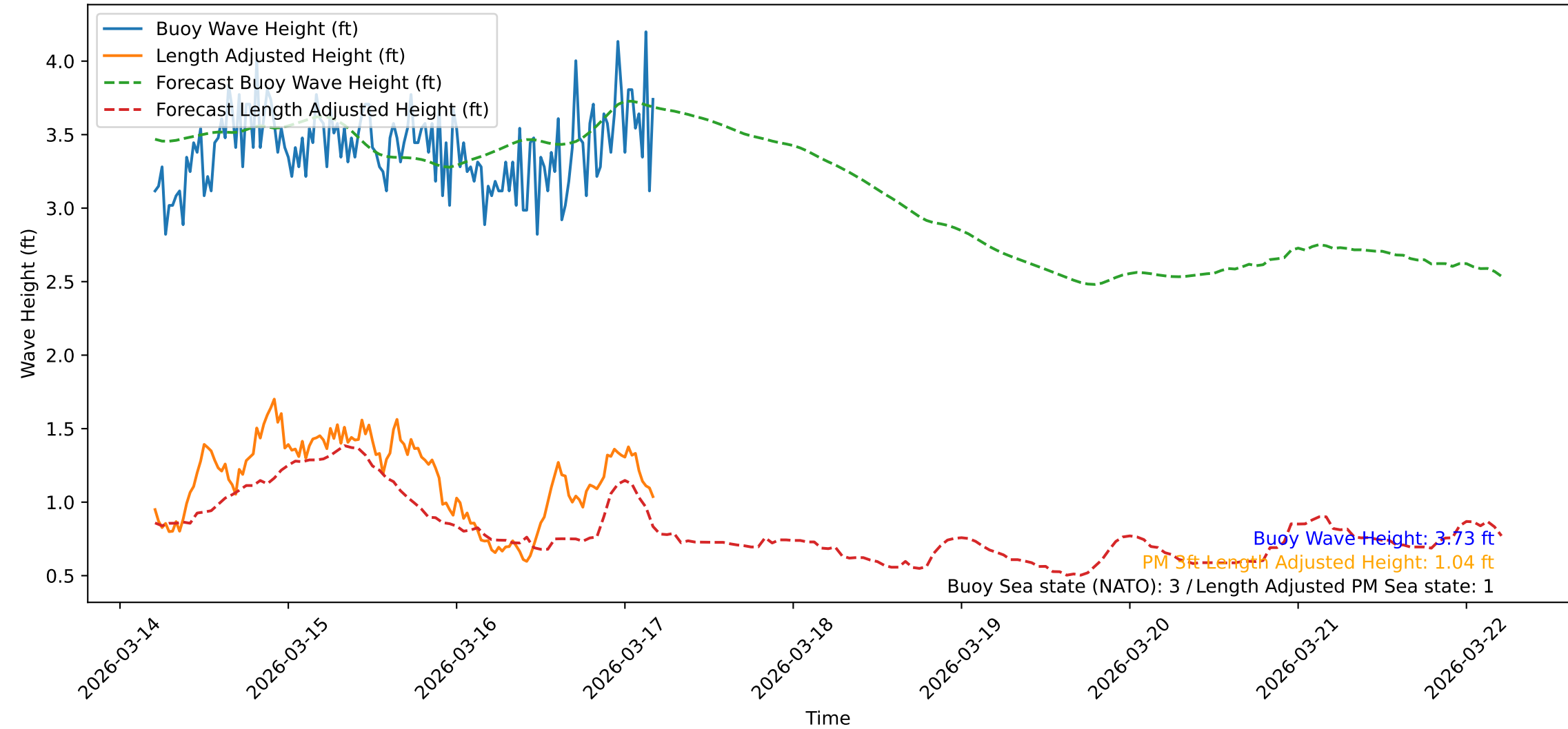
Wave Heights over Time for Green Beach at 2026-03-17 05:01:47
