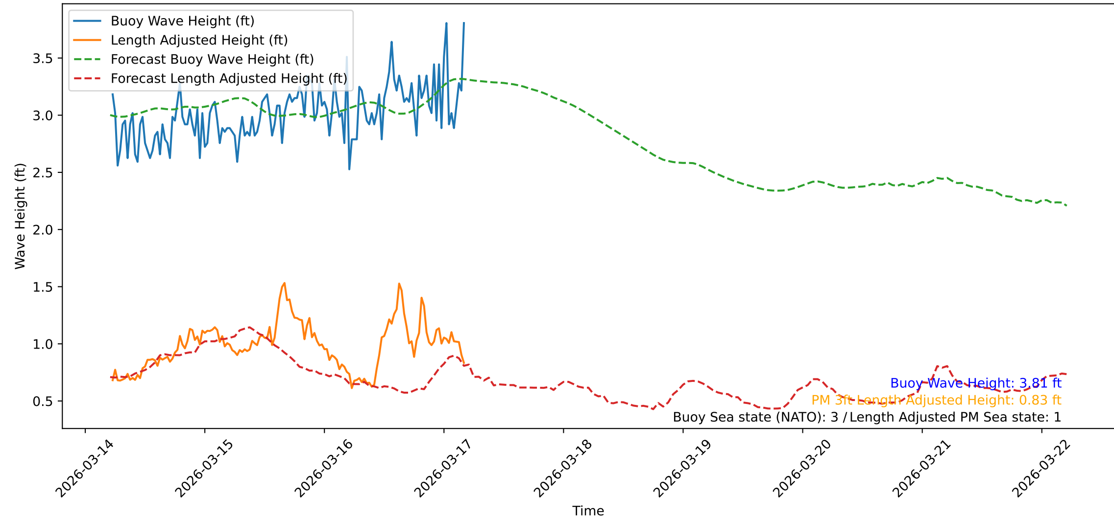
Wave Heights over Time for Red Beach at 2026-03-17 05:01:08
