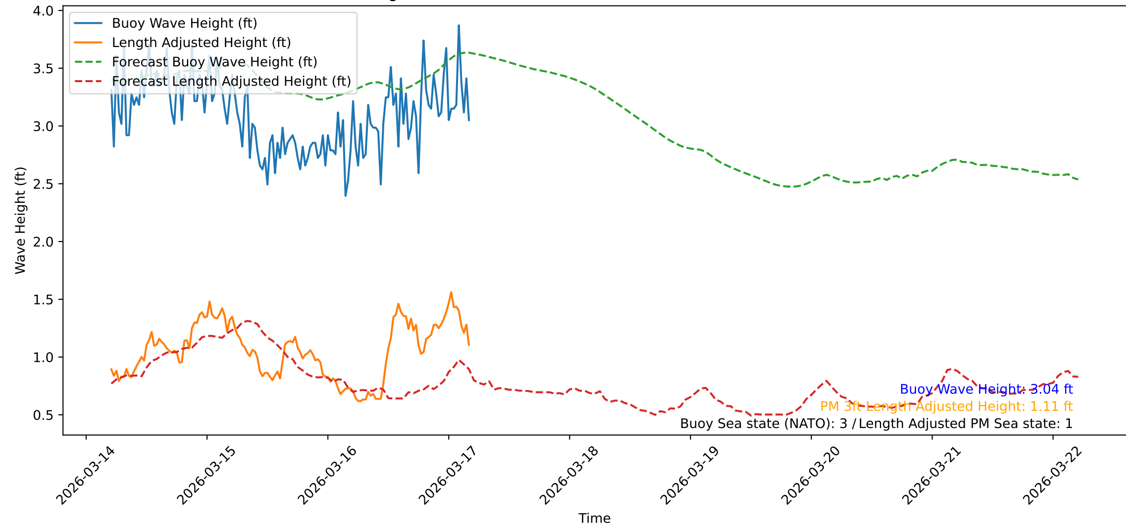
Wave Heights over Time for Oceanside Harbor at 2026-03-17 05:00:45
