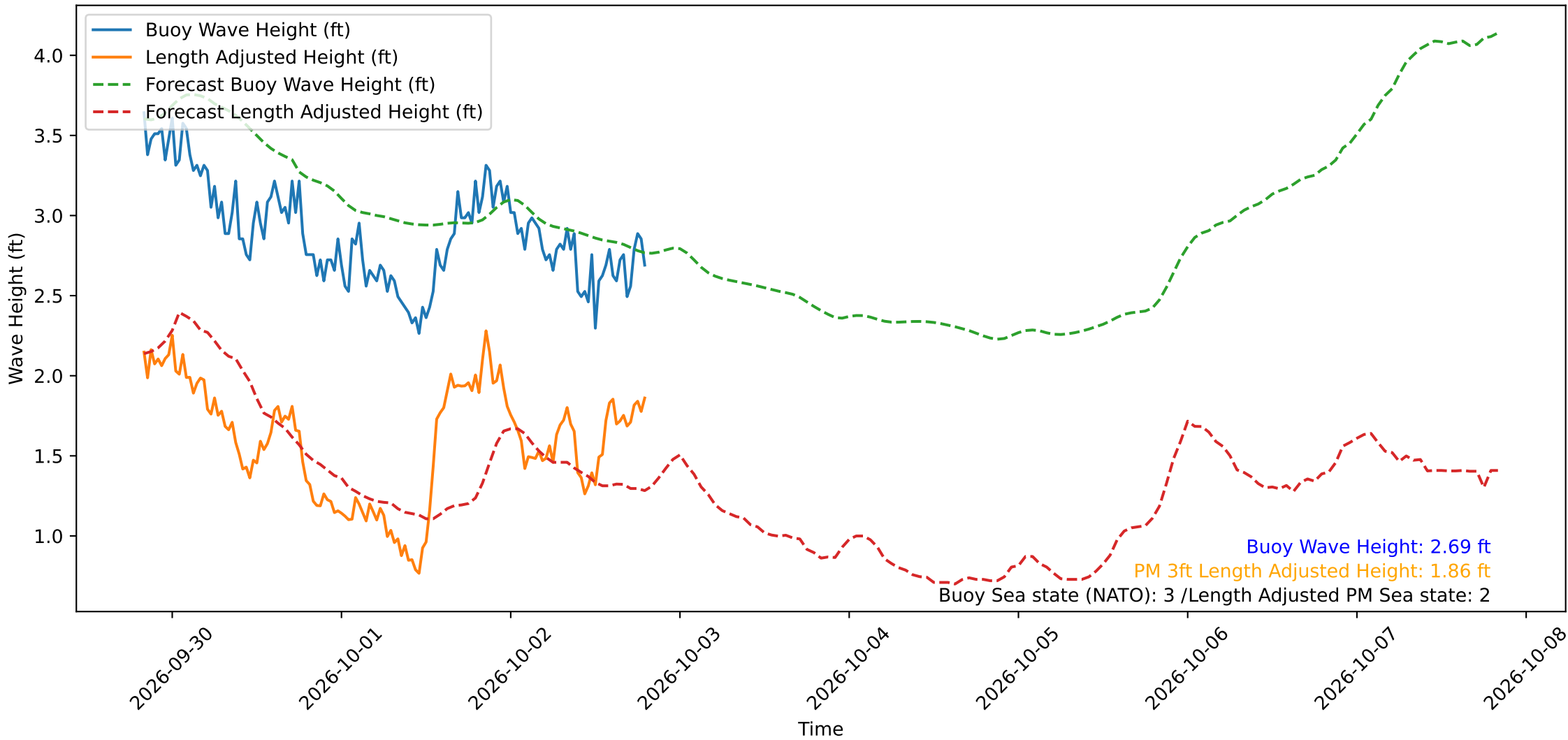
Wave Heights over Time for Oceanside Harbor at 2026-10-02 20:00:29
