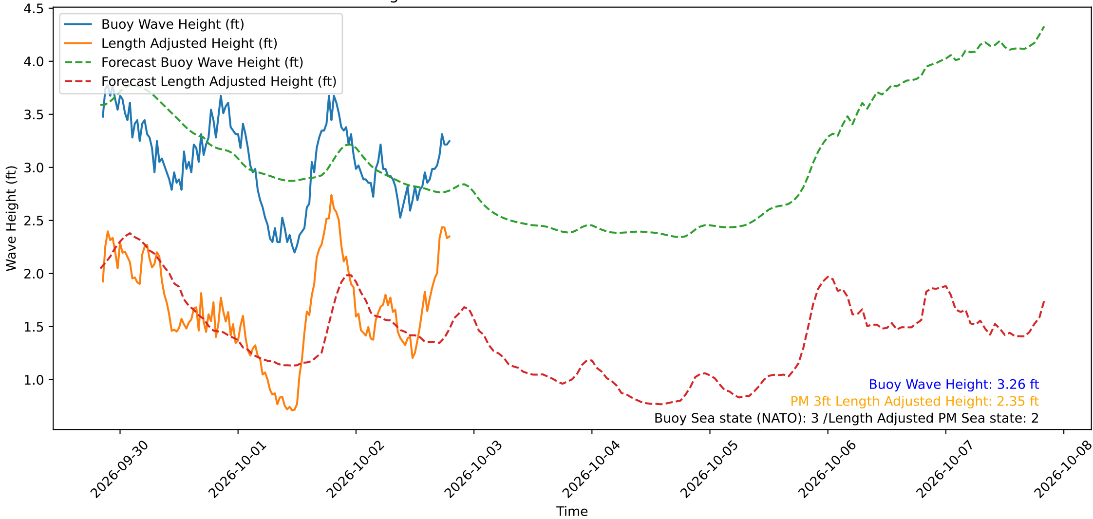
Wave Heights over Time for Green Beach at 2026-10-02 20:01:12
