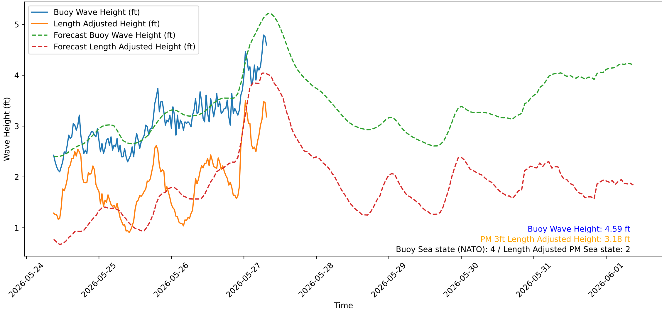
Wave Heights over Time for Red Beach at 2026-05-27 08:30:44
