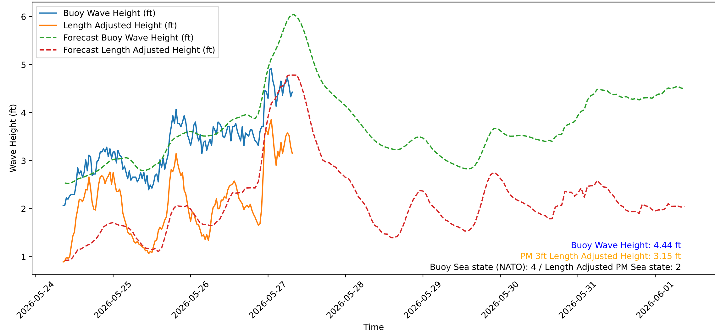
Wave Heights over Time for Green Beach at 2026-05-27 08:31:07
