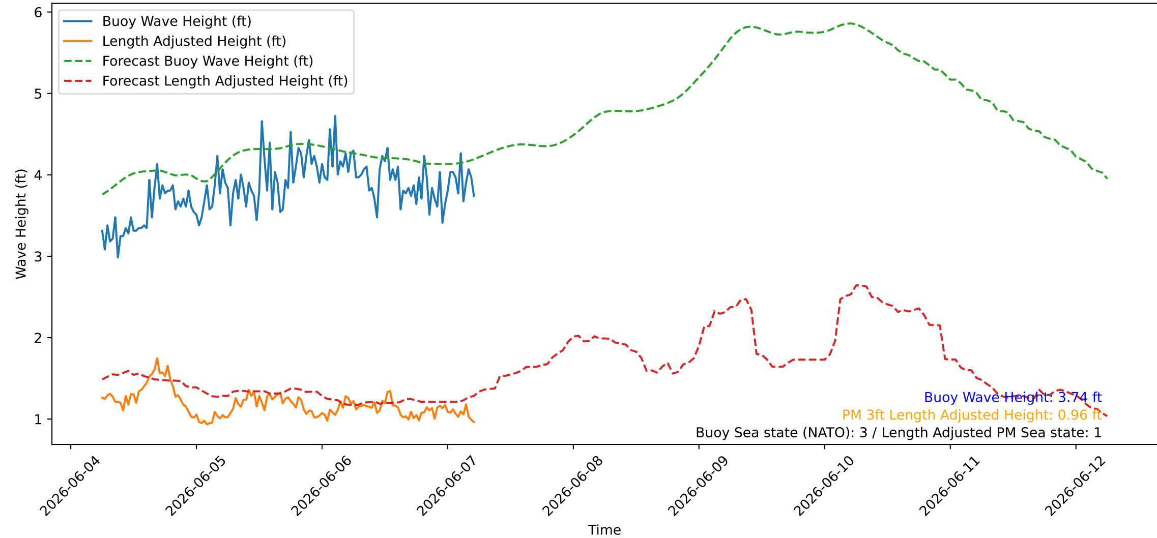
Wave Heights over Time for Green Beach at 2026-06-07 06:01:07
