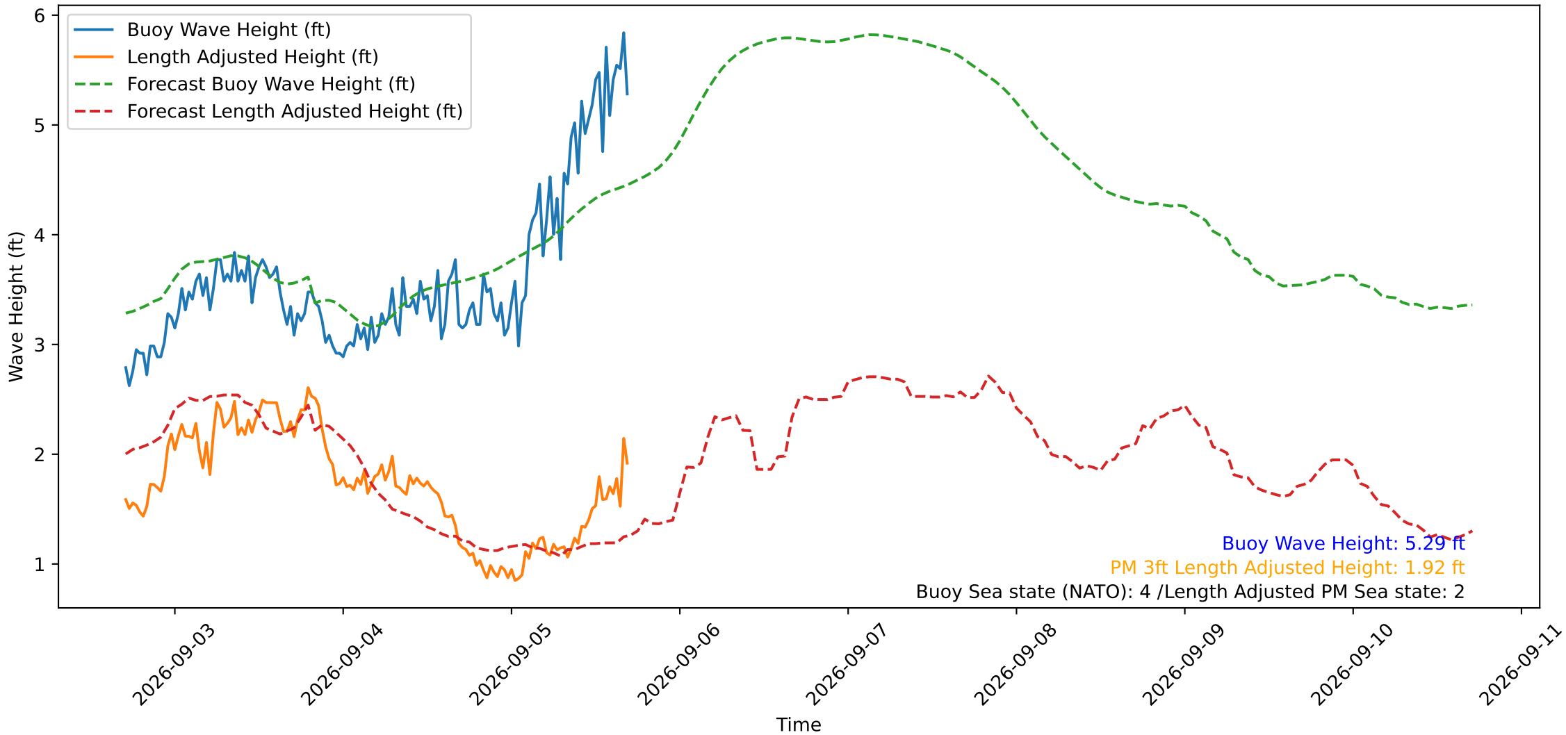
Wave Heights over Time for Oceanside Harbor at 2026-09-05 17:10:30
