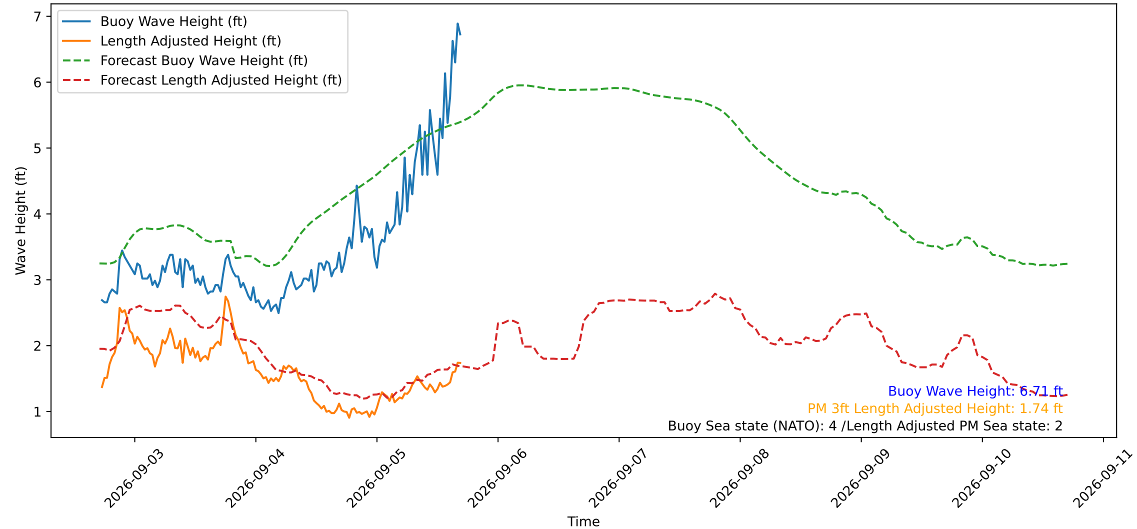
Wave Heights over Time for Green Beach at 2026-09-05 17:11:13
