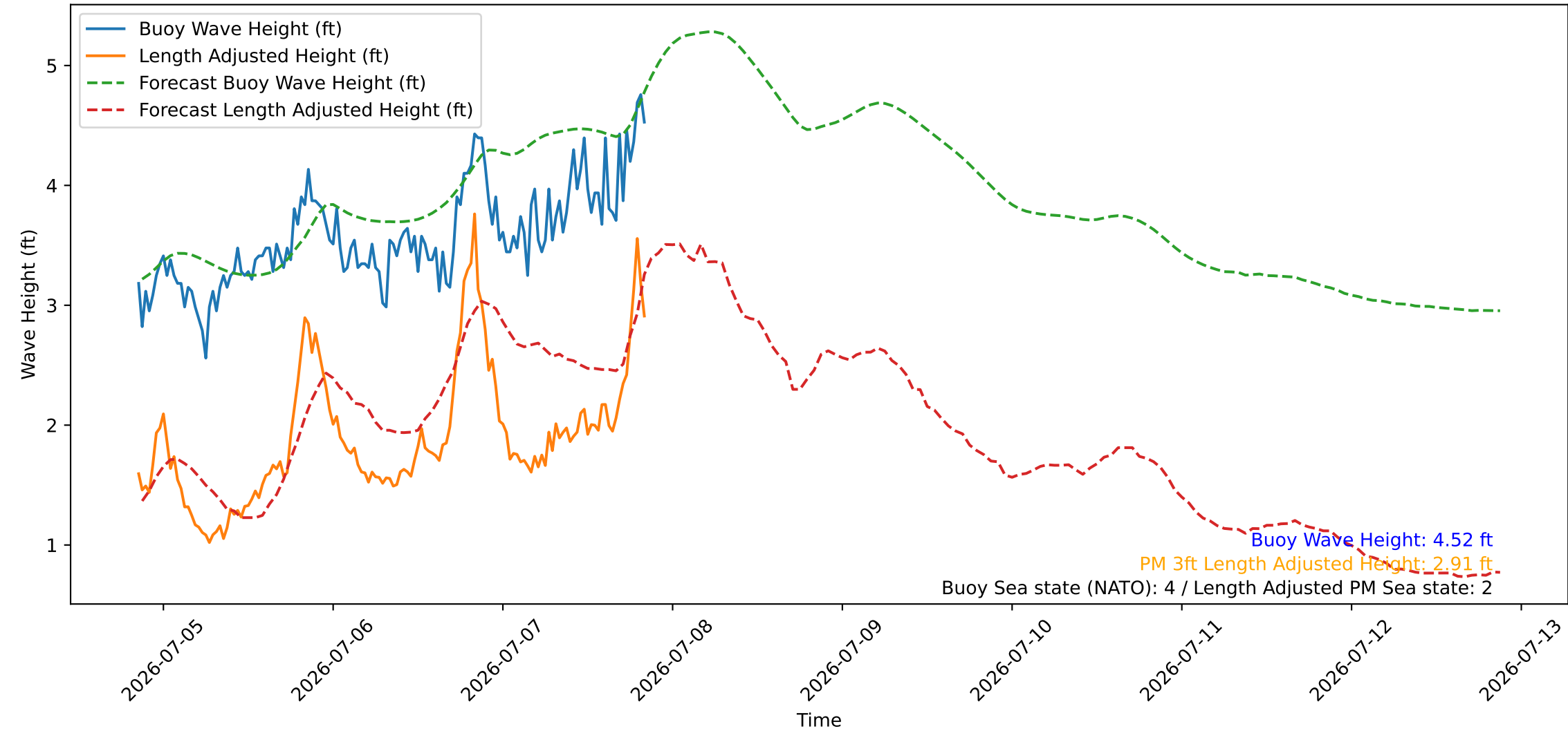
Wave Heights over Time for Green Beach at 2026-07-07 20:41:09
