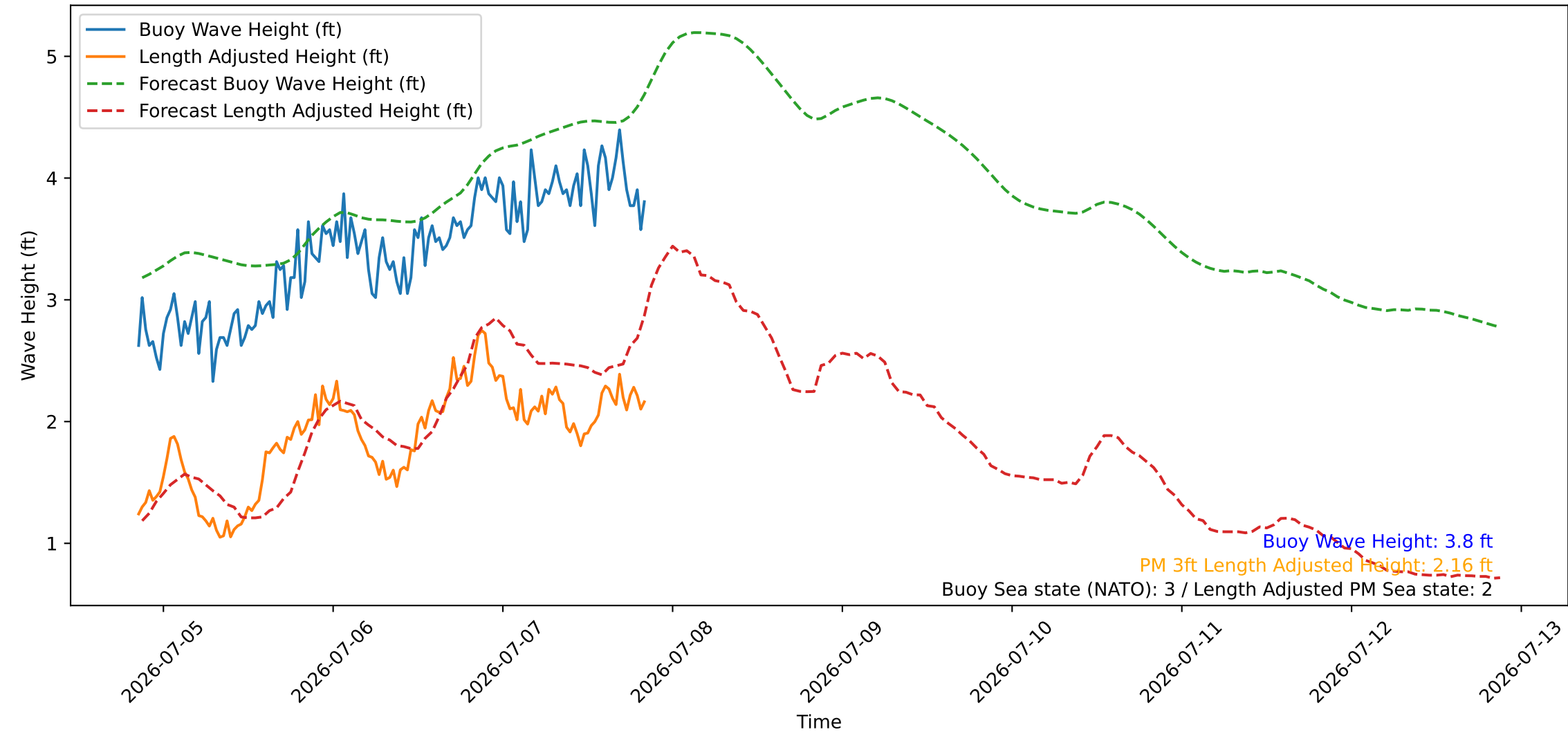
Wave Heights over Time for Oceanside Harbor at 2026-07-07 20:40:26
