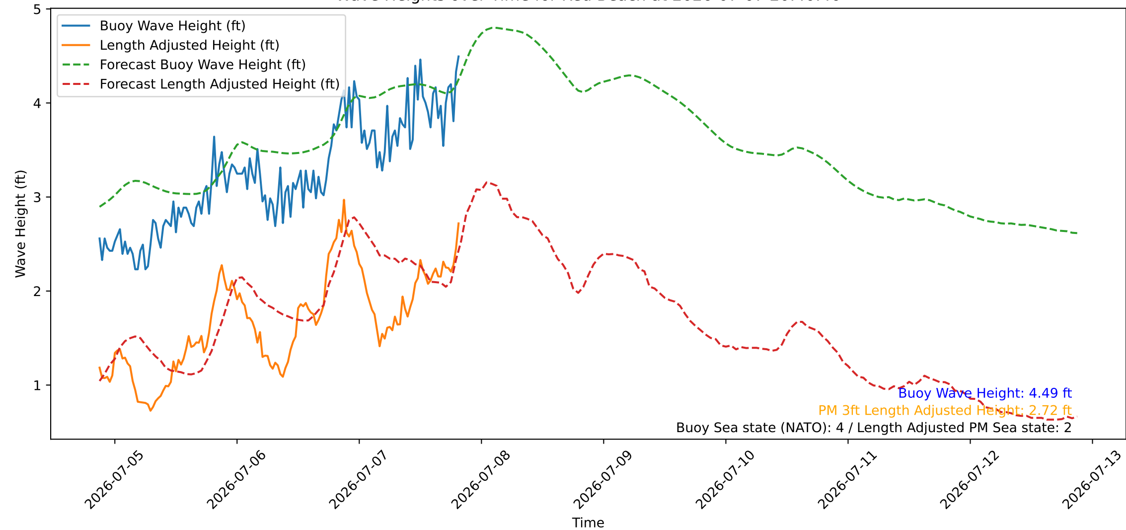
Wave Heights over Time for Red Beach at 2026-07-07 20:40:46
