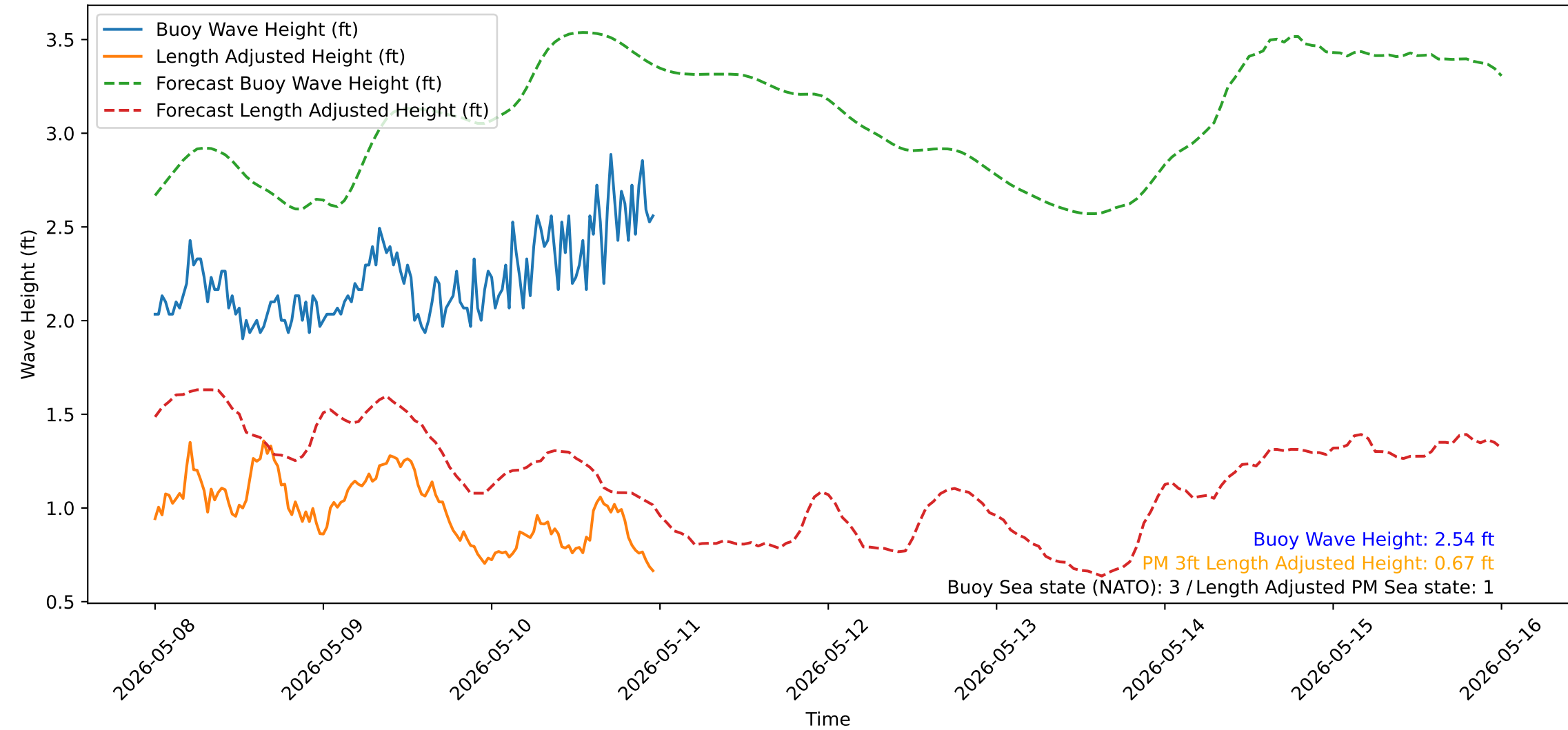
Wave Heights over Time for Red Beach at 2026-05-10 23:40:50
