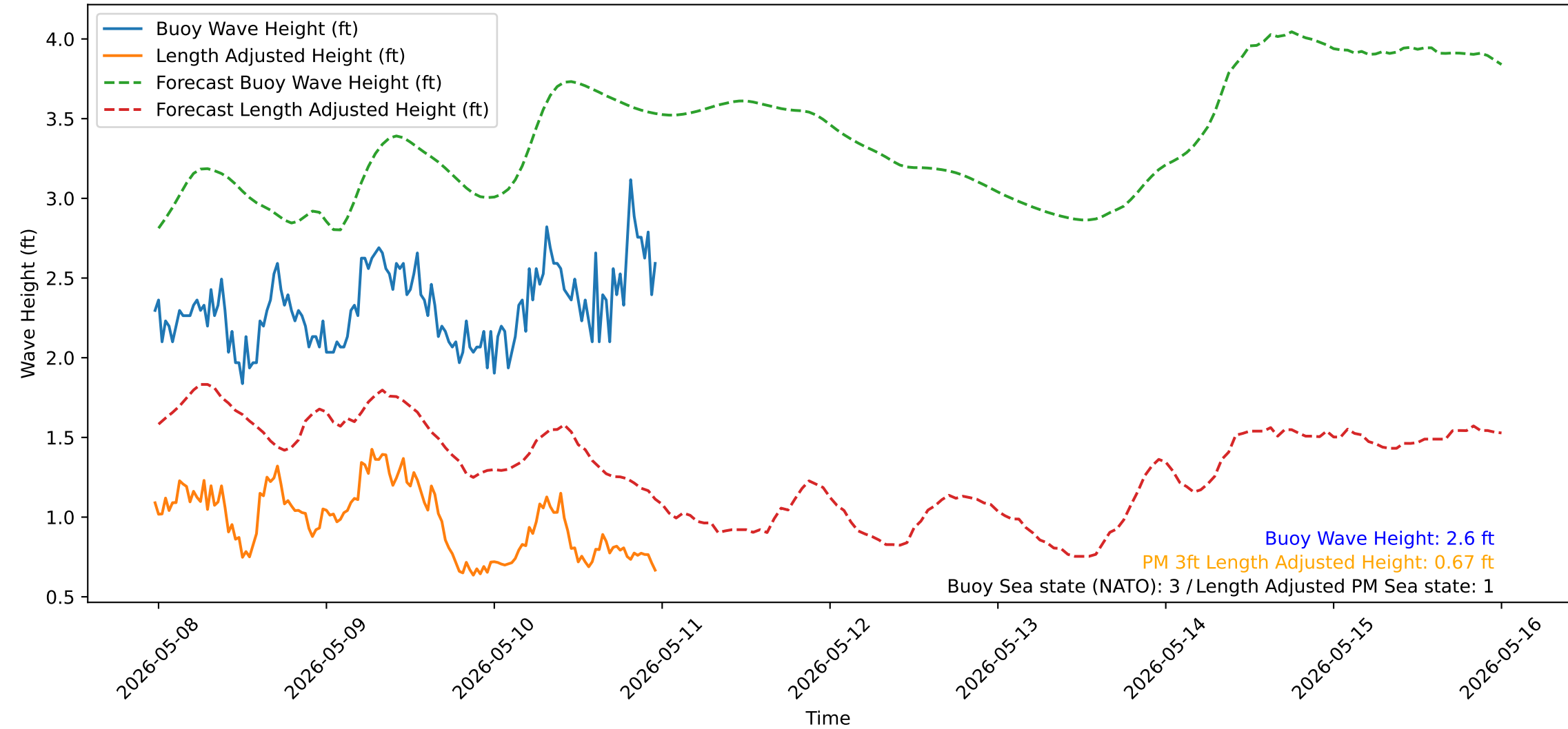
Wave Heights over Time for Green Beach at 2026-05-10 23:41:12
