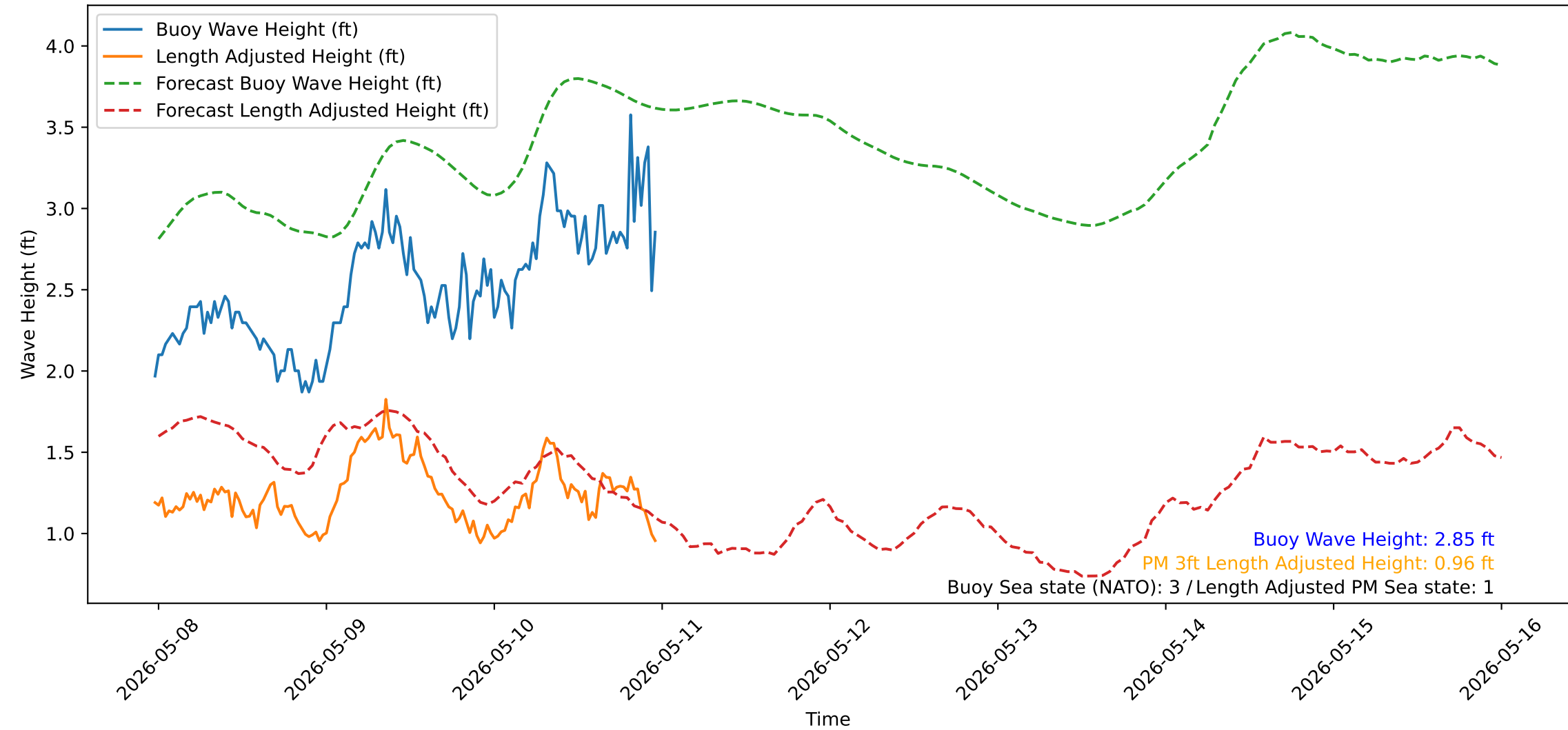
Wave Heights over Time for Oceanside Harbor at 2026-05-10 23:40:31
