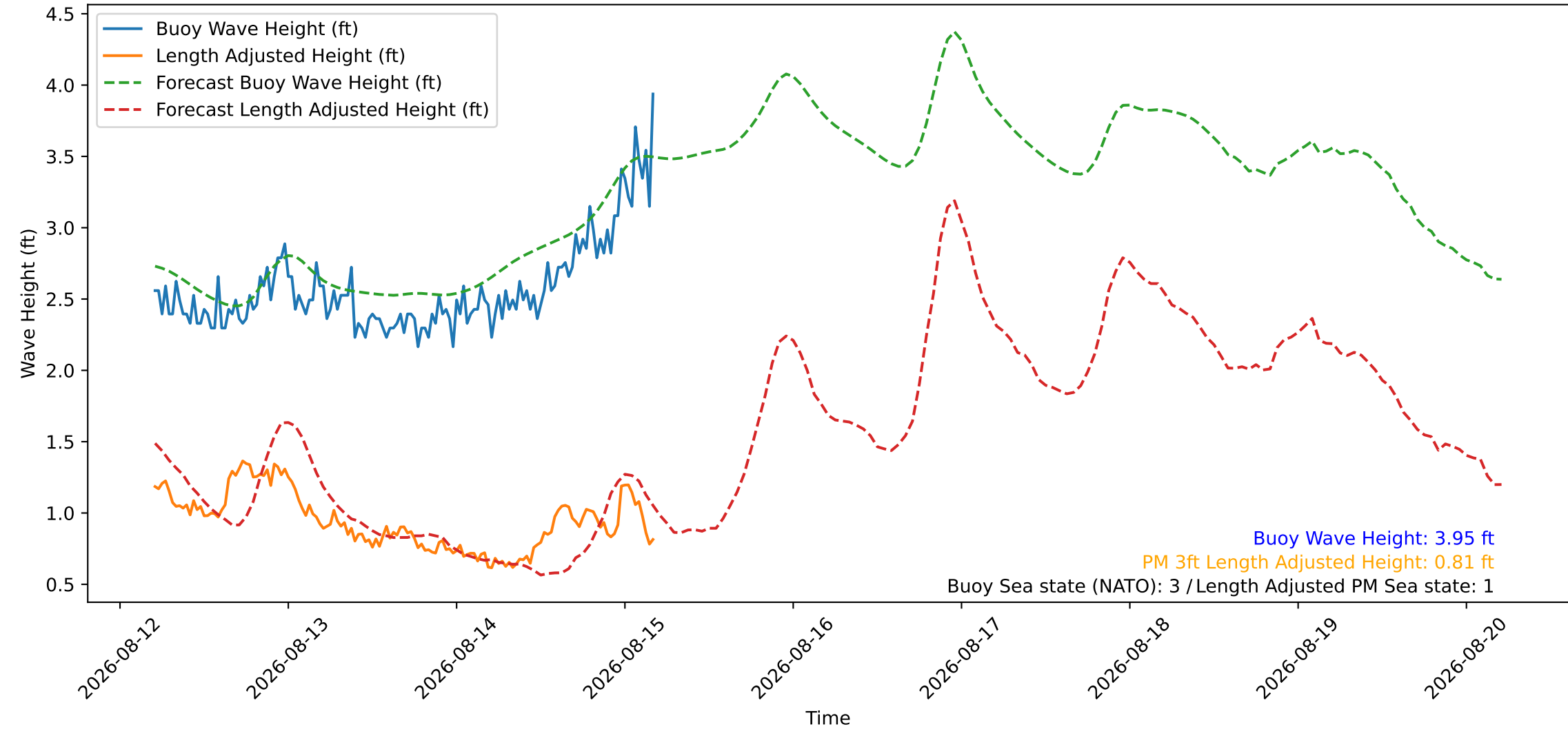
Wave Heights over Time for Red Beach at 2026-08-15 04:50:47
