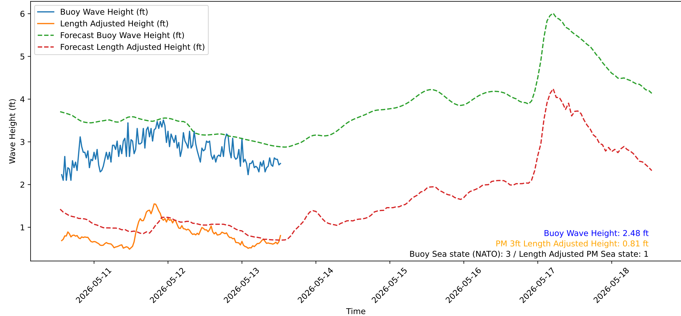
Wave Heights over Time for Green Beach at 2026-05-13 13:21:14
