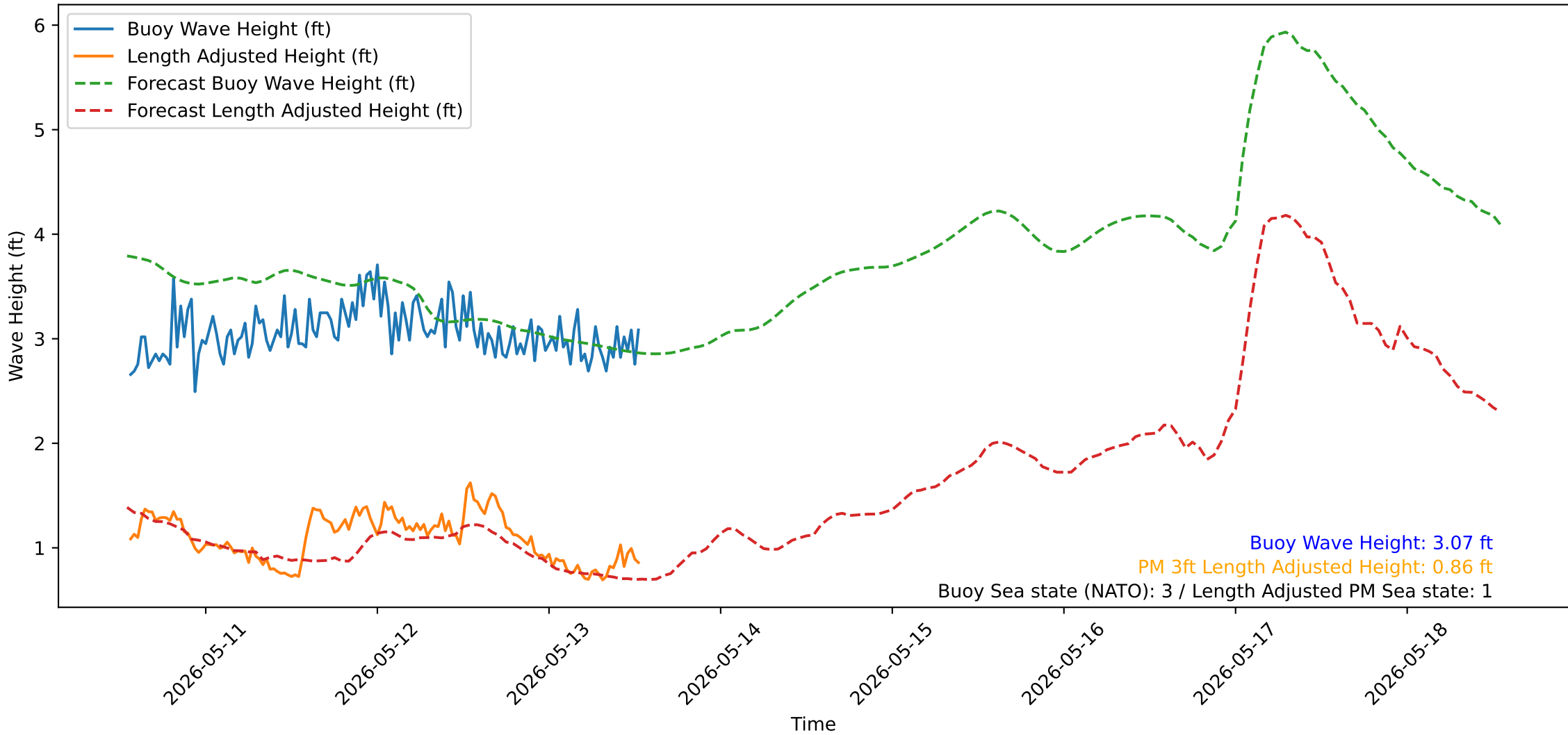
Wave Heights over Time for Oceanside Harbor at 2026-05-13 13:20:31
