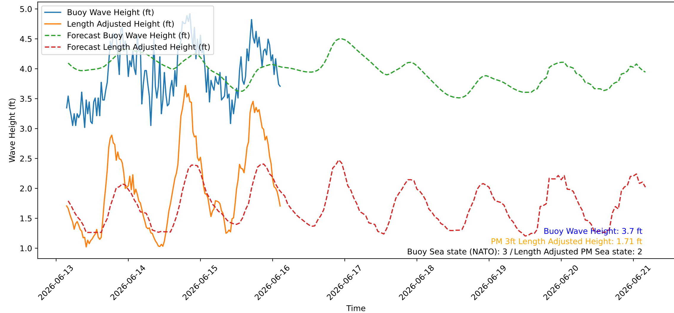
Wave Heights over Time for Green Beach at 2026-06-16 03:31:07
