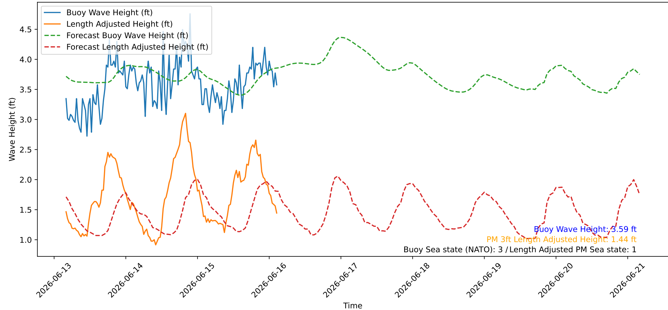
Wave Heights over Time for Red Beach at 2026-06-16 03:30:44
