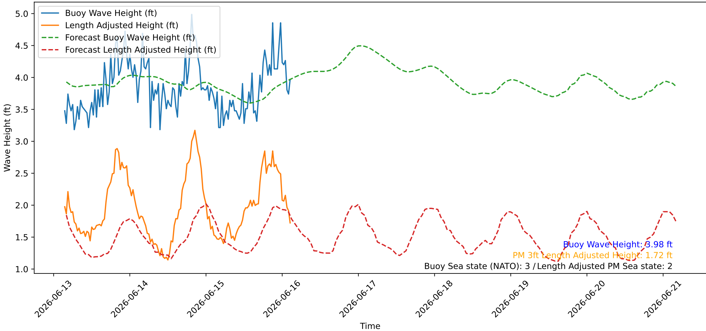
Wave Heights over Time for Oceanside Harbor at 2026-06-16 03:30:26
