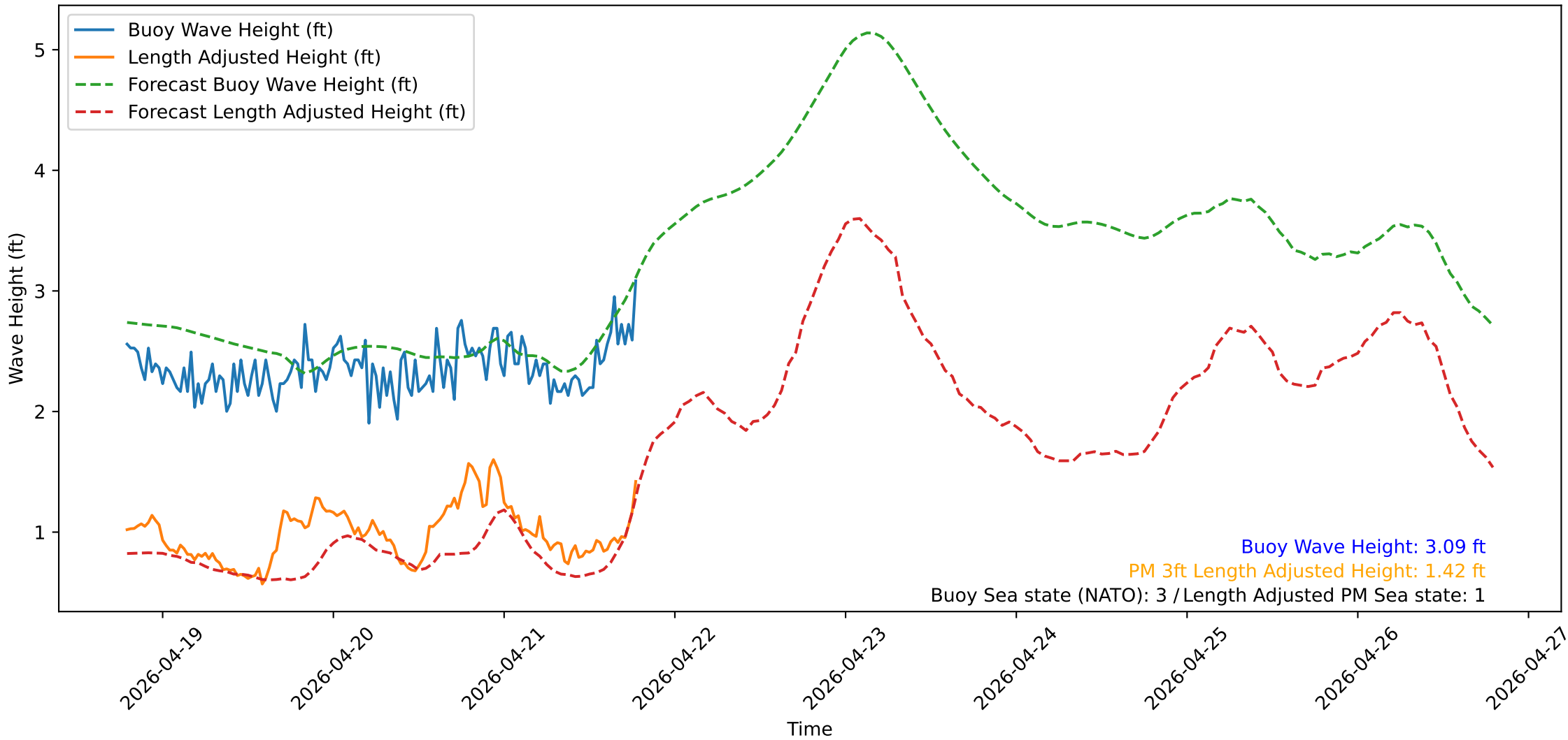
Wave Heights over Time for Oceanside Harbor at 2026-04-21 19:10:31
