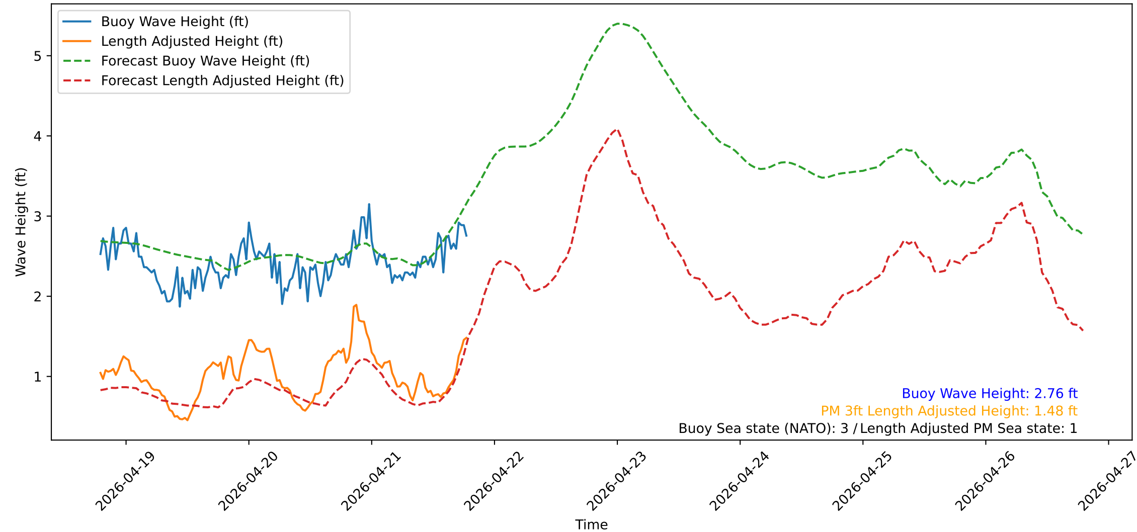
Wave Heights over Time for Green Beach at 2026-04-21 19:11:13
