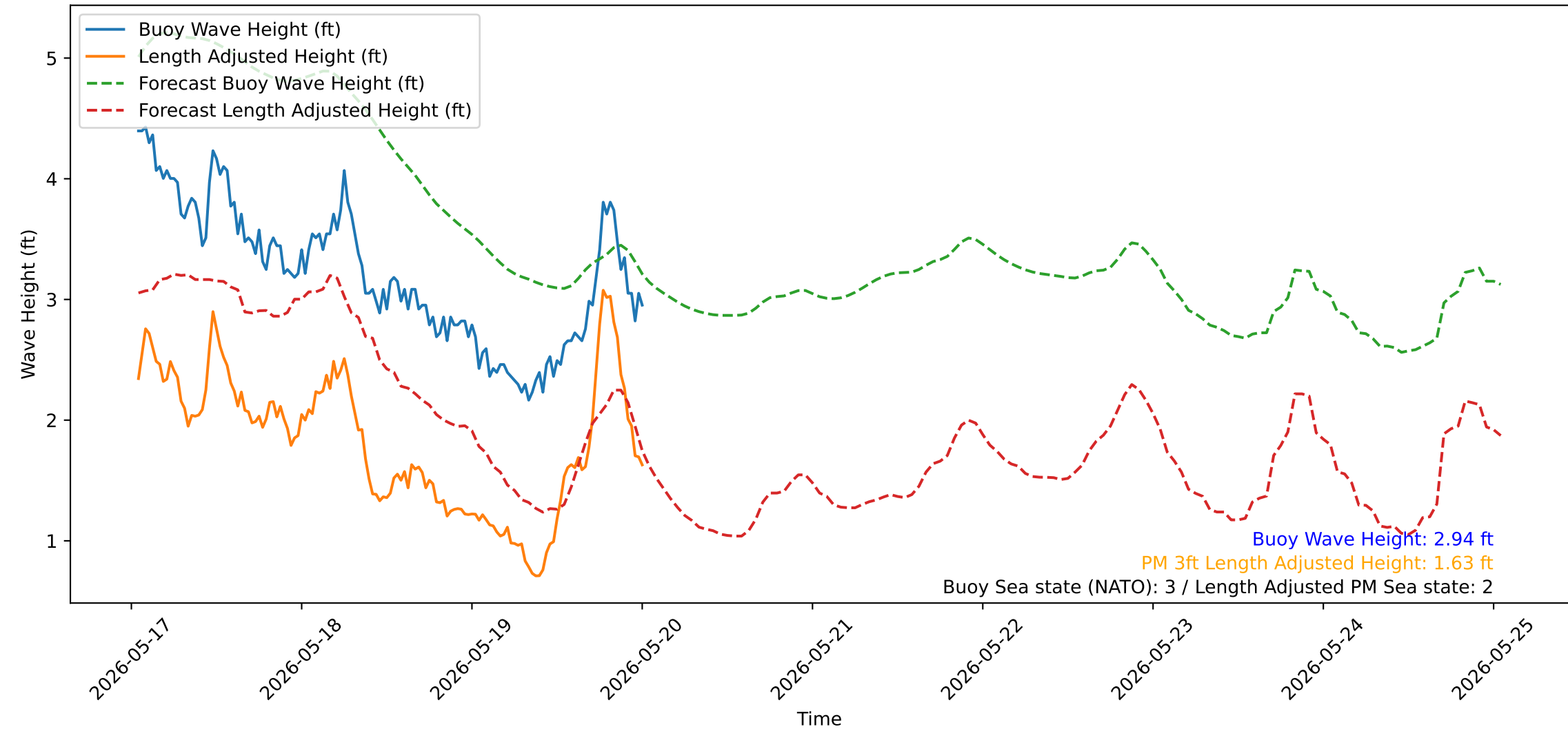
Wave Heights over Time for Green Beach at 2026-05-20 00:51:15
