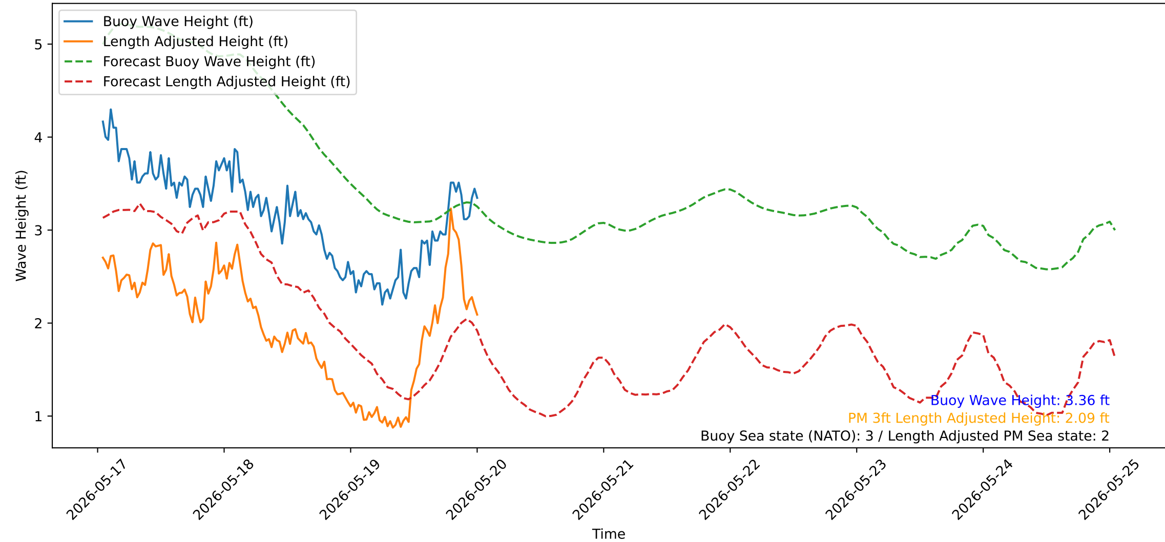
Wave Heights over Time for Oceanside Harbor at 2026-05-20 00:50:31
