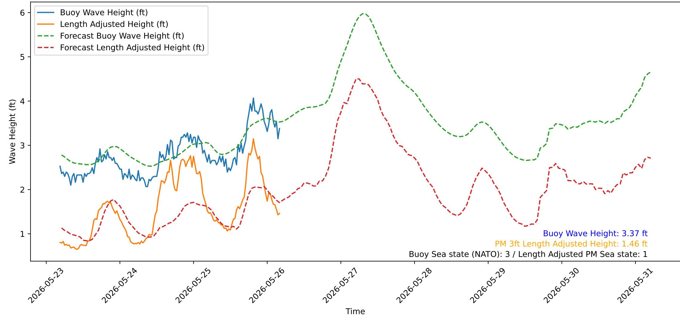
Wave Heights over Time for Green Beach at 2026-05-26 04:41:10
