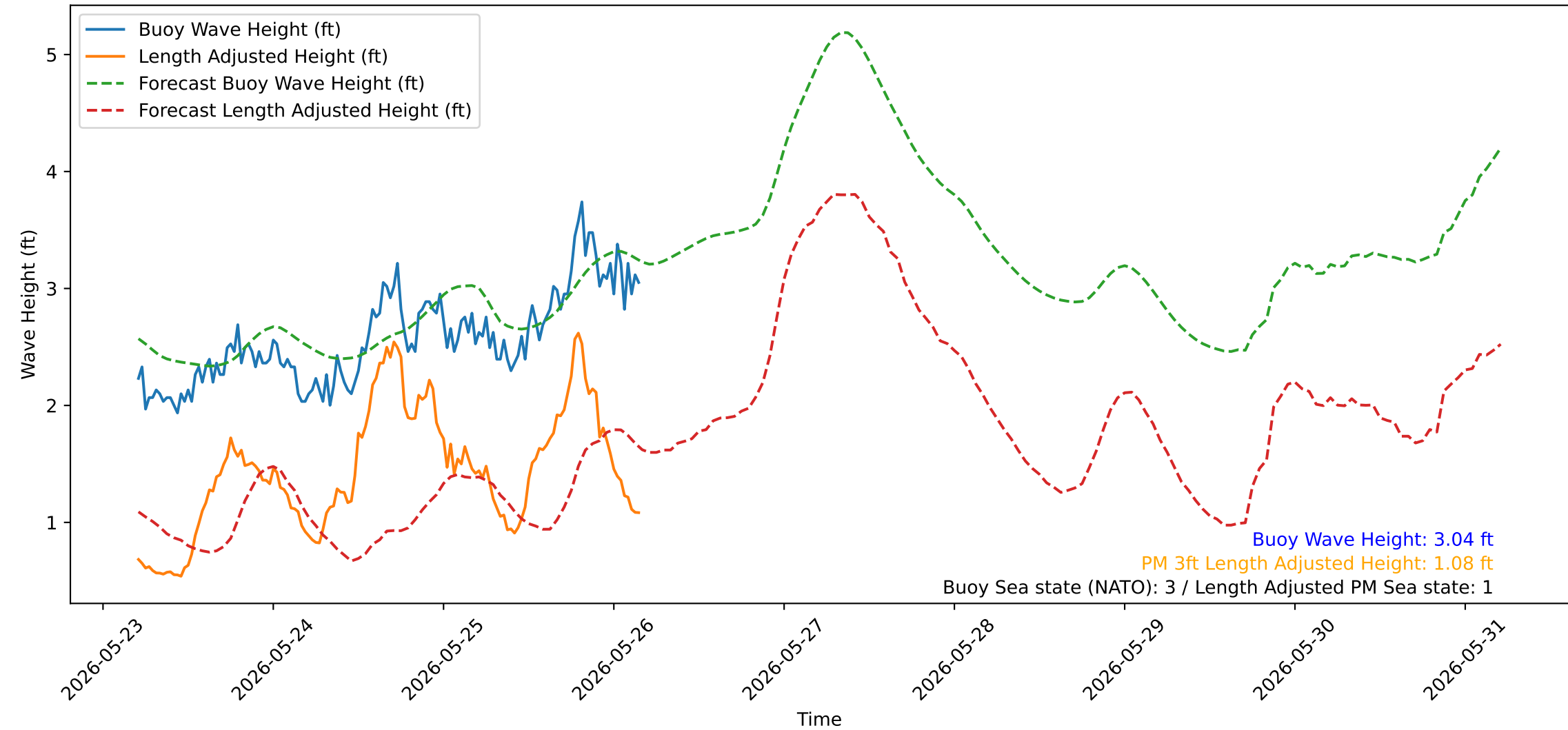
Wave Heights over Time for Red Beach at 2026-05-26 04:40:48
