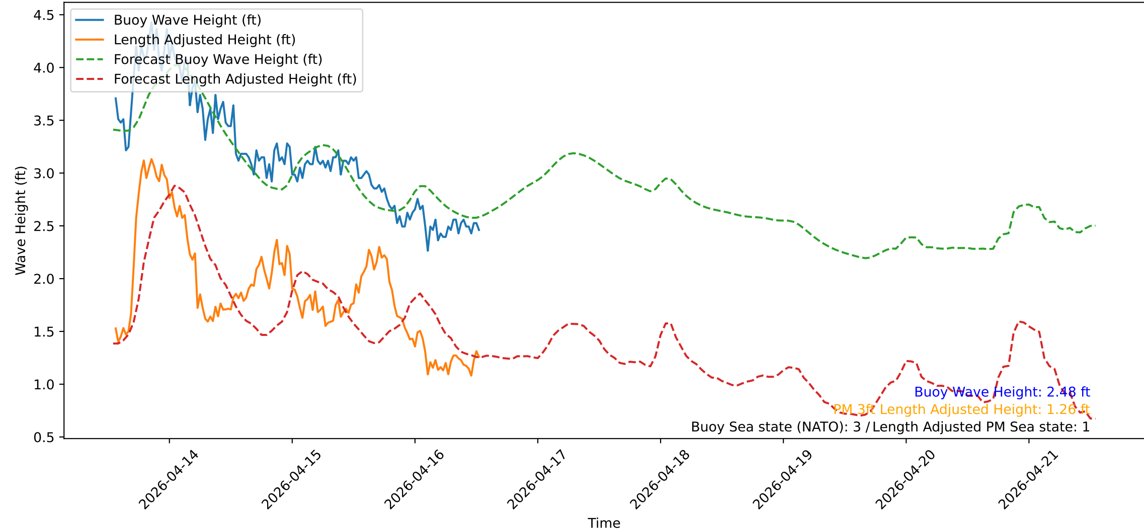
Wave Heights over Time for Red Beach at 2026-04-16 13:10:50
