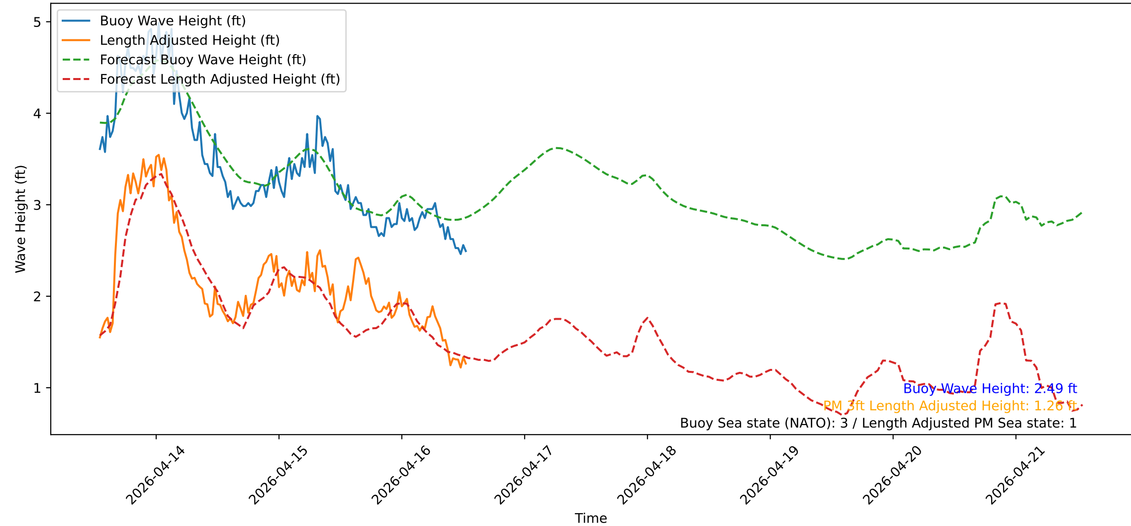
Wave Heights over Time for Green Beach at 2026-04-16 13:11:13
