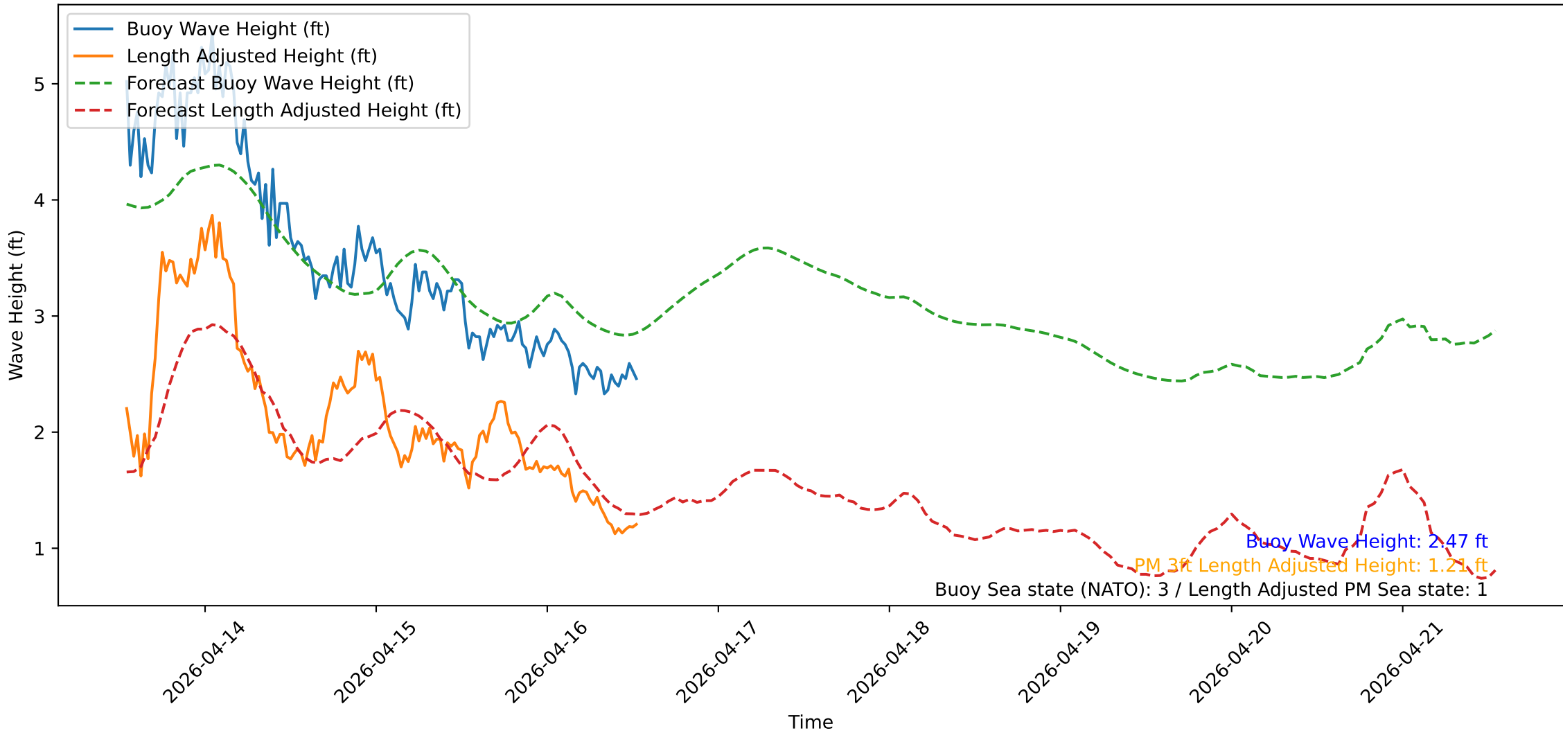
Wave Heights over Time for Oceanside Harbor at 2026-04-16 13:10:31
