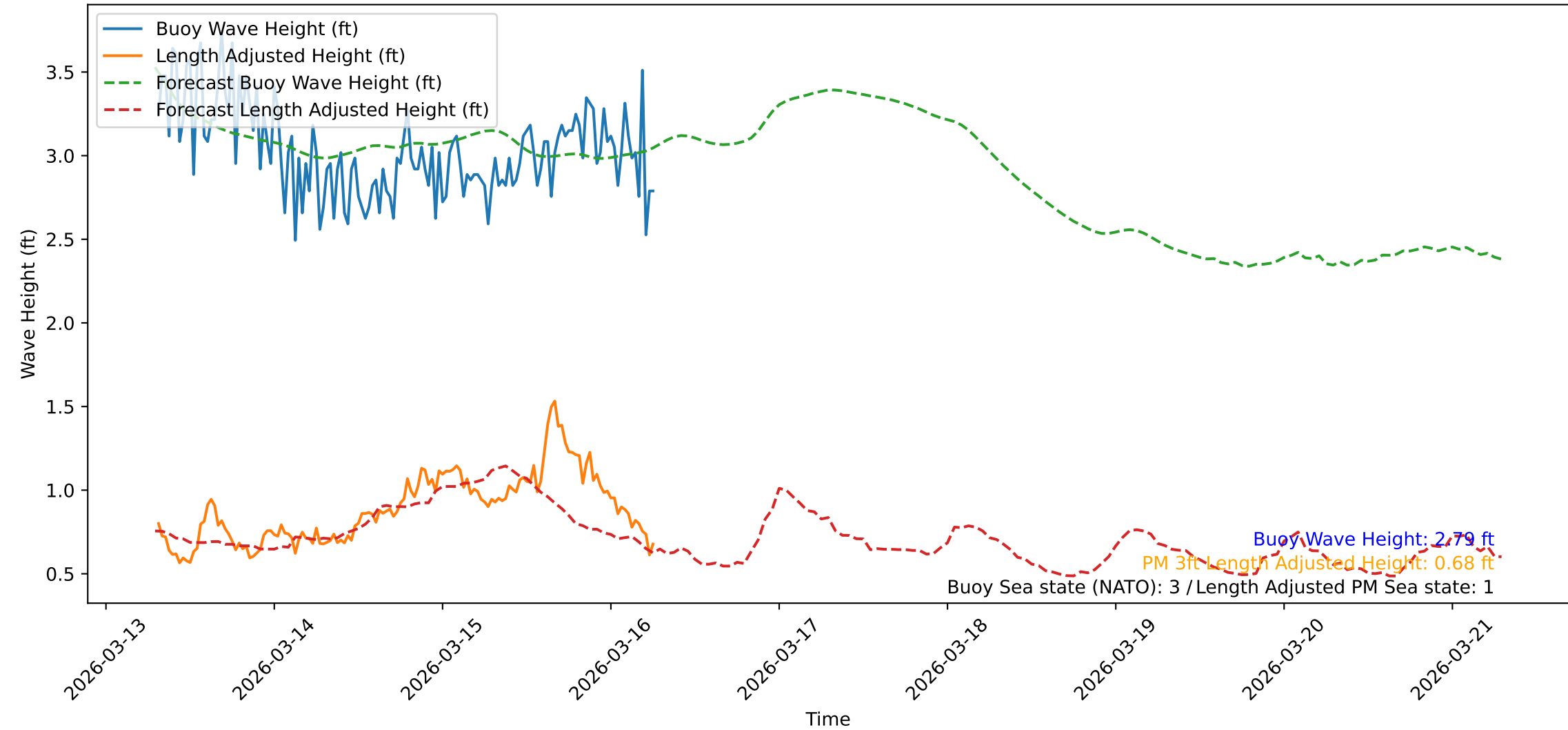
Wave Heights over Time for Red Beach at 2026-03-16 07:21:02
