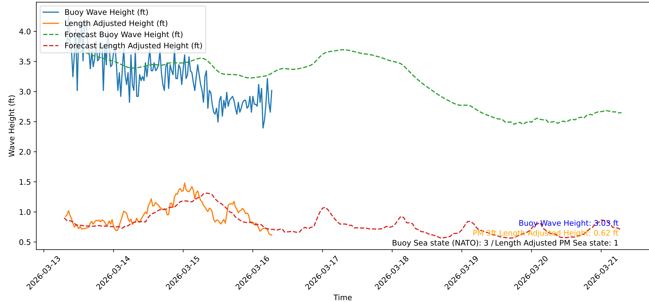
Wave Heights over Time for Oceanside Harbor at 2026-03-16 07:20:41
