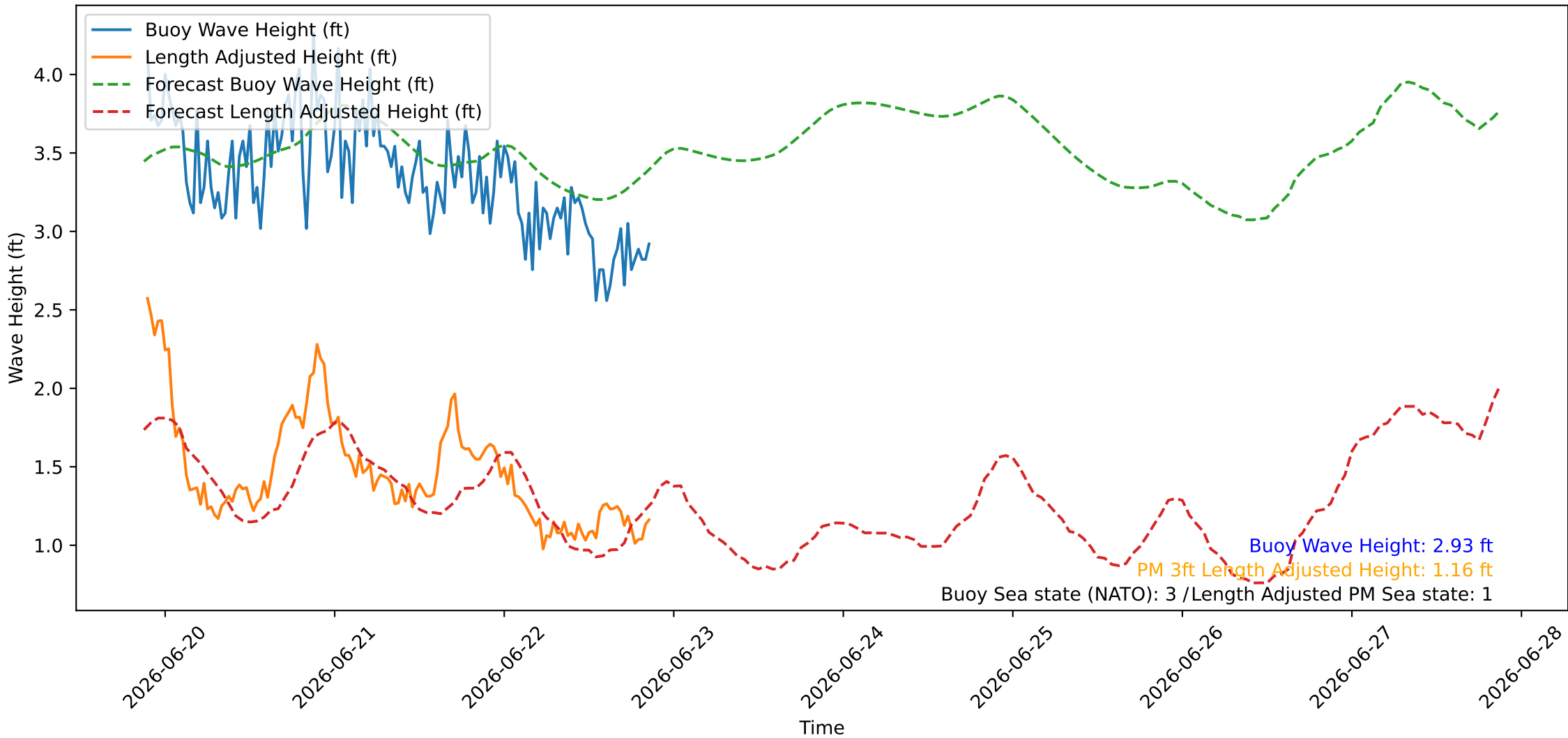
Wave Heights over Time for Oceanside Harbor at 2026-06-22 21:20:26
