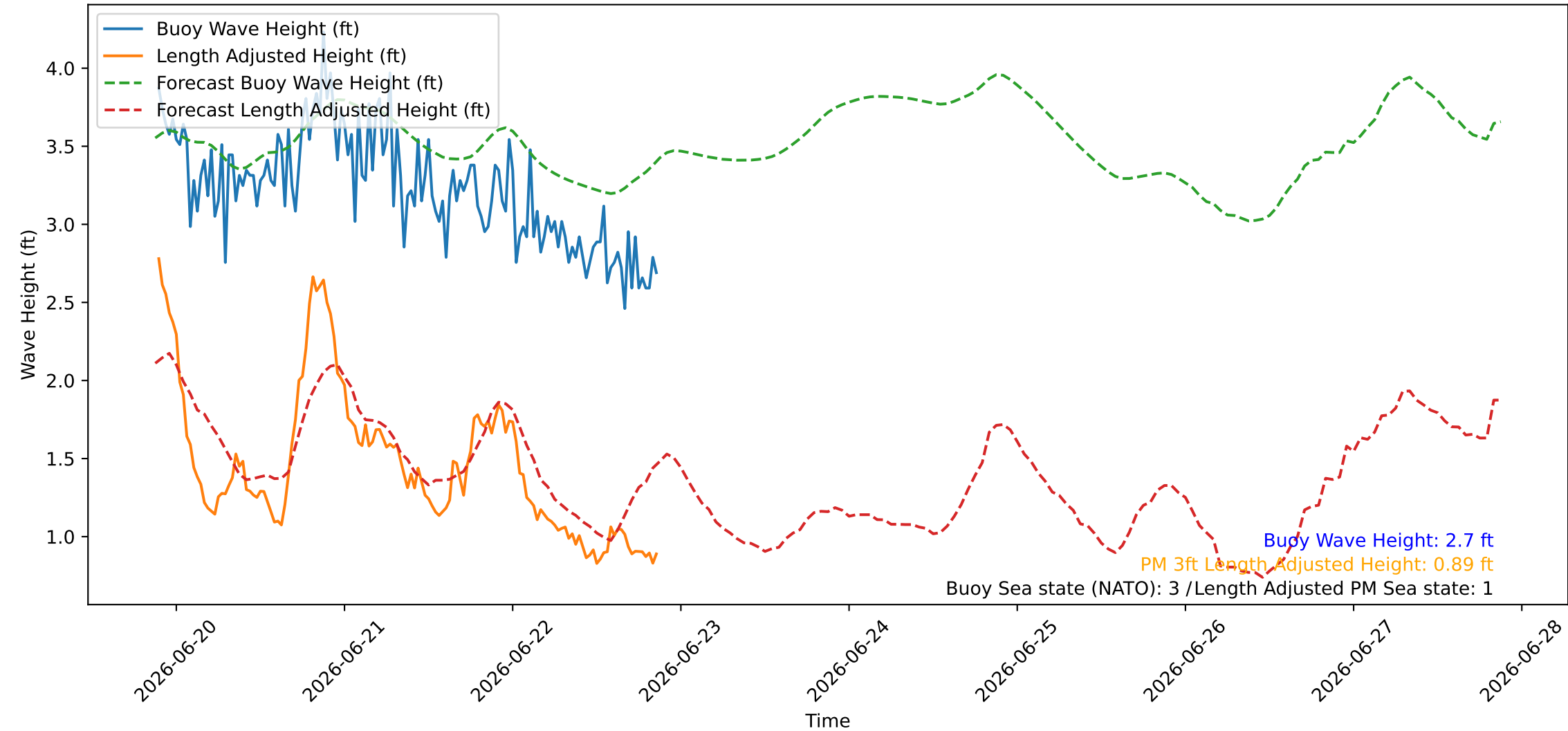
Wave Heights over Time for Green Beach at 2026-06-22 21:21:10
