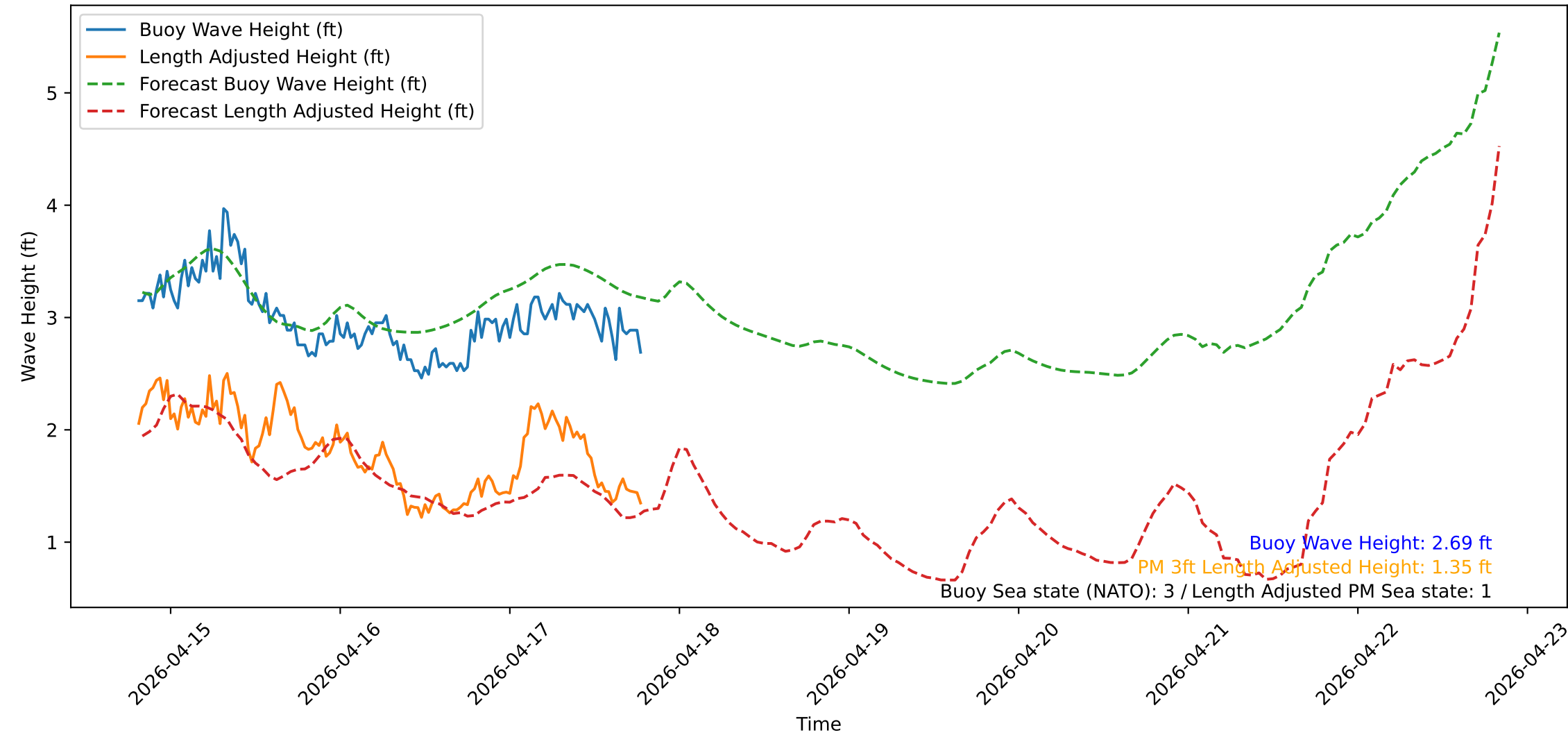
Wave Heights over Time for Green Beach at 2026-04-17 19:31:13
