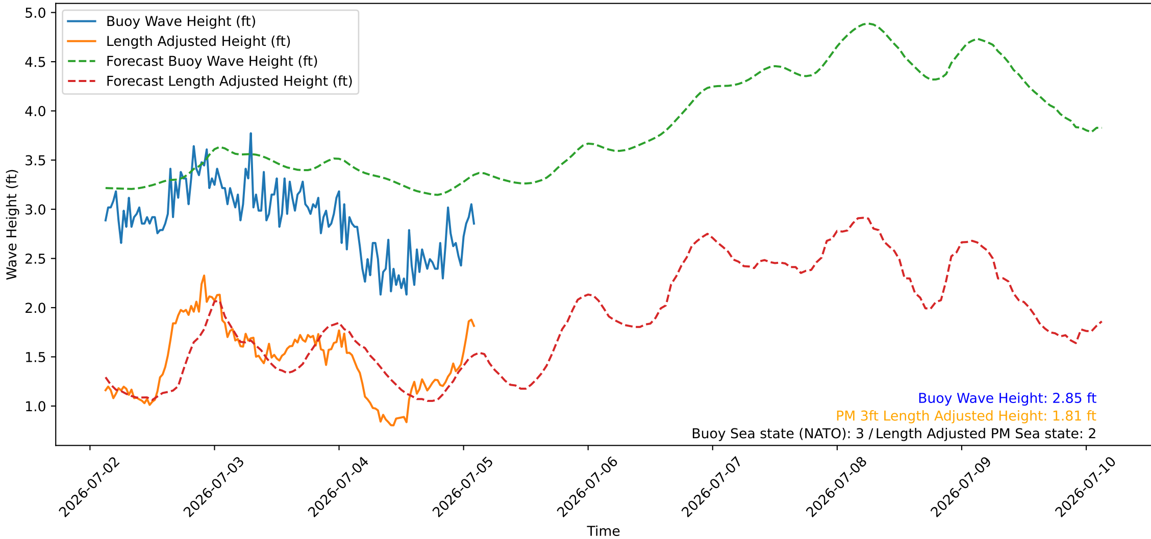
Wave Heights over Time for Oceanside Harbor at 2026-07-05 03:00:26
