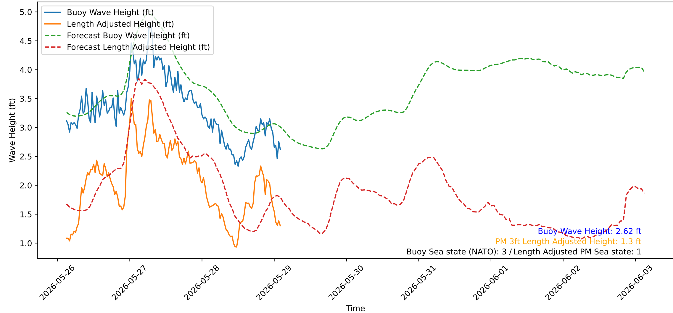
Wave Heights over Time for Red Beach at 2026-05-29 02:40:39
