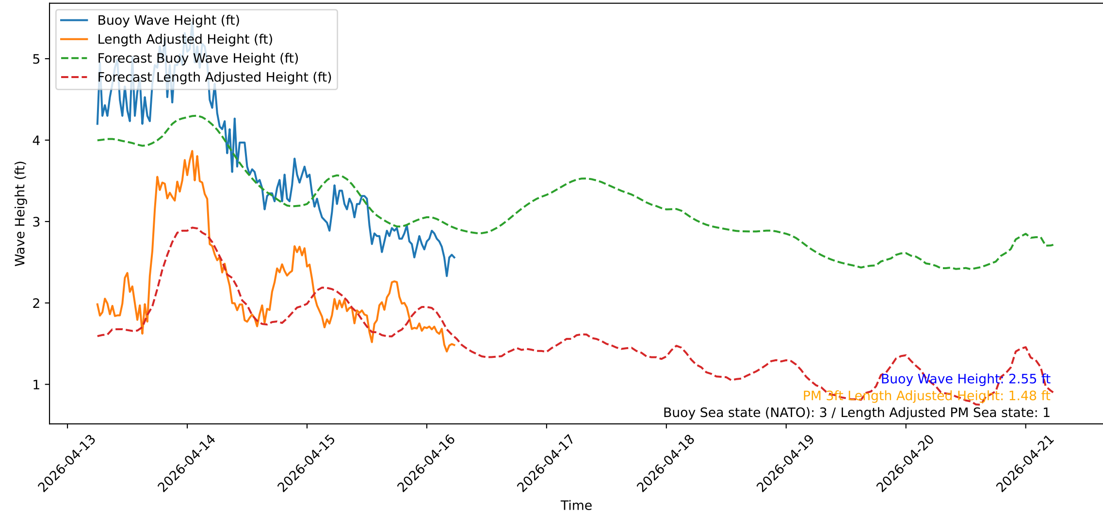
Wave Heights over Time for Oceanside Harbor at 2026-04-16 06:10:31
