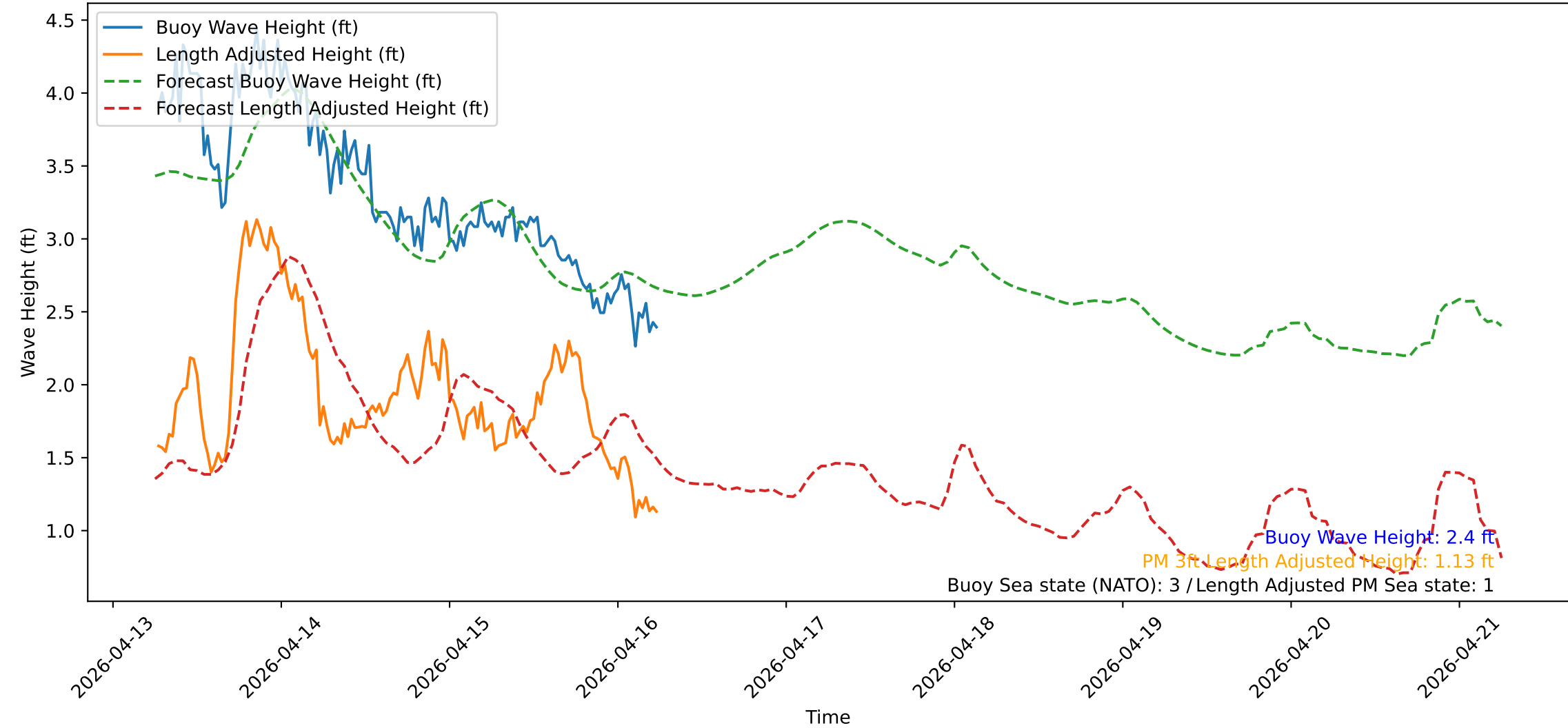
Wave Heights over Time for Red Beach at 2026-04-16 06:10:51
