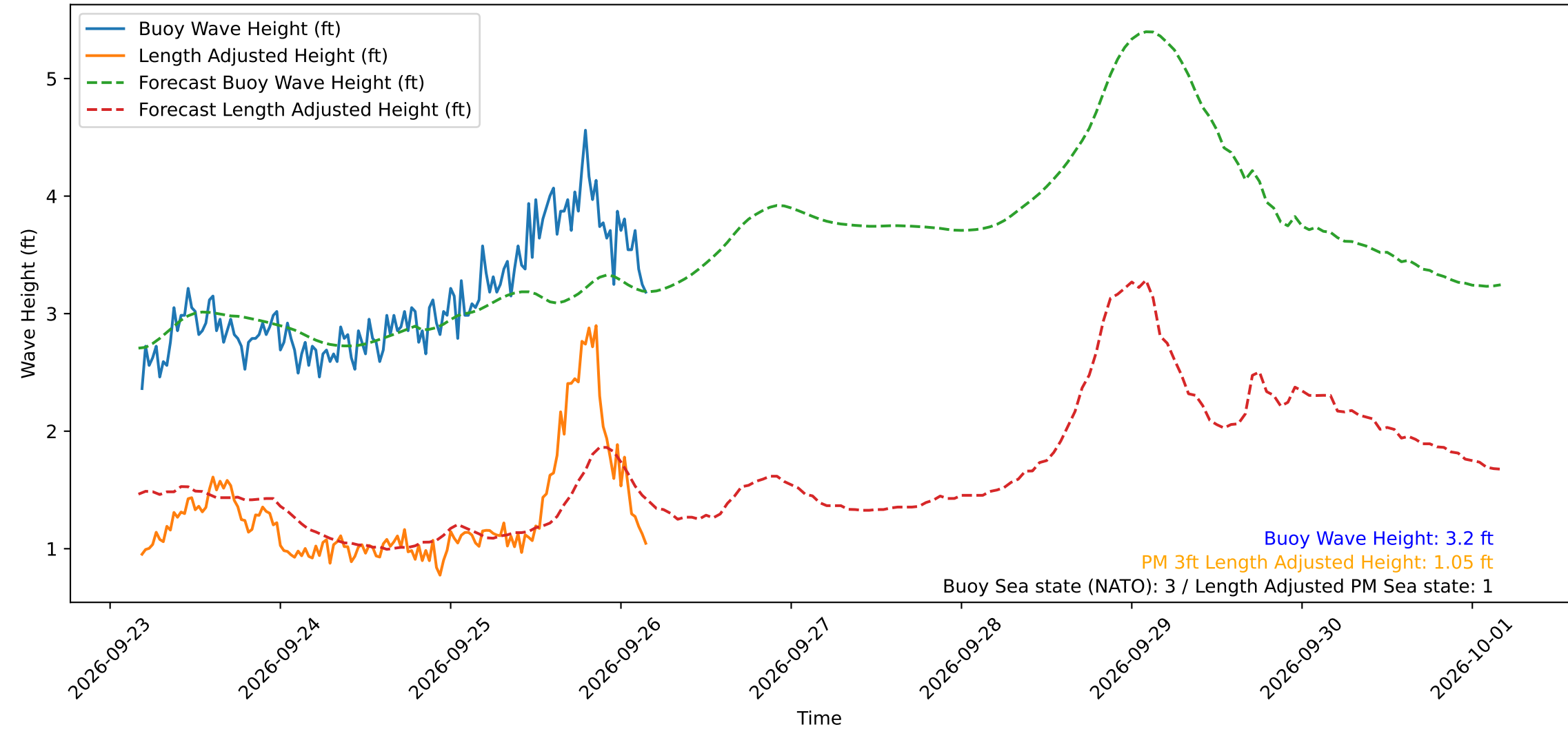
Wave Heights over Time for Green Beach at 2026-09-26 04:11:11
