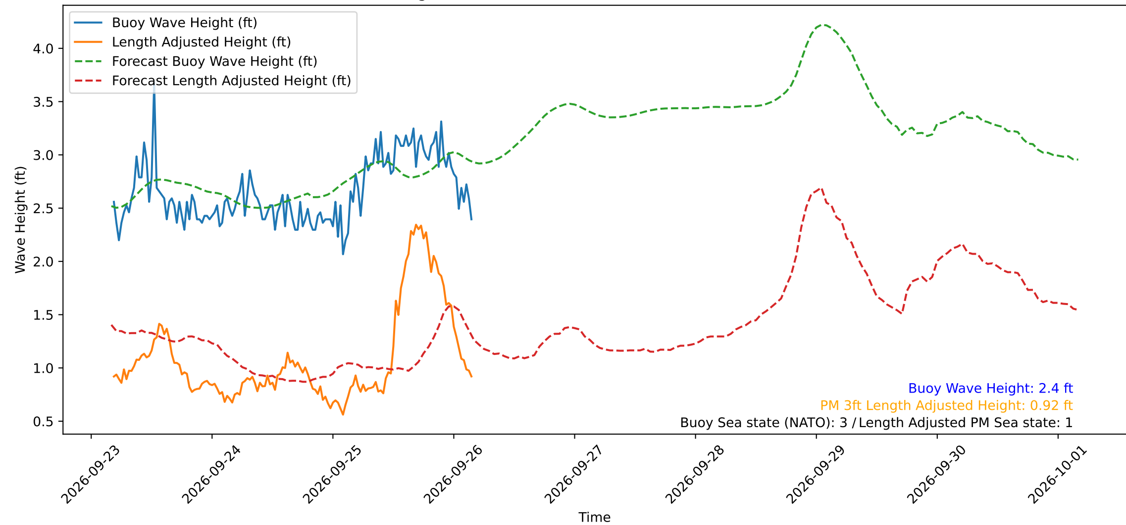
Wave Heights over Time for Red Beach at 2026-09-26 04:10:49
