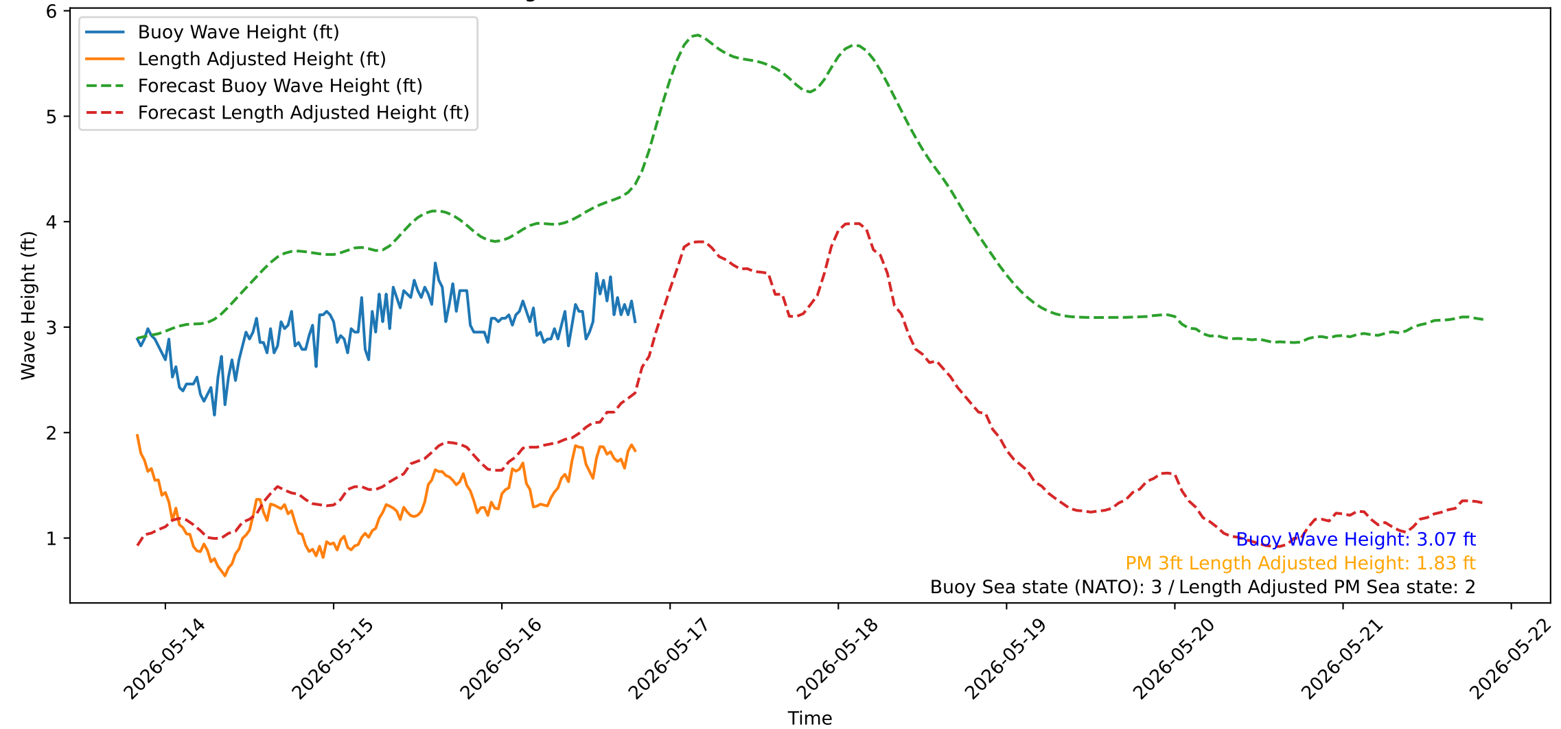
Wave Heights over Time for Oceanside Harbor at 2026-05-16 19:50:31
