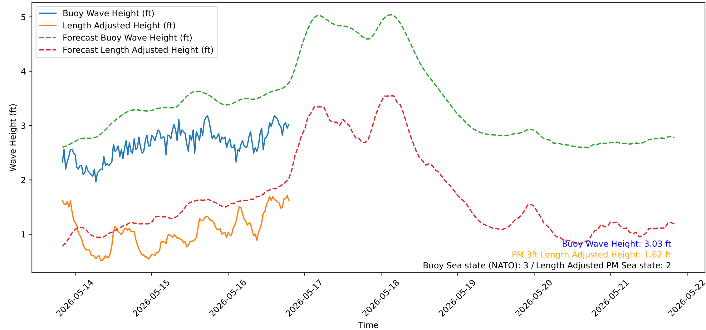
Wave Heights over Time for Red Beach at 2026-05-16 19:50:51
