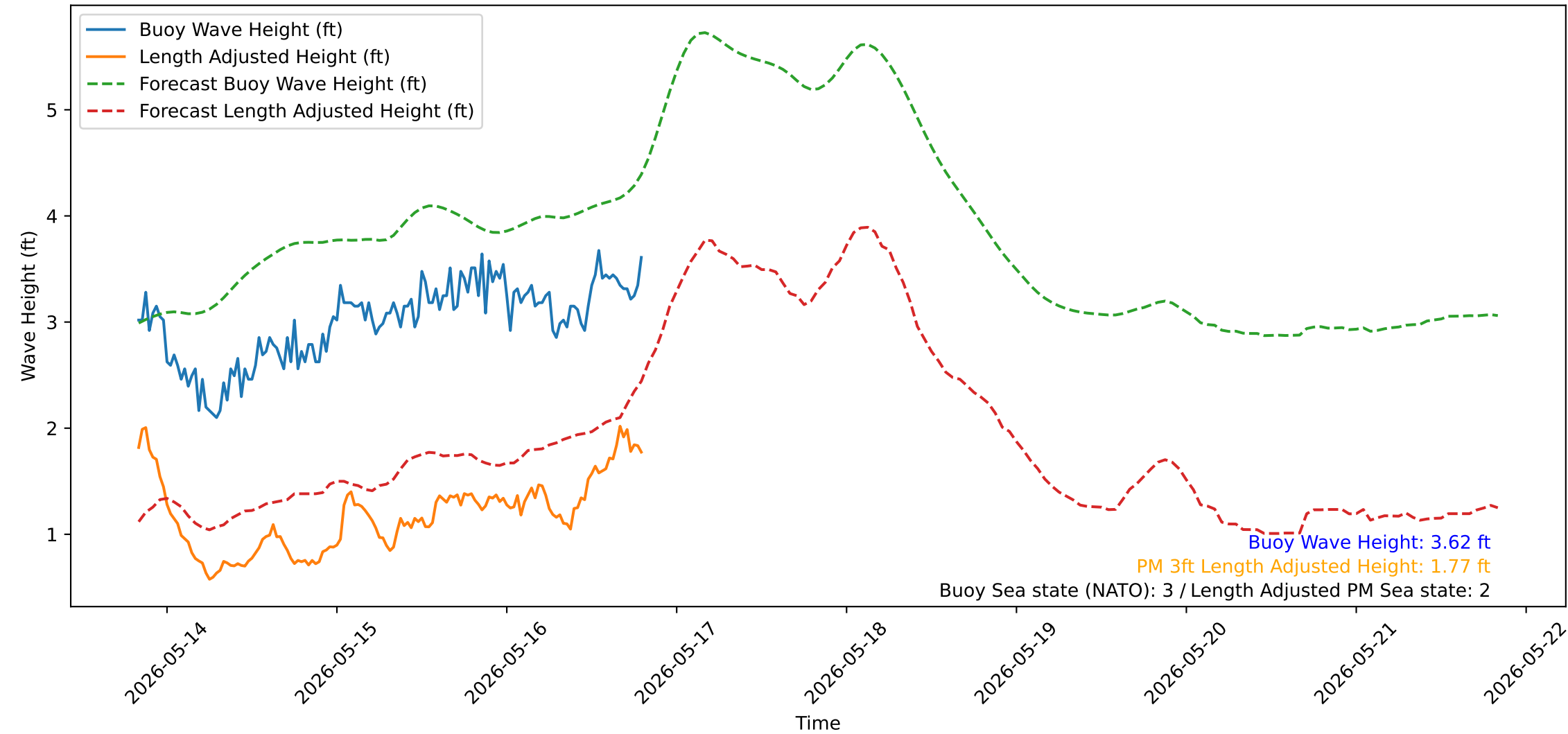
Wave Heights over Time for Green Beach at 2026-05-16 19:51:14
