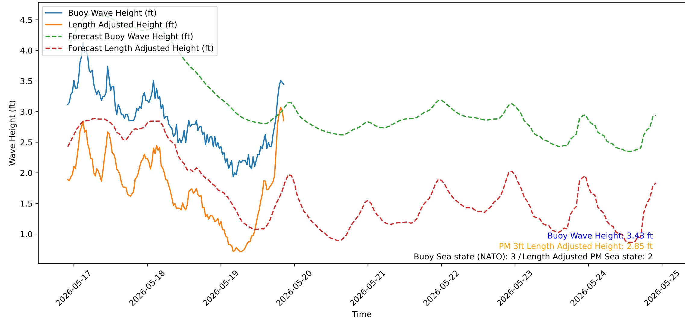
Wave Heights over Time for Red Beach at 2026-05-19 21:30:52
