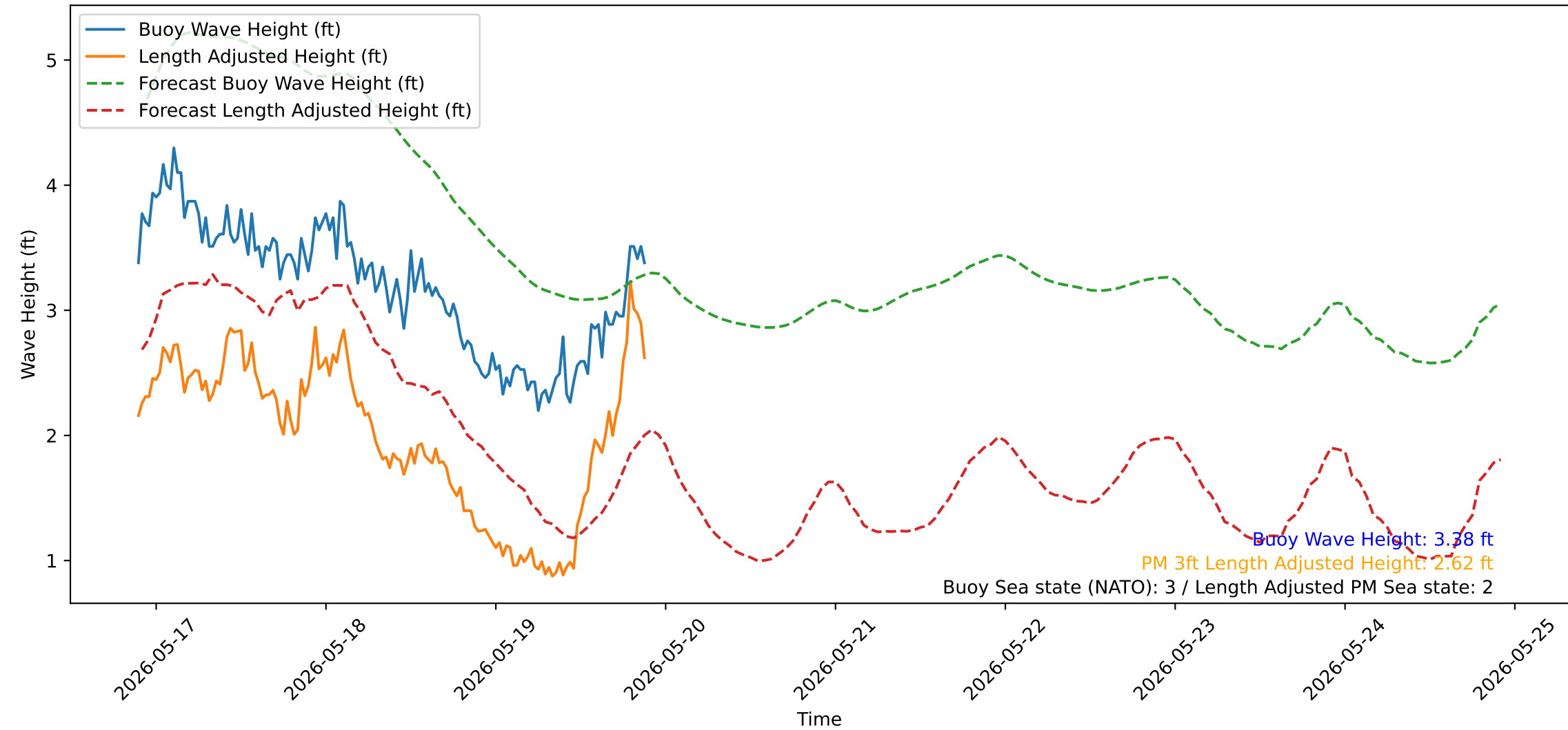
Wave Heights over Time for Oceanside Harbor at 2026-05-19 21:30:32
