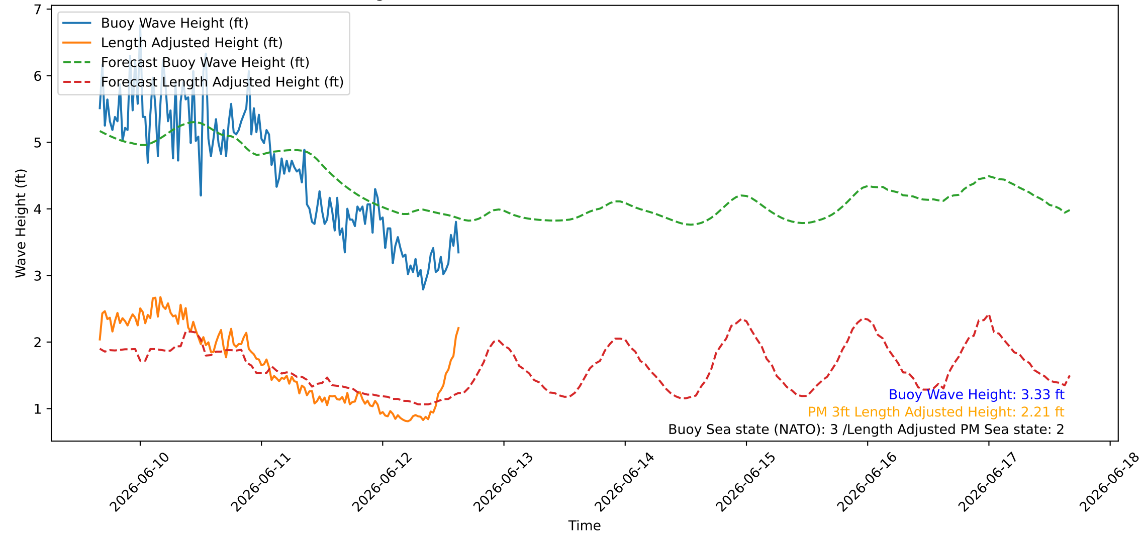
Wave Heights over Time for Oceanside Harbor at 2026-06-12 15:50:26
