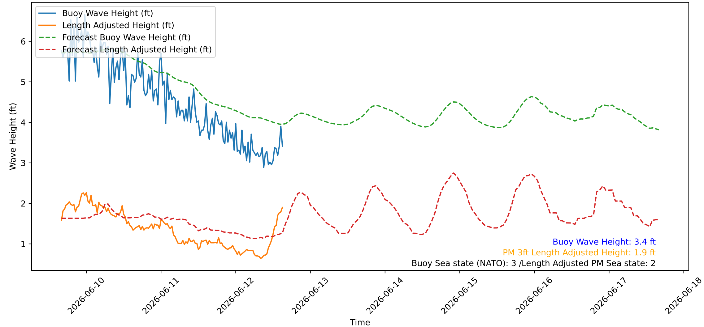
Wave Heights over Time for Green Beach at 2026-06-12 15:51:10
