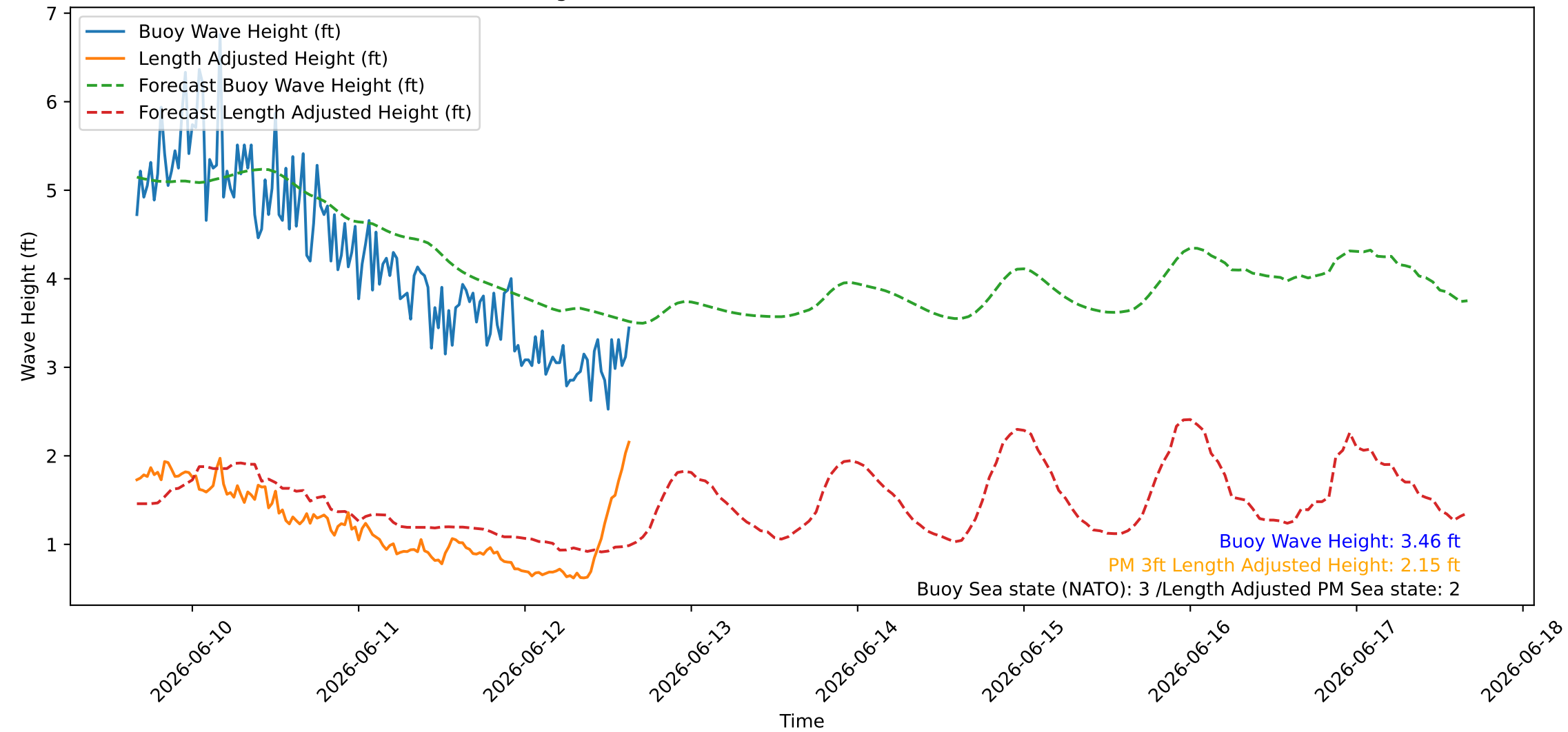
Wave Heights over Time for Red Beach at 2026-06-12 15:50:47
