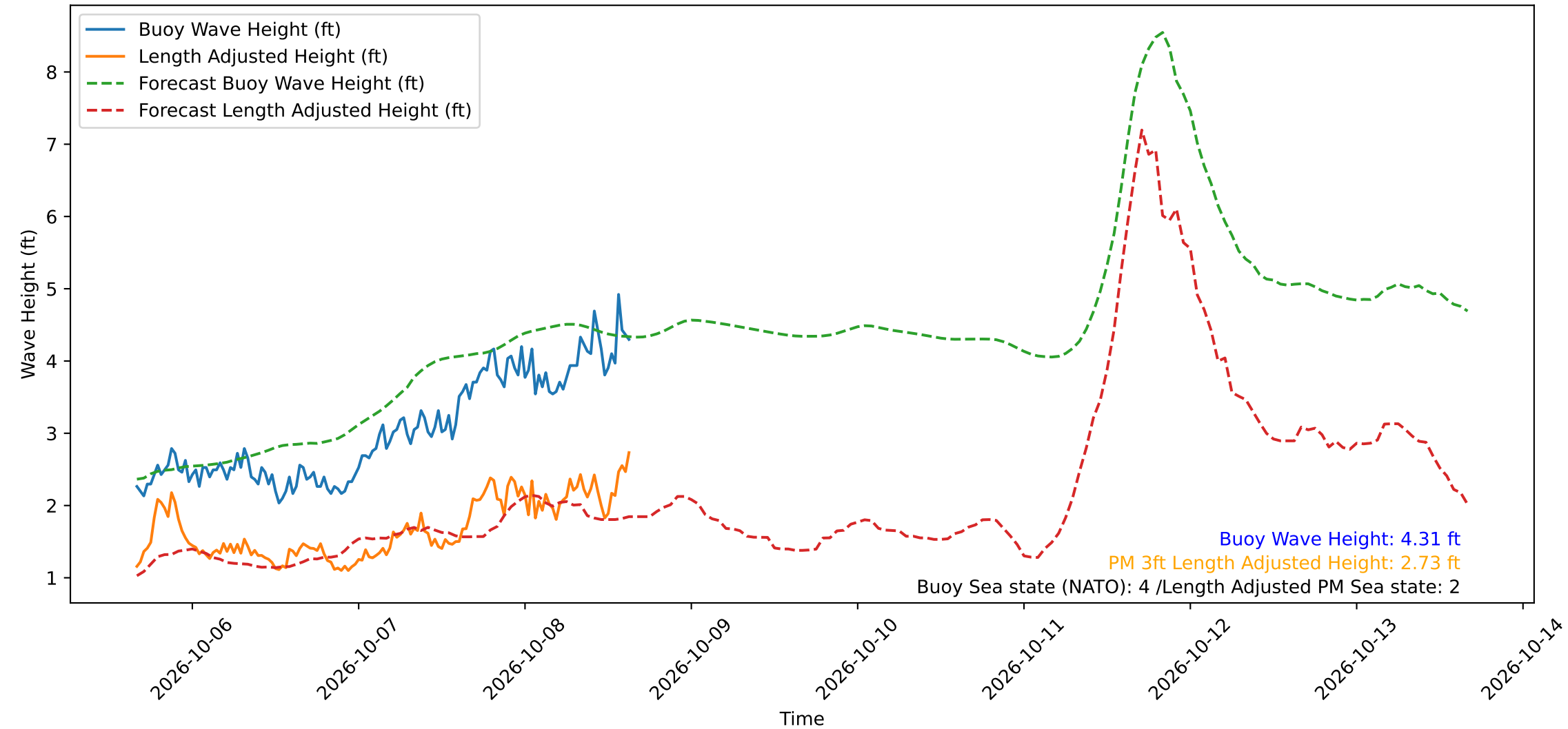
Wave Heights over Time for Oceanside Harbor at 2026-10-08 16:00:30
