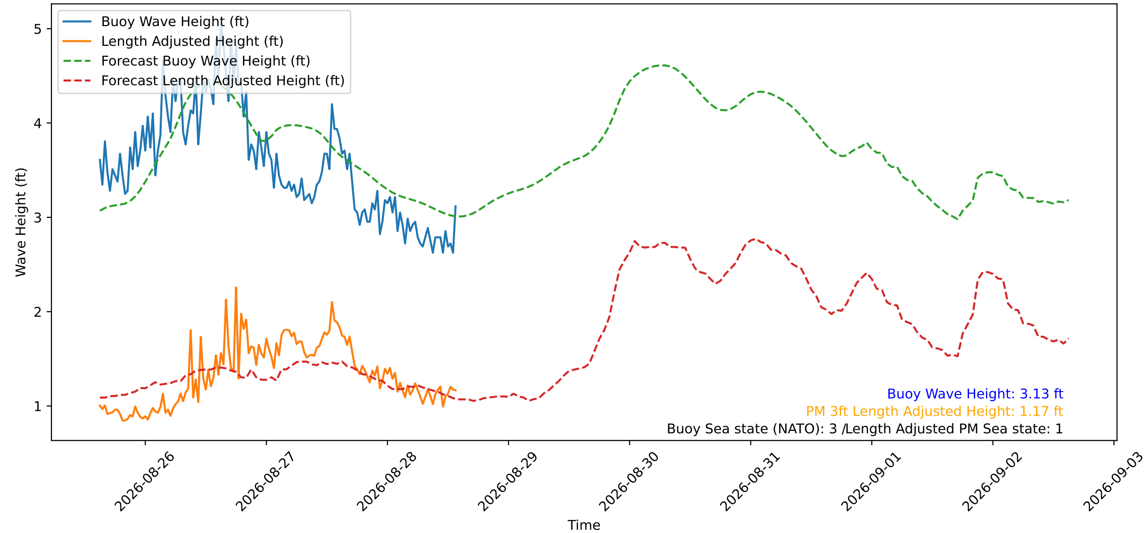
Wave Heights over Time for Red Beach at 2026-08-28 14:30:49
