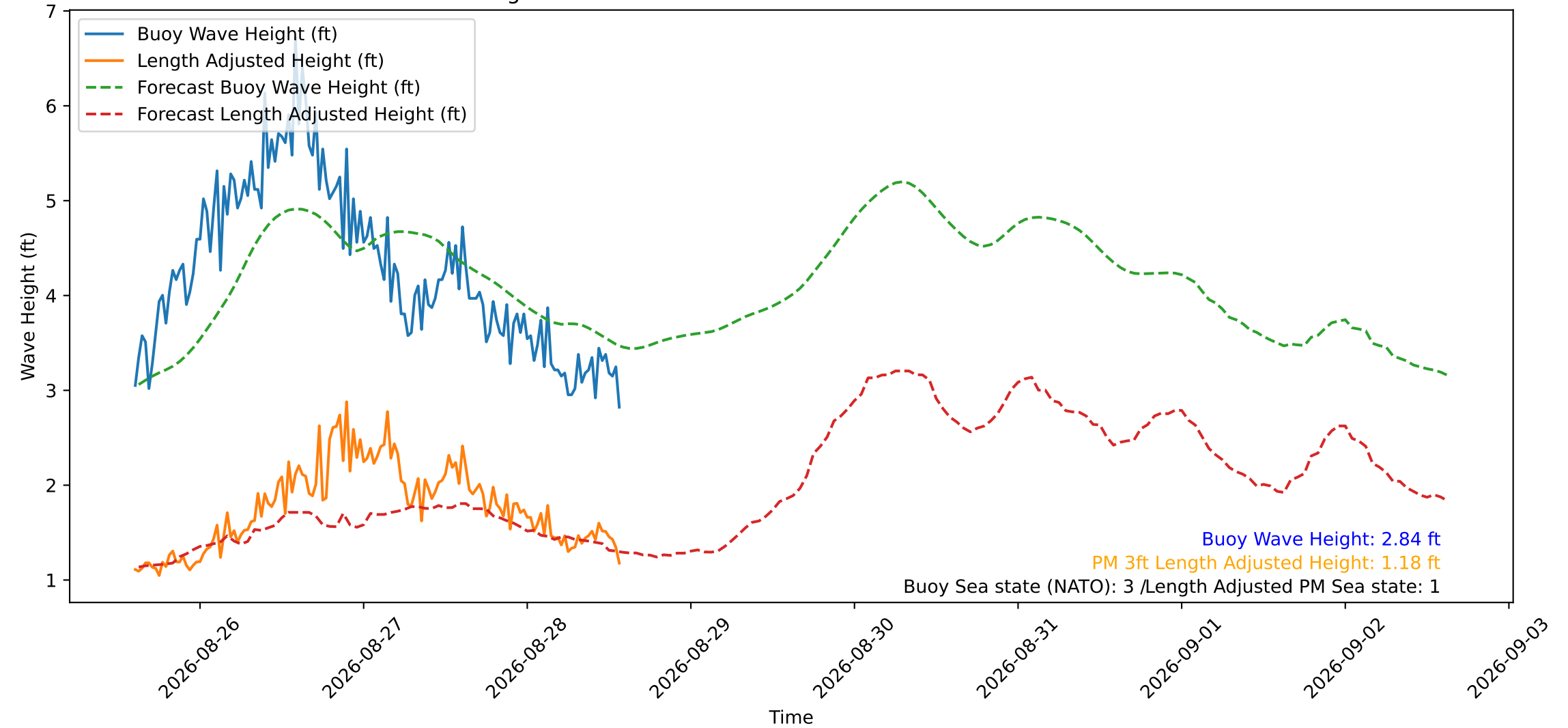
Wave Heights over Time for Oceanside Harbor at 2026-08-28 14:30:29
