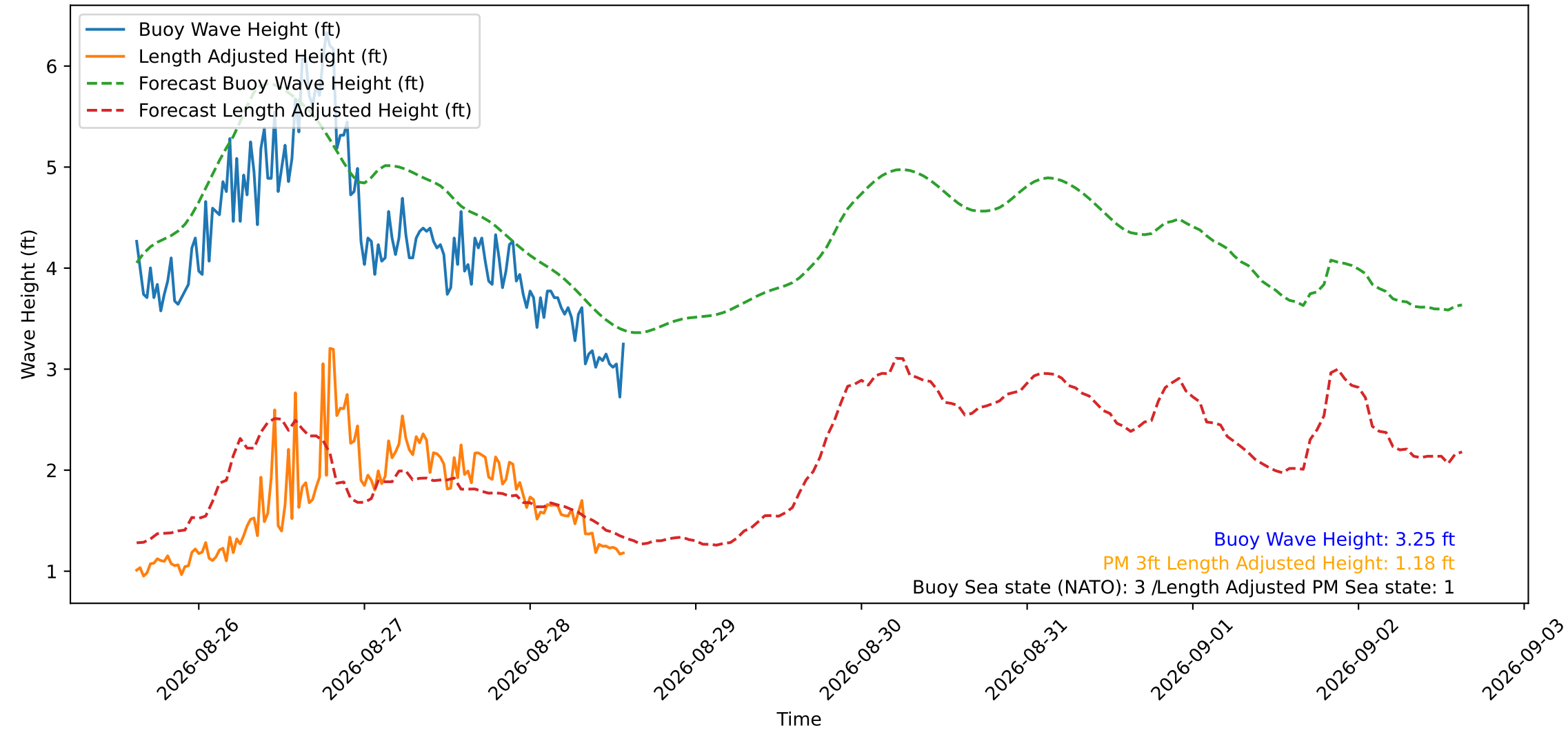
Wave Heights over Time for Green Beach at 2026-08-28 14:31:11
