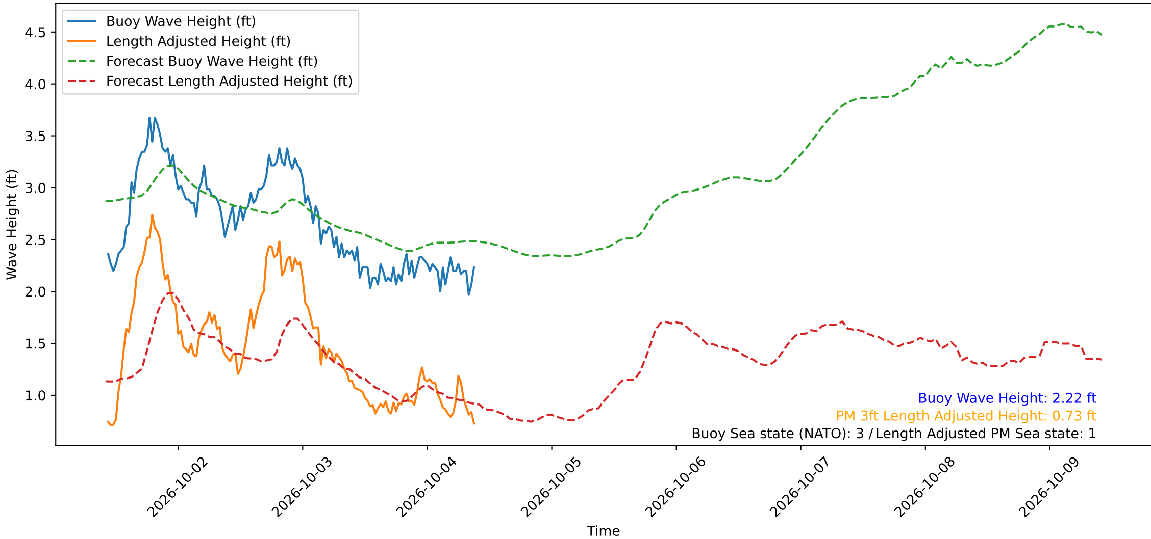
Wave Heights over Time for Green Beach at 2026-10-04 10:01:11
