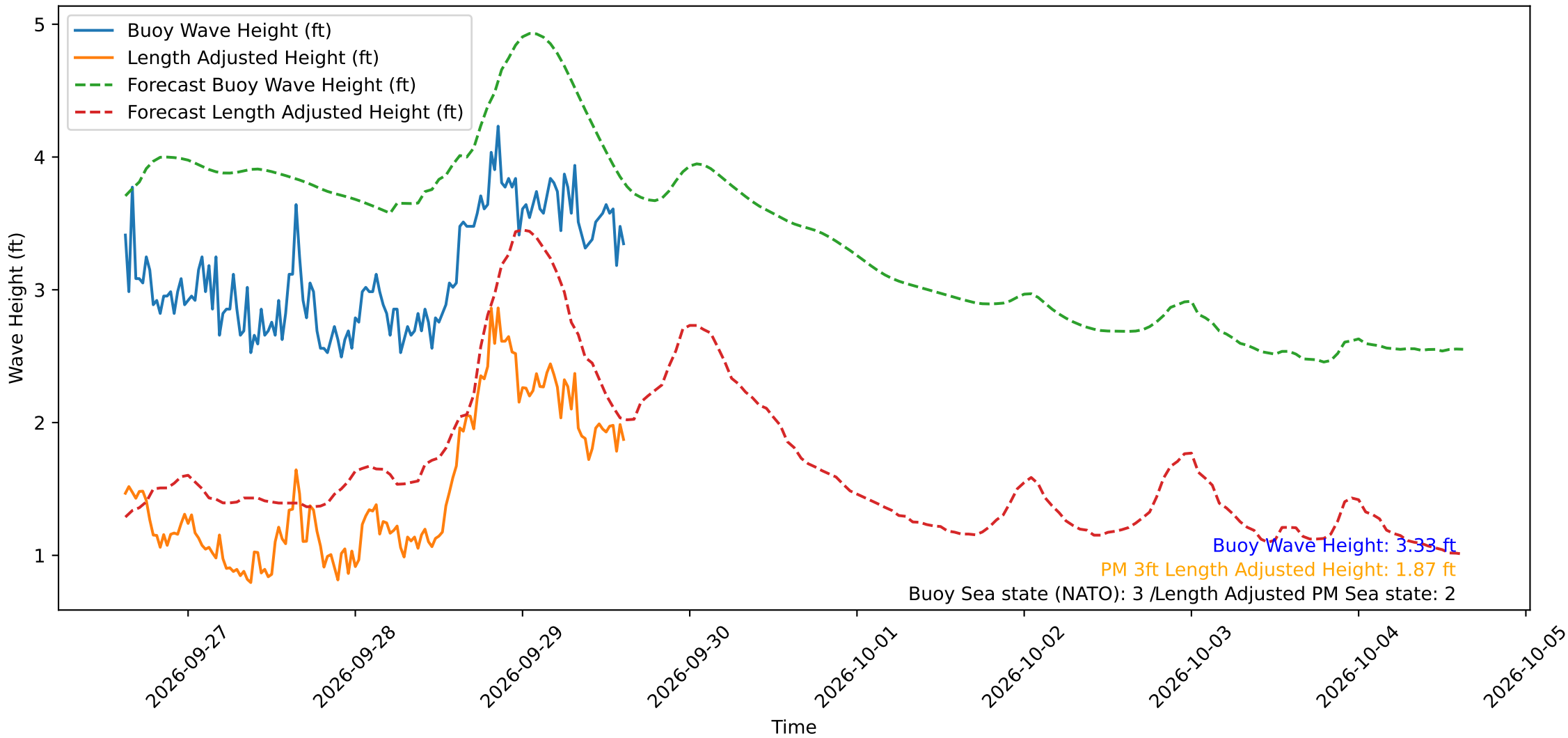
Wave Heights over Time for Oceanside Harbor at 2026-09-29 15:10:29
