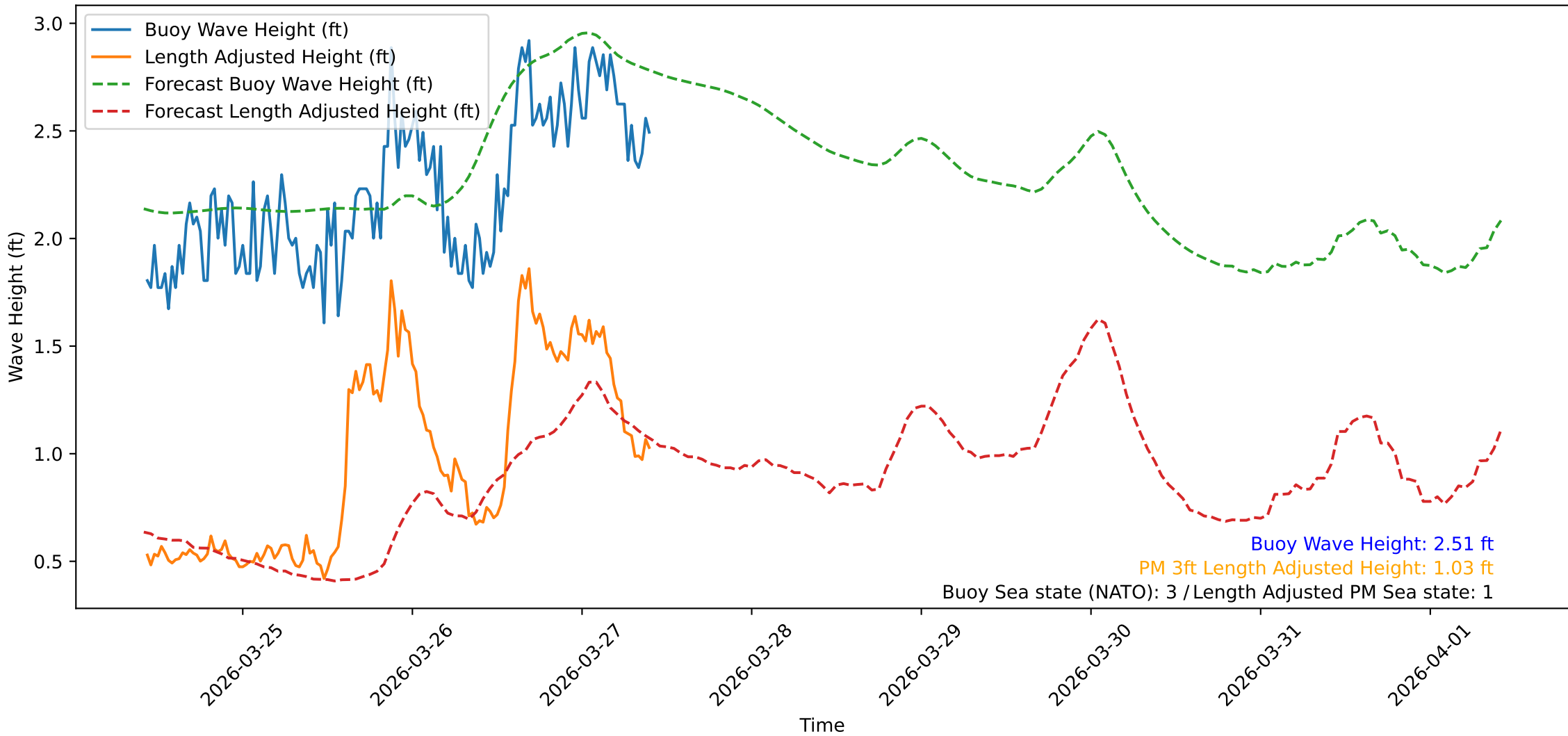
Wave Heights over Time for Oceanside Harbor at 2026-03-27 10:20:31
