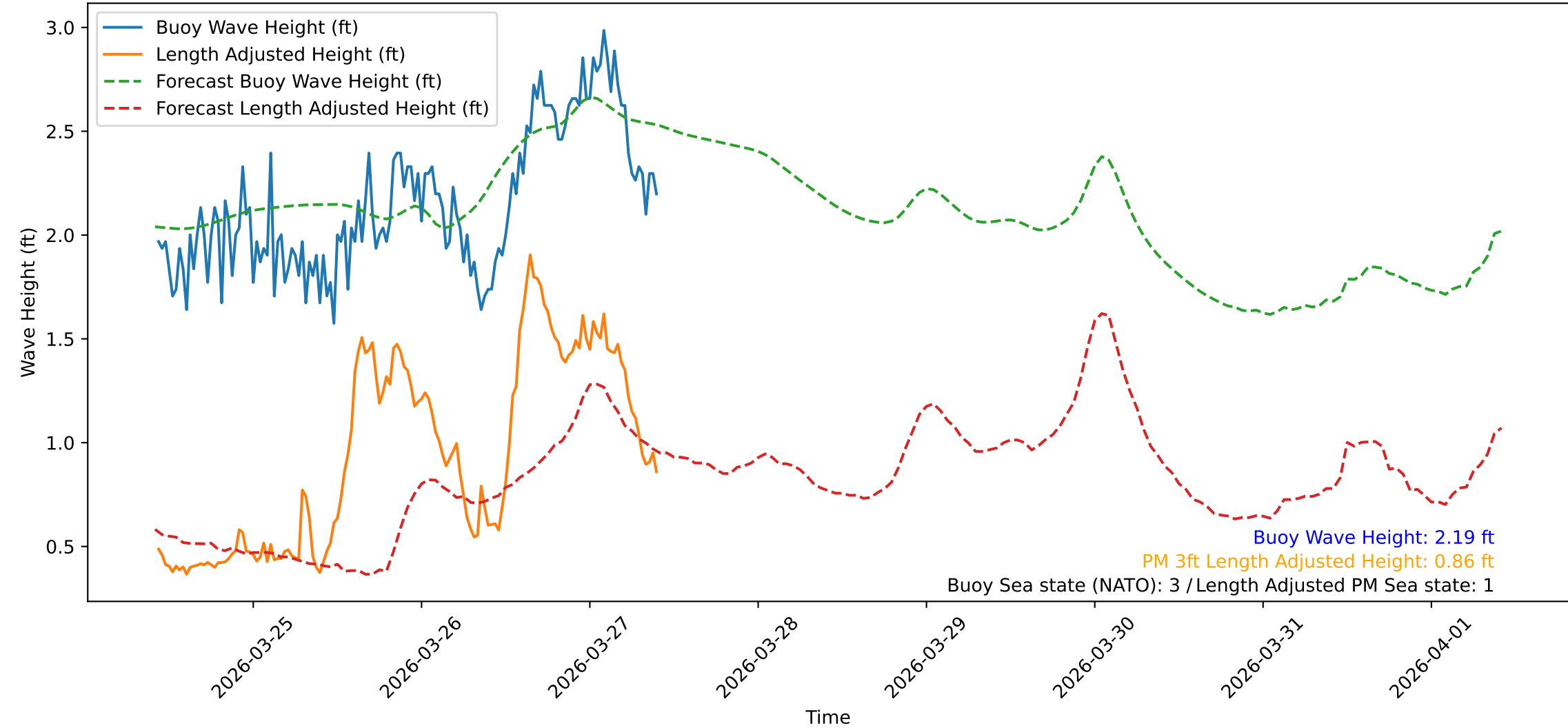
Wave Heights over Time for Red Beach at 2026-03-27 10:20:47
