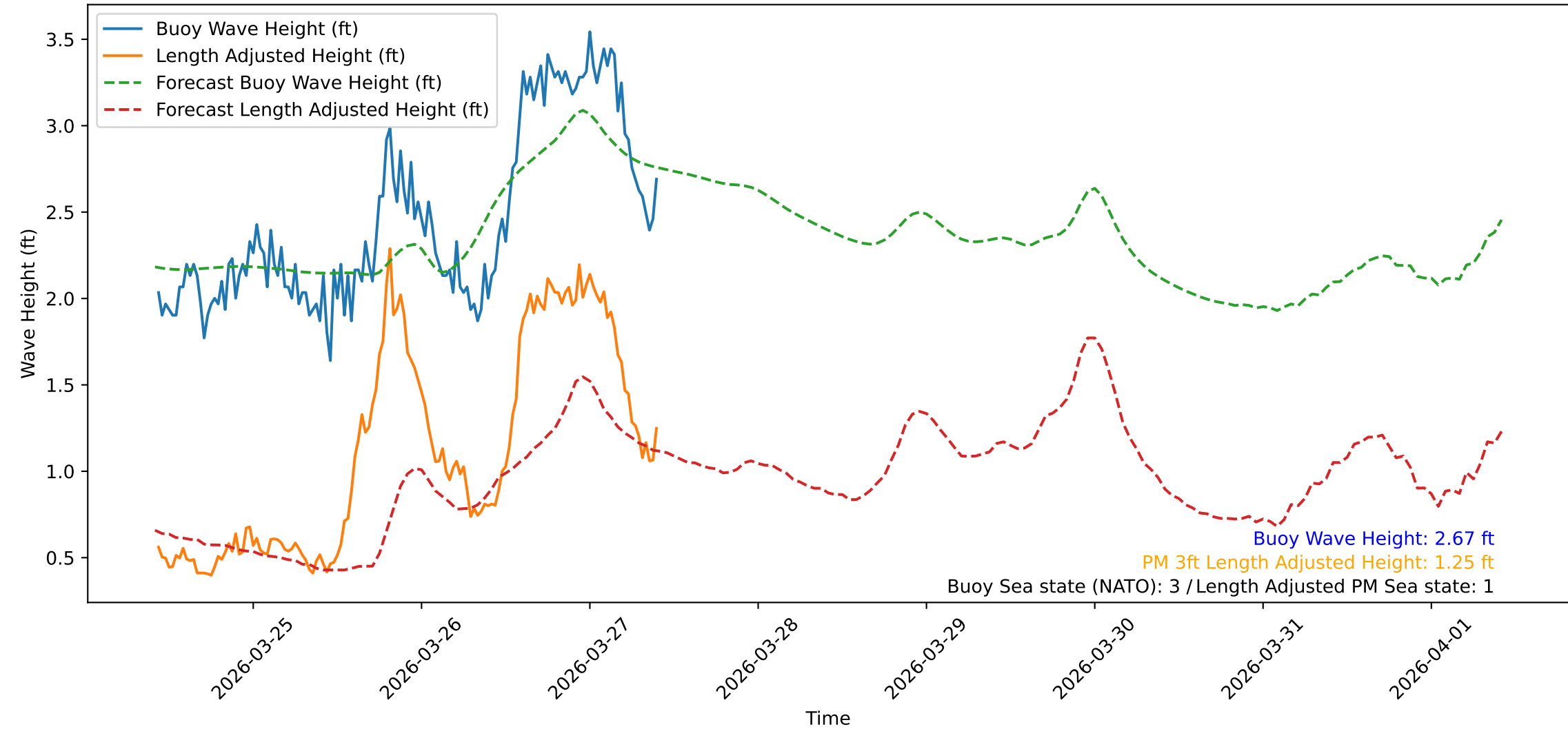
Wave Heights over Time for Green Beach at 2026-03-27 10:21:11
